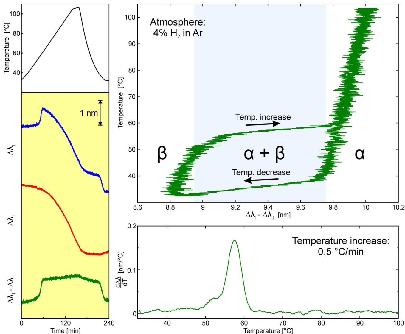
Figure 4. Drift correction during a temperature ramp from 30 °C to above 100 °C in 4% H 2 in Ar. The top left graph shows the temperature ramp and the graph below shows the corresponding LSPR peak shifts measured in parallel (blue) and perpendicular (red) polarizations, as well as the difference (green) between the two. Notably, both the blue and red curves show significant irreversible peak shift (the reasons are discussed in the main text), whereas the difference signal is perfectly reversible and shows the following features: at the lower temperatures the Pd element is in the hydride phase ( \beta -phase) until a critical temperature is reached where the hydride is decomposed into the \alpha -phase (redshift). Upon cooling the opposite occurs, that is, below a critical temperature the hydride is formed again (blueshift). In the top right graph the difference signal is plotted versus the temperature of the sample, which yields a fully reversible isobar of the hydride decomposition and formation process in the Pd nanoparticle (note also the hysteresis between the decomposition and formation). The bottom right graph shows the numerical derivative of the isobar during the temperature increase (calculated using moving a linear fit with dT = 5 °C), yielding a signal similar to a temperature programmed desorption (TPD) measurement with a peak at the hydride decomposition temperature.
