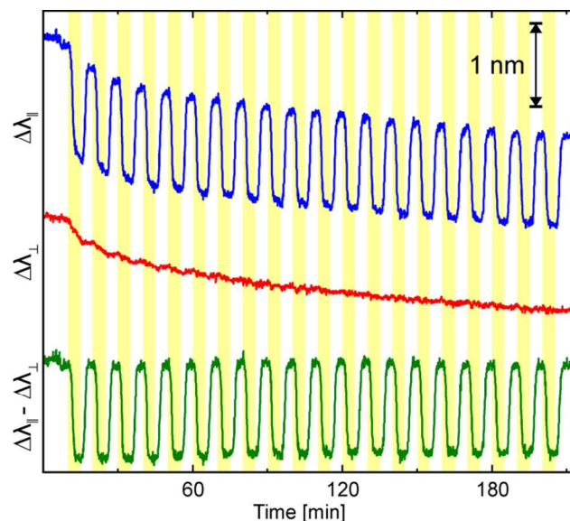
Figure 3. Sensor response upon cyclic exposure to pure Ar (white shaded areas) and 4 % H 2 in Ar (yellow shaded areas) at 30 °C. The blue line shows the LSPR peak response of the sensor upon excitation in the parallel polarization configuration, and the red line in the perpendicular polarization. The green line shows the difference between the two polarization signals and does not exhibit any drift or irreversibility over the 3.5 h duration of the experiment.
