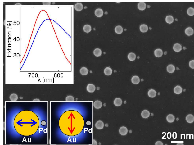
Figure 1. Sketch of the drift-corrected nanoplasmonic hydrogen sensing principle with an SEM image of the used AuPd heterodimer structures in the background. The sensor consists of a quasi-random array of heterodimers featuring a large, inert disk-shaped Au sensor element (diameter 140 nm), and a small hydrogen-sensitive Pd particle (diameter 40 nm) fabricated next to it. The size-mismatch is chosen such that the LSPRs in the Au and Pd elements are significantly spectrally detuned. By the use of a polarizing beamsplitter the extinction spectra of polarizations parallel and perpendicular to the dimer axis are monitored simultaneously. The inset shows extinction spectra for the two polarizations, parallel (blue) and perpendicular (red). In the case of parallel polarization the Au disk plasmon couples to the Pd particle through its near field. For the perpendicular polarization the coupling is basically absent.
