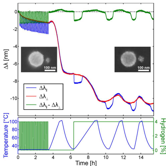
Figure 2. The top graph shows the LSPR-peak response of the sensor for light polarization parallel to the dimer axis (blue), polarization perpendicular to the dimer axis (red), and the difference between the two (green). Note the almost perfect correction for long-term irreversible peak shifts in the drift-corrected (green) signal. The reshaping of the Pd particle induced by repeated hydride formation and decomposition, as seen in the two inset SEM images of the structures before (left) and after (right) the measurement, is the reason for the slight long-term signal drift that still is seen. Further cycling in hydrogen can be applied to completely eliminate this effect. The lower graph shows the temperatures (blue line) and hydrogen concentrations (green line) the sample was subjected to during the entire measurement sequence.
