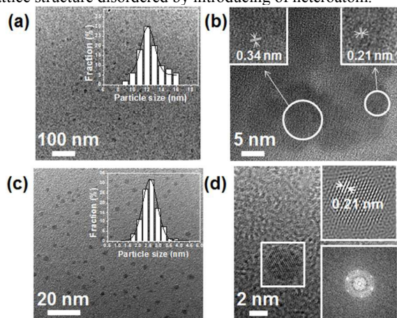
Figure 7. (a) TEM image of GQD (a) TEM image of G-QQDs. Inset: size distribution with Gaussian fitting curve. The average size is 12.1 \pm 3.5 nm. (b) HRTEM image of G-QQDs, showing lattice fringes of 0.34 nm and 0.21 nm. (c) TEM image of GQDs derived from ATP. Inset: Size distribution with Gaussian fitting curve. The average size is 2.8 \pm 1.0 nm. (d) HRTEM image of GQDs derived from ATP. Insets: (top) FFT-filtered HRTEM image, (bottom) the corresponding FFT of the HRTEM image highlighted in the white square in (d).
