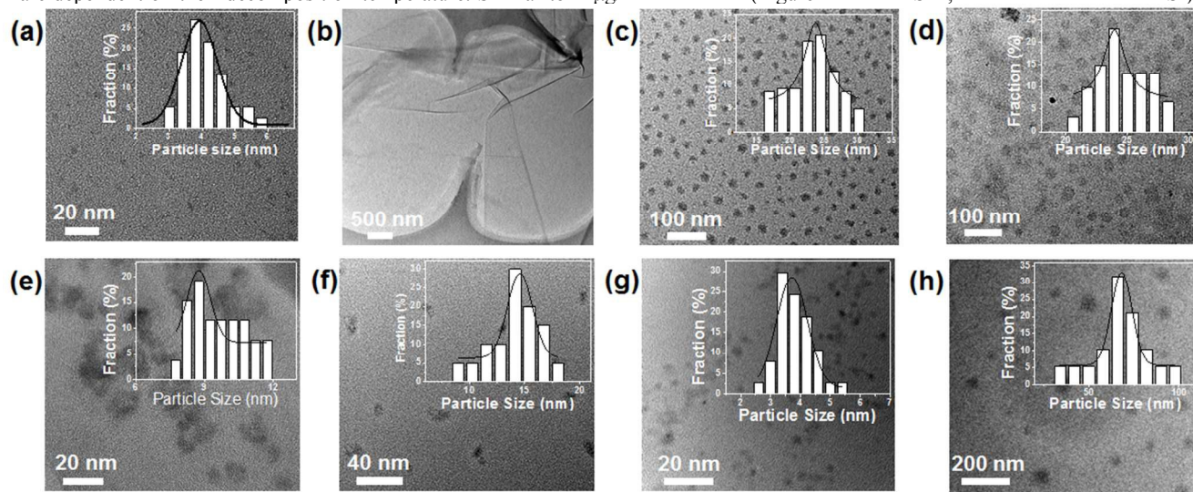
Figure 6. (a) TEM image of GQDs derived from (a) arginine. Inset: size distribution with Gaussian fitting curve. The average size is 4.5 \pm 1.5 \text{ nm} . (b) TEM image of large flakes obtained with arginine as precursor at longer reaction time. TEM image of GQDs derived from (c) lysine ( 23.5 \pm 6.6 \text{ nm} ), (d) tartaric acid ( 24.5 \pm 3.8 \text{ nm} ), (e) sucrose ( 9.8 \pm 2.0 \text{ nm} ), (f) cysteine ( 13.5 \pm 4.6 \text{ nm} ), (g) cystine ( 3.8 \pm 1.6 \text{ nm} ) and (h) DTT ( 66 \pm 32 \text{ nm} ). Insets show the size distributions.
