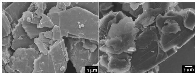
Fig. 4. SEM morphology of the as-received graphite material used as the cathode during the electrolysis process.
