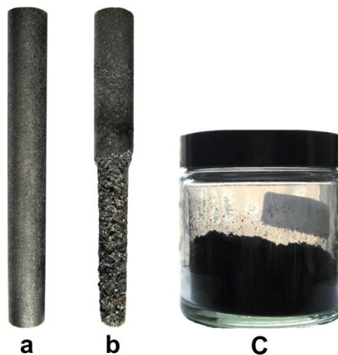
Fig. 2. The photographs of (a) the graphite rod which was used as cathode in the molten salt process conducted under moist gas flow, (b) the graphite cathode after the molten salt process, and (c) the graphene product stored in a jar.
