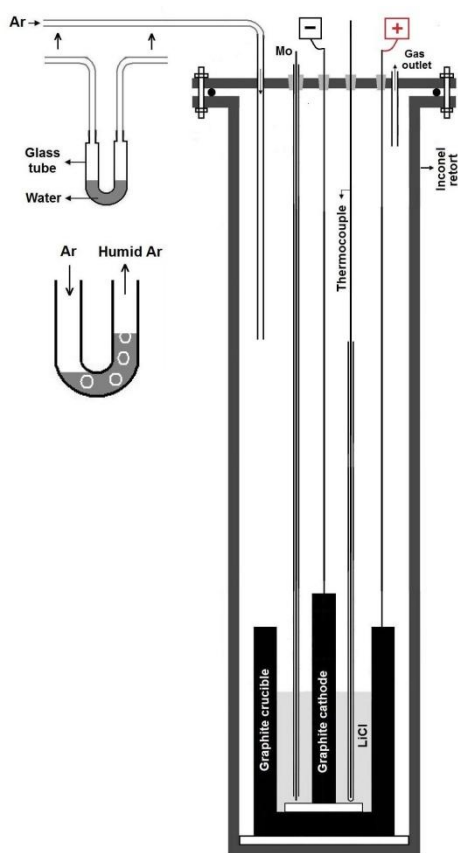
Fig. 1. A schematic presentation of the reactor used for the molten salt process. The apparatus comprised of a vertical tubular Inconel reactor, which is positioned inside a resistance furnace. The upper end of the reactor is closed with a stainless steel lid sealed with an O-ring and compression fittings. The lid is equipped with feedthroughs for electrodes leads and the thermocouple as well as with steel pipes for gas inlet and outlet. The gas inlet was coupled to a gas canister containing argon. The argon could bubble through the water within a U-bend tube before entering the reactor at the gas inlet. The U-bend tube is shown more clearly in the inset of the figure. On passing through the U-bend tube, the dry argon picked up water vapour and becomes moist argon. Thus, the atmosphere within the reactor above the molten lithium chloride was moist argon that enters through the gas inlet and exits through the gas outlet.
