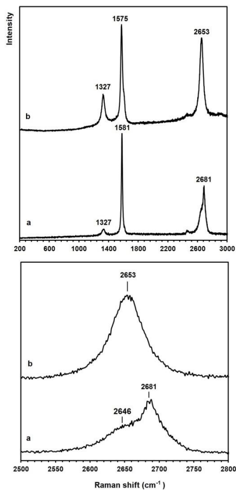
Fig. 7. Raman spectra of (a) natural graphite flakes and (b) graphene nanosheets which were produced in molten LiCl, and then heated to 1300°C in the range of (upper panel) 200–3000 and (down panel) 2500–2800 \text{cm}^{-1} at 633 nm wavelength.
