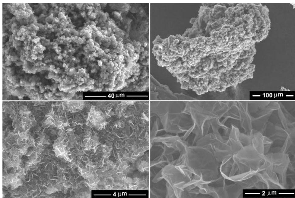
Fig. 5. Secondary electron SEM images of the graphene nanosheets, produced by heating the as-synthesised carbonaceous material to 1300°C (left panels) and 1450°C (right-upper panel) at different magnifications. The right-down panel shows a backscattered electron SEM micrograph of graphene nanosheets obtained at 1450°C. The products exhibited nanosheets morphology with a high yield.
