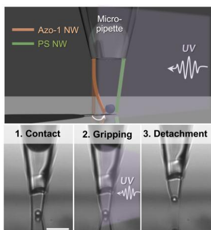
Fig. 5 Azo-1 and a PS nanowire (500 nm ( d ) x 12.5 \mu m ( l )) arms were individually integrated on the tip of a glass microcapillary tube. As demonstrated by the optical microscope images, the resulting tweezers successfully grips a PS microparticle ( d \sim 4 \mu m) on a silicon substrate upon irradiation with UV light (1.5 mW/cm 2 for 20 s): 1 (contact) \rightarrow 2 (gripping) \rightarrow 3 (detachment). Scale bar, 20 \mu m.
