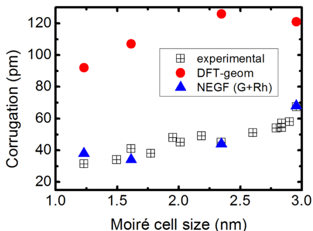
Fig. 5. Variation of the corrugation with the moirés' periodicity: both the experimental and the theoretical results have been plotted in this figure. Despite the fact that geometrical values for the corrugation are higher (red circles) than the apparent corrugation measured in the STM experiments (black squares), accurate transport simulations of constant current STM profiles using a NEGF formalism yield apparent corrugations (blue triangles, extracted from the profiles at z_0 = 5 Å in Fig. 4) in excellent agreement with the experiments.
