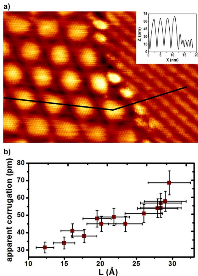
Fig. 3. Variation of the corrugation with the moirés' periodicity: (a) 19 \times 13 \text{ nm}^2 atomically resolved STM image of two different moirés; tunnelling parameters, V_s = 40 \text{ mV} , I_t = 11 \text{ nA} ; inset: profile taken from the STM image where the difference in the corrugation amplitude in both moirés can be easily observed. (b) Plot of the apparent corrugation of several moirés as a function of their periodicity parameter ( L ). The apparent corrugations have been taken from measurements performed with bias voltage in the range between -1.1 and -1.8 \text{ V} . See ESI† for more details on measurements performed with other tunnelling conditions.
