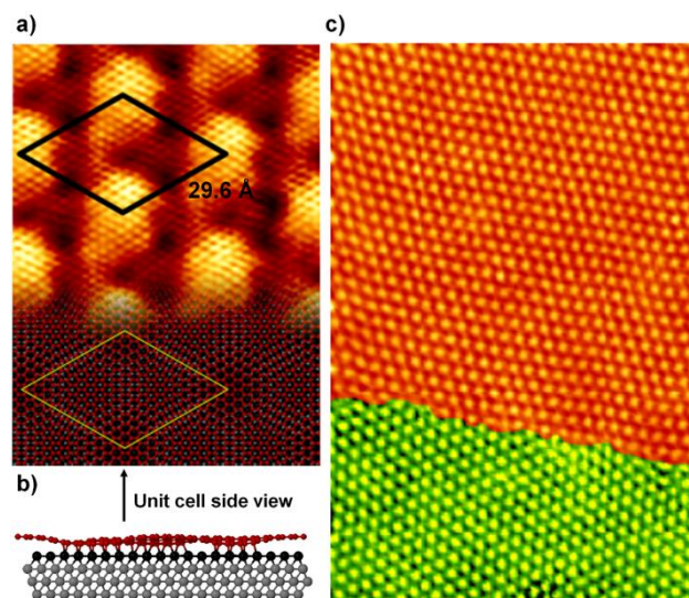
Fig. 1. (a) 7.5 × 10.5 nm 2 atomically resolved STM image ( V_s = -0.4 V, I_t = 2.0 nA) of 1ML graphene on Rh(111) where the structure of the (12 × 12) G moiré is observed. The DFT calculated atomic positions are overlaid on the bottom part of the image. (b) Ball and stick model of the DFT structure for the same moiré pattern. This side view highlights the large corrugation of the graphene layer (121 pm). (c) 63 × 96 nm 2 STM image ( V_s = 0.8 V, I_t = 0.9 nA) of 1ML graphene grown by UHV-CVD on Rh(111). Two different rotational domains are observed in the same terrace: the (12 × 12) G moiré is observed in the top while a different moiré pattern (highlighted in green) is resolved in the bottom.
