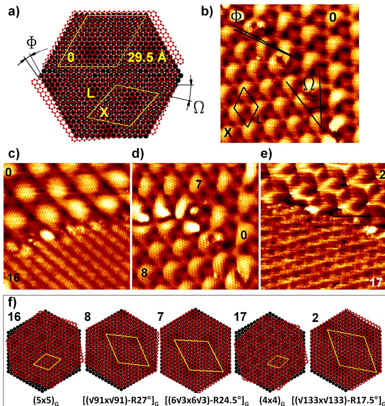
Fig. 2. Procedure to determine the new moirés' parameters: (a) schematic model in which both the "usual" ( 12 \times 12 ), moiré 0, and a new one (x) are compared. (b) 15 \times 15 \text{ nm}^2 STM image ( V_s = 0.3 \text{ V} , I_t = 18.7 \text{ nA} ) where both the moiré 0 and the new one appear together. The new moirés' parameters, characterized by the angles \Omega and \Phi (see text), are obtained comparing them to those already known from the moiré 0. (c-e) 12 \times 12 \text{ nm}^2 atomically resolved STM images where five moirés different from moiré 0 are shown. The corresponding numbers of these moirés are consistent with table 1. (c) On the bottom part of the image ( V_s = 38 \text{ mV} , I_t = 11.1 \text{ nA} ), the (5 \times 5)_G moiré (labeled as 16 in the figure) is observed; (d) the [(\sqrt{91} \times \sqrt{91}) - R27^\circ]_G moiré is on the bottom-left of the image (named as 8) while the [(6\sqrt{3} \times 6\sqrt{3}) - R24.5^\circ]_G moiré (labelled as 7) is on the top-left ( V_s = 0.3 \text{ V} , I_t = 18.7 \text{ nA} ); (e) on the bottom part of the image, the moiré number 17 corresponds to the (4 \times 4)_G superperiodicity, while number 2, in the top part, corresponds to [(\sqrt{133} \times \sqrt{133}) - R17.5^\circ]_G ( V_s = 0.7 \text{ V} , I_t = 15.7 \text{ nA} ). (f) Schematic models of the moirés obtained by STM measurements in the figures on top.
