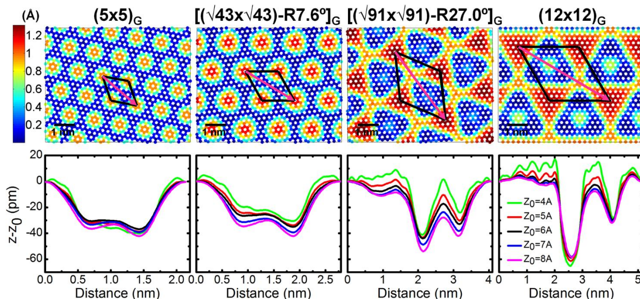
Fig. 4. (top) Colormaps (in Å) of the graphene heights obtained in the DFT simulations for the four different moiré patterns. Notice that all images have the same dimensions and color scale. (bottom) Constant current profiles along the high symmetry path marked in the corresponding top panels for different values of the current (different average heights). Profiles are calculated using a NEGF formalism at a voltage of -1.0 V and taking as reference the current calculated in the initial position with the tip placed at a z_0 height above the highest carbon atom.
