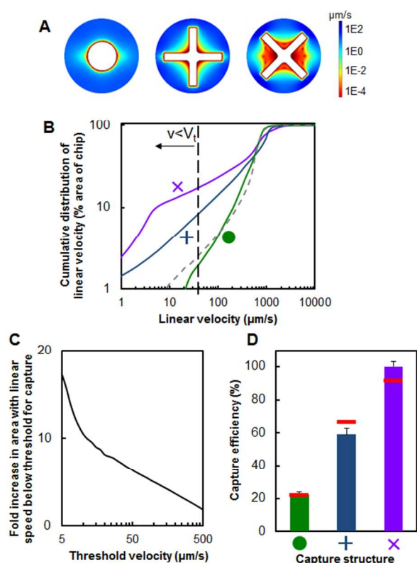
Figure 2. Optimization of the capture structures. (A) Spatial distribution of linear velocities in devices with 'x', '+', and 'o' shaped structures. Velocity valleys are in red. (B) Cumulative distribution of linear velocities in devices with various capture structure geometries compared to a device without structures. The y-axis is the percent area of the chip with linear velocity less than or equal to the corresponding value on the x-axis. X-shaped capture structures markedly increase the percentage area of the chip with low linear velocities. (C) X-shaped capture structures drastically increase the area with linear speed below the threshold for capture when compared to circular posts which do not generate velocity valleys. (D) Capture efficiency as a function of capture structure geometry for VCaP cells. The red lines represent the predicted capture efficiency as a function of structure geometry. Error bars represent standard error.
