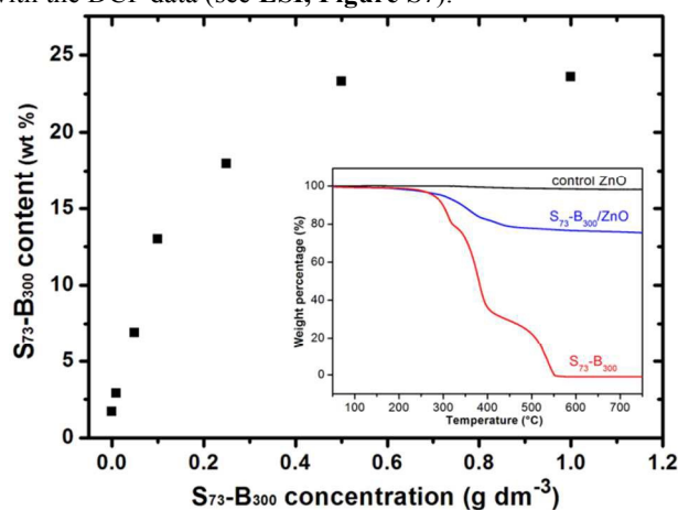
Figure 5. S_{73}\text{-}B_{300} mass contents within S_{73}\text{-}B_{300}/\text{ZnO} nanocomposites prepared using various S_{73}\text{-}B_{300} nanoparticle concentrations, as determined by thermogravimetry. Inset shows the weight loss curves obtained for ZnO alone, a S_{73}\text{-}B_{300}/\text{ZnO} nanocomposite prepared using 0.50 \text{ g dm}^{-3} S_{73}\text{-}B_{300} nanoparticles, and the precursor S_{73}\text{-}B_{300} nanoparticles.
