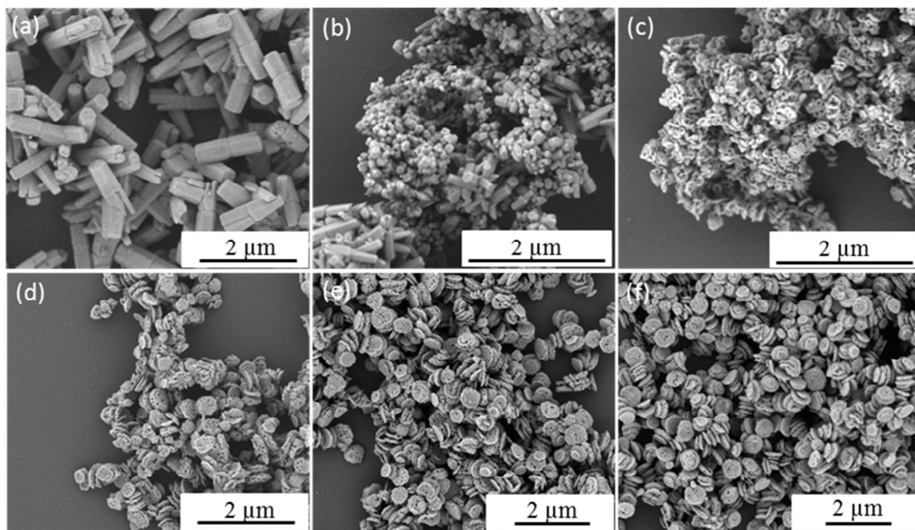
Figure 3. Representative SEM images showing ZnO particles prepared in the presence of various concentrations of S_{73} - B_{300} copolymer nanoparticles: (a) 0.0 \text{ g dm}^{-3} ; (b) 0.01 \text{ g dm}^{-3} ; (c) 0.05 \text{ g dm}^{-3} ; (d) 0.10 \text{ g dm}^{-3} ; (e) 0.50 \text{ g dm}^{-3} ; (f) 1.00 \text{ g dm}^{-3} .
