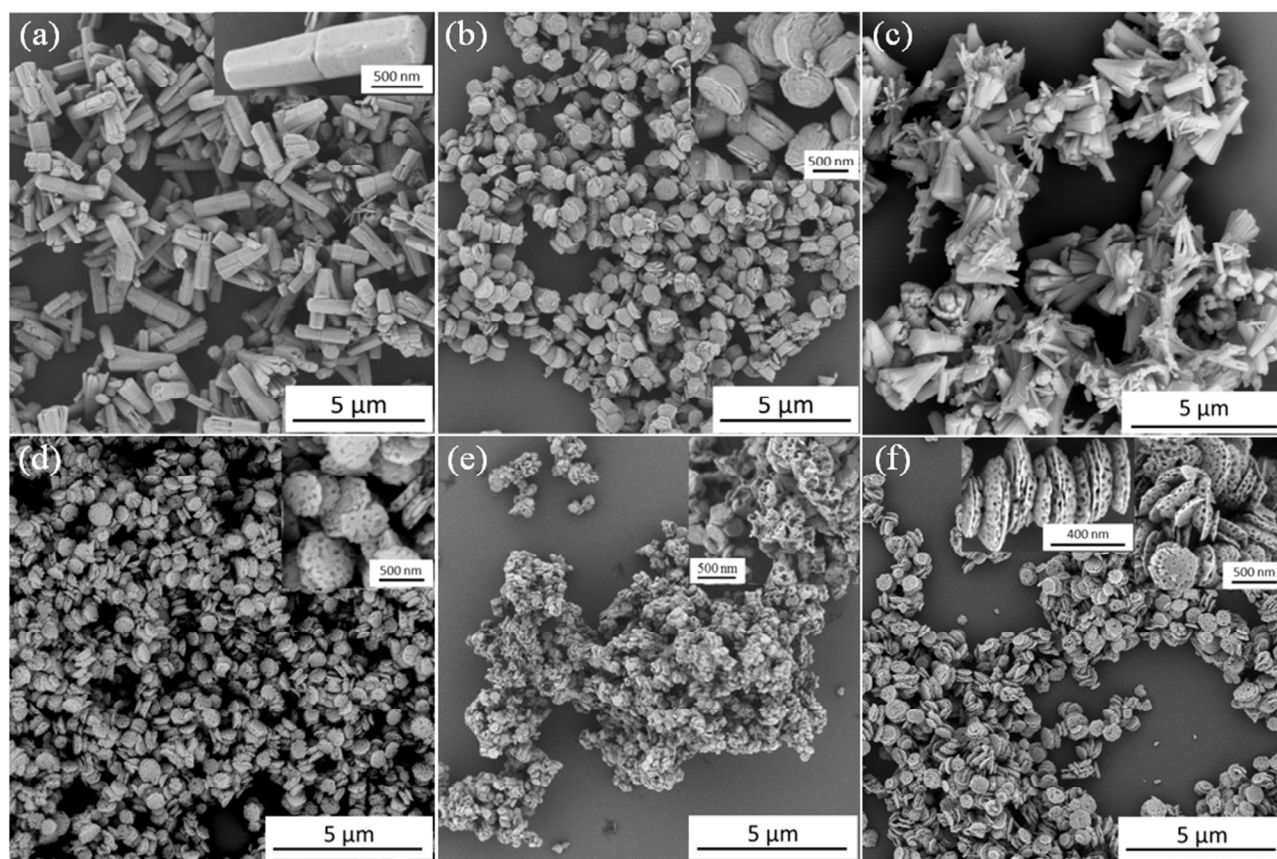
Figure 2. SEM images of ZnO particles mineralised under various conditions after calcination at 700 °C: (a) without any additive; (b) in the presence of 0.12 g dm -3 PSEM 73 homopolymer (i.e. the number of moles of PSEM 73 homopolymer is equivalent to the number of moles of S 73 -B 300 nanoparticles used in (f)); (c) 0.50 g dm -3 M 68 -B 300 ; (d) 0.50 g dm -3 [0.5 S 73 + 0.5 M 68 ]-B 300 ; (e) 0.50 g dm -3 S 32 -B 300 ; (f) 0.50 g dm -3 S 73 -B 300 . The insets present the corresponding magnified images.
