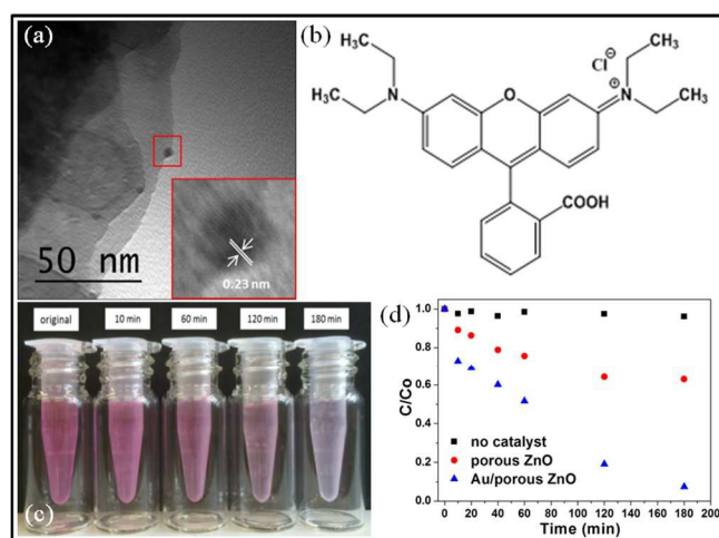
Figure 8. (a) TEM image of Au/ZnO nanocomposite particles; inset shows the Au nanoparticles with a mean diameter of ~ 5 nm; (b) chemical structure of rhodamine B (RhB) dye; (c) digital photograph of aqueous solutions of RhB illustrating the gradual UV photodegradation of this dye after various irradiation times; (d) Relative photocatalytic activities of porous ZnO particles and Au/ZnO nanocomposite particles after UV-induced degradation of RhB dye at room temperature ( \lambda = 254 nm, 6 W; Au catalyst concentration is fixed at 0.50 g dm -3 , initial RhB concentration = 1 \times 10^{-5} M; here C/C_0 denotes the ratio of the concentration, C , at any given time to the original concentration, C_0 ).
