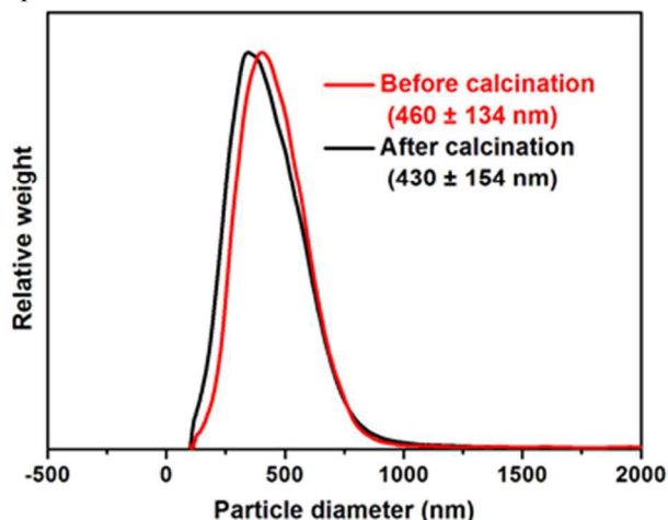
Figure 4. Weight-average particle size distributions determined for ZnO particles prepared in the presence of 0.50 \text{ g dm}^{-3} S_{73}\text{-}B_{300} copolymer nanoparticles before and after calcination, as determined by disc centrifuge photosedimentometry. Particle densities were calculated to be 3.17 and 5.31 \text{ g cm}^{-3} for the S_{73}\text{-}B_{300}/\text{ZnO} precursor nanocomposite particles and calcined ZnO particles, respectively.
