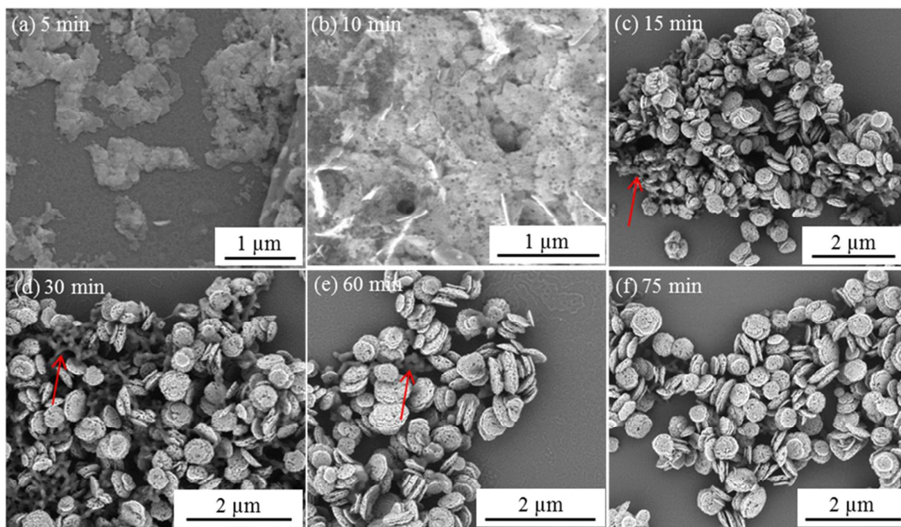
Figure 7. Representative SEM images showing the evolution in morphology for ZnO prepared in the presence of S_{73} - B_{300} copolymer nanoparticles at various reaction times: (a) 5 min; (b) 10 min; (c) 15 min; (d) 30 min; (e) 60 min; (f) 75 min. The red arrows indicate the presence of impurities, which are likely to be \text{Zn}(\text{OH})_2 .
