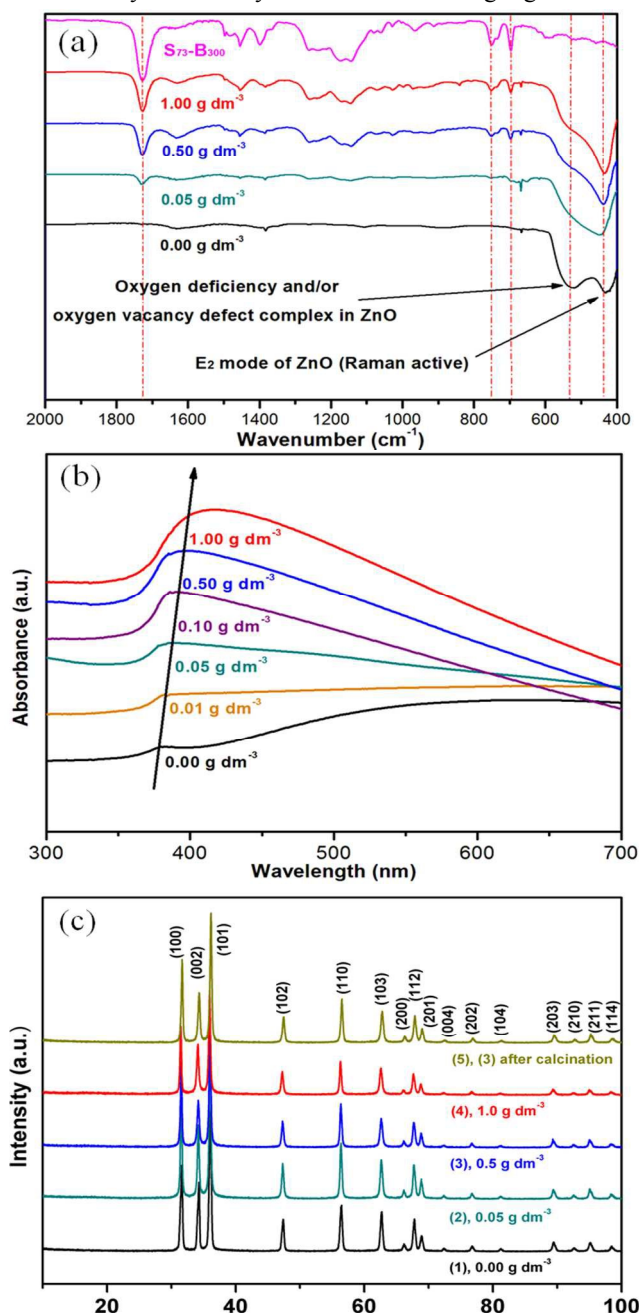
Figure 6. (a) FT-IR spectra recorded for ZnO nanocomposites prepared using various S_{73}\text{-}B_{300} nanoparticle concentrations and also a reference spectrum for S_{73}\text{-}B_{300} nanoparticles alone; (b) UV-visible absorption spectra recorded for ZnO particles prepared in the presence of various S_{73}\text{-}B_{300} nanoparticle concentrations after calcination; (c) XRD patterns obtained for ZnO particles prepared in the presence of various S_{73}\text{-}B_{300} nanoparticle concentrations.
