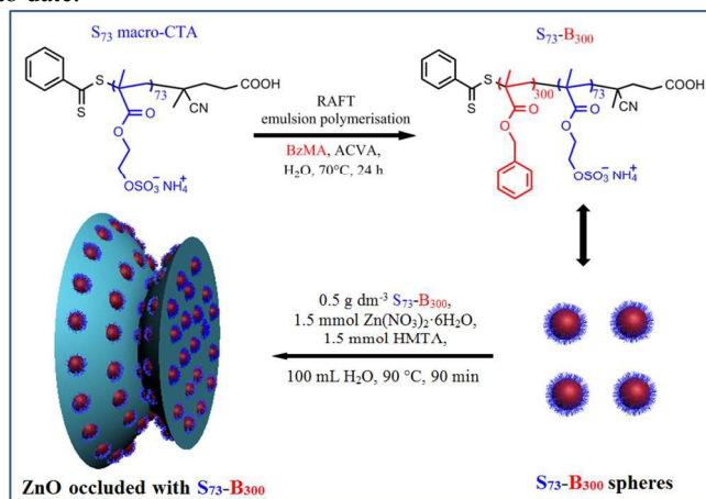
Scheme 1. RAFT aqueous emulsion polymerisation of benzyl methacrylate (BzMA) using a PSEM 73 macromolecular chain transfer agent (macro-CTA) at 70 °C to produce PSEM 73 -PBzMA 300 (S 73 -B 300 ) diblock copolymer nanoparticles and associated cartoon showing S 73 -B 300 spherical nanoparticles and their occlusion within zinc oxide.
