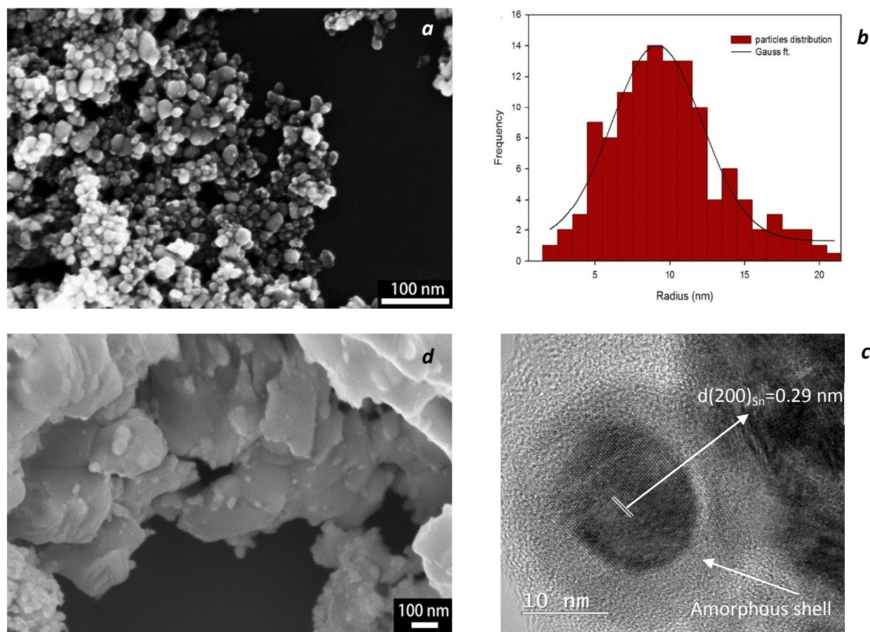
Fig. 1 SEM image of as-synthesized SAC particles with ( a ) and without ( d ) the use of surfactant (PVP). A size distribution histogram of the particles in ( a ) is presented in ( b ). The HRTEM image of a nanoparticle from ( a ) is shown in ( c ) which consists of a well-crystallized \beta -Sn core of ca. 18 nm diameter covered with an amorphous layer of ca. 5 nm.
