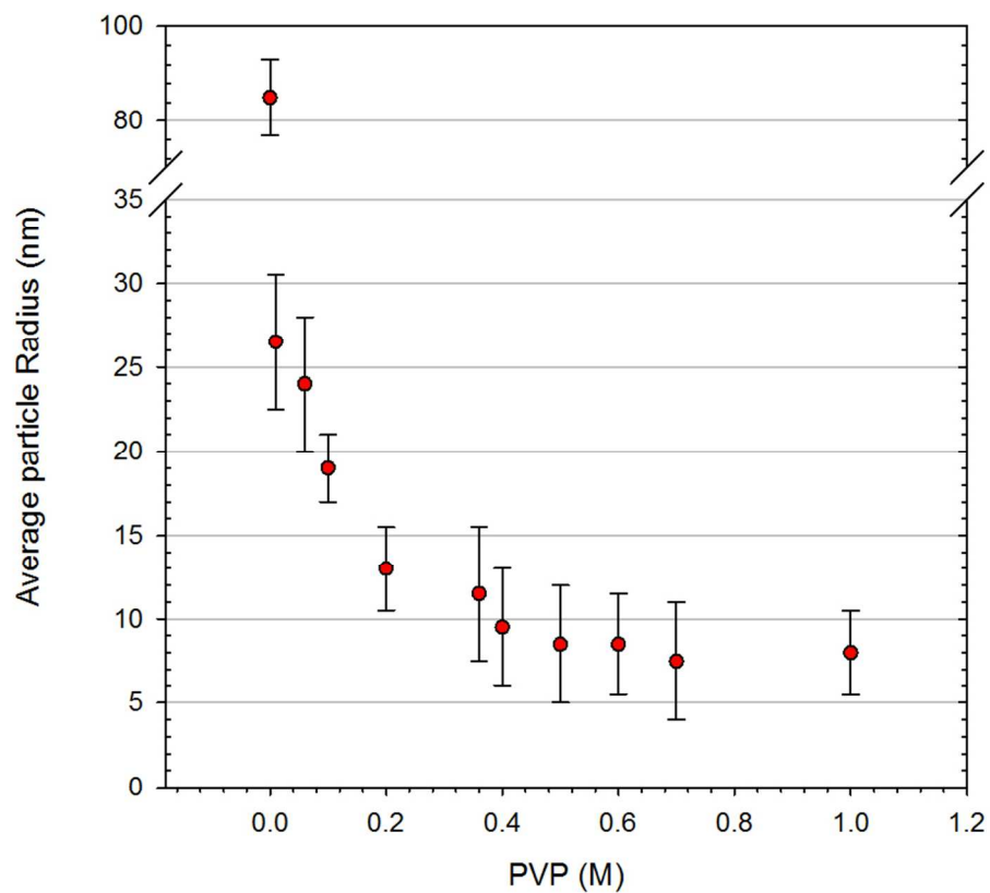
Fig.2 The effect of PVP concentration on average particle size ( r ) of nanoparticles
