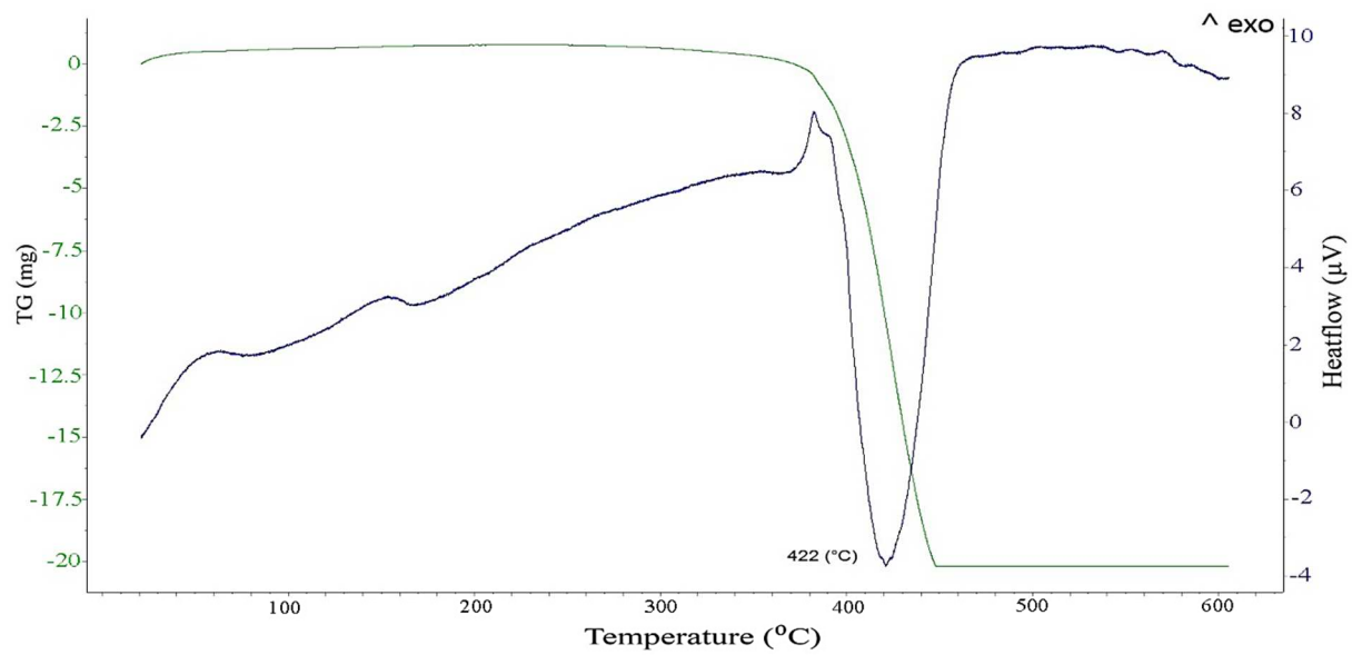
Fig. 5 DSC/TG curves of PVP dissolved in DEG
