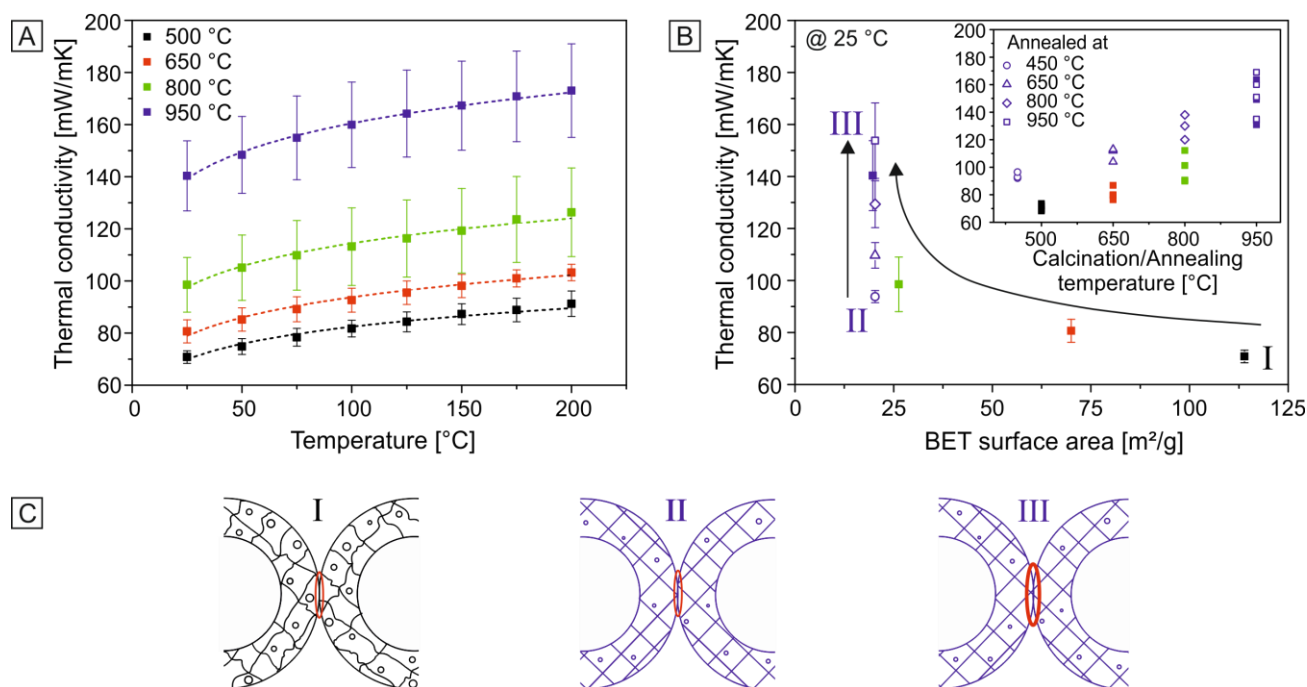
Fig. 6 Thermal conductivity of calcinated (closed symbols) and annealed HSNP colloidal crystals (open symbols). A) Thermal conductivity of HSNP monoliths calcinated at different temperature (500 – 950 °C) as a function of the measurement temperature. The dashed lines represent \kappa \sim T^x . B) BET surface area and calcination temperature (inset) as a function of the thermal conductivity at 25 °C measurement temperature. C) Schematic representation of the internal structural changes and the increase in interfacial adhesion within a colloidal crystal ensemble.
