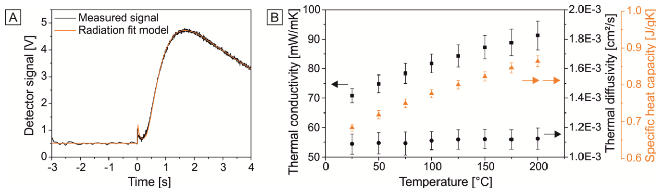
Fig. 5 LFA measurements of HSNP calcinated at 500 °C. A) Measured signal (black line) with radiation fit model (orange line). B) Summary of the necessary input parameters (thermal diffusivity – black circles and mean specific heat capacity – orange triangles) to determine the thermal conductivity (black squares).
