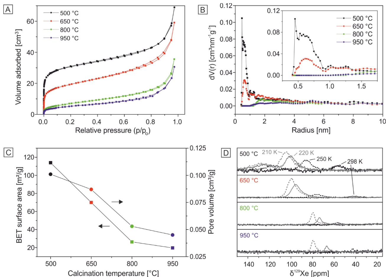
Fig. 2 Internal structural characterization of hollow silica spheres in dependence of the calcination temperature: A) Nitrogen adsorption and desorption isotherms measured at 77 K allow the determination of pore volume and surface area. B) Pore radius distributions, calculated by applying NLDFT silica kernel based on a cylindrical pore model, indicate closure of the micropores at higher calcination temperatures. C) BET surface area (squares) and pore volume (dots) as a function of calcination temperature. D) ^{129}\text{Xe} NMR spectra of hyperpolarized xenon in silica hollow spheres as a function of the sample temperature. Even for the highest calcination temperatures a small amount of micropores is still present in the silica shell.
