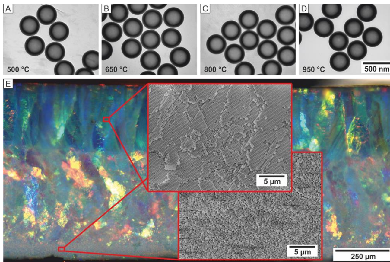
Fig. 1 A-D) TEM images of hollow silica nanoparticles at different calcination temperatures (500 – 950 °C). The particle dimensions remain constant for the various calcination temperatures and do not show any clustering. E) Correlative light and electron microscope (CLEM) images of a HSNP colloidal crystal calcinated at 500 °C. The bright colors are caused by coherent Bragg scattering. Most of the crystal is in a fully crystalline state as confirmed by the scanning electron microscopy (SEM) insets.
