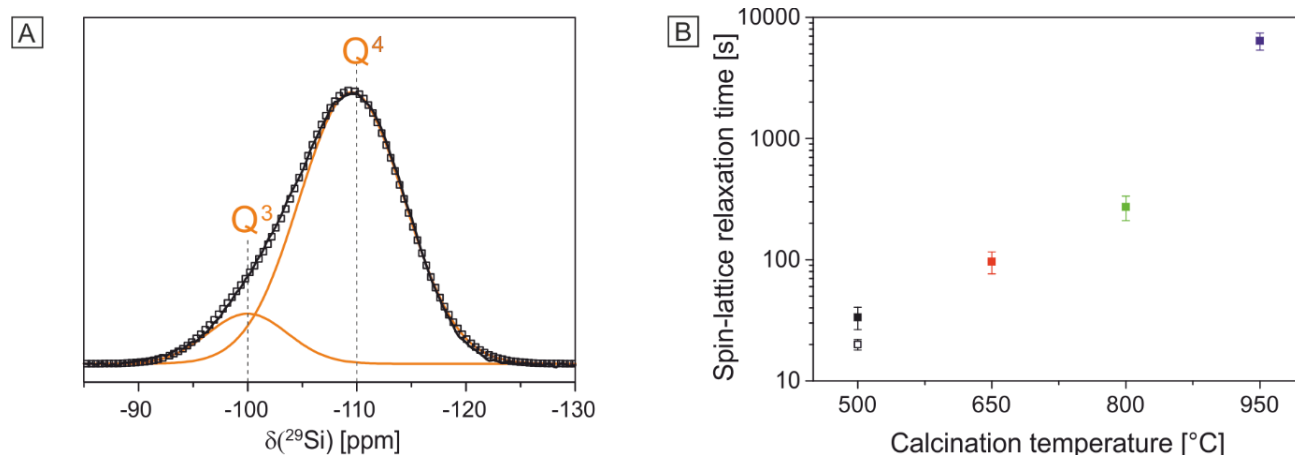
Fig. 3 Internal structural characterization of hollow silica spheres. A) Deconvoluted projection of the 29 Si spectrum of HSNP calcinated at 500 °C; measured signal (black line), cumulative fit (open squares), simulated signals (orange lines), B) Spin-lattice relaxation time of silica hollow spheres calcinated at different temperatures. The closed symbols represent untreated and the open symbol pre-dried powder to remove water residues.
