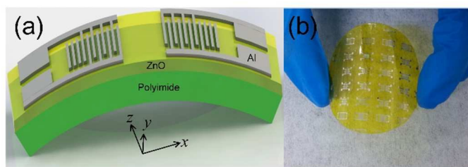
Fig.1 Schematic view of the flexible SAW device (a) and a photograph of the flexible devices fabricated (b).
