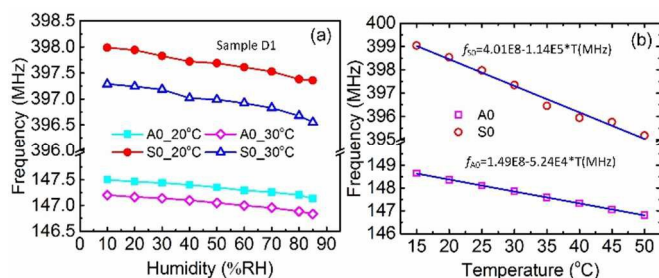
Fig.6 The resonant frequency of D1 as a function of humidity at 20°C and 30°C (a) and as a function of temperature at 30%RH (b). The temperature coefficient of frequency for both the wave modes has an excellent linearity with the correlation coefficient of 0.9996 for A0 and 0.9832 for S0.
