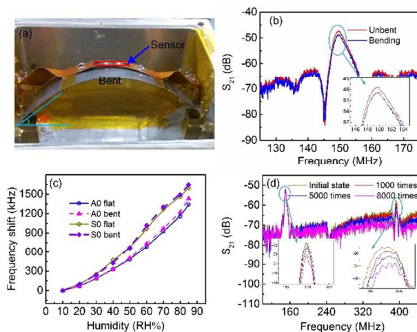
Fig.7 Photograph of the sensor at a bent state (a); Comparison of transmission spectra (b), frequency shifts of a flexible humidity sensor ( \lambda=12 \mu\text{m} , D3) unbent and bent at an angle of 36°(c), and (d) the dependence of the transmission property of the sensor as a function of bending cycles.
