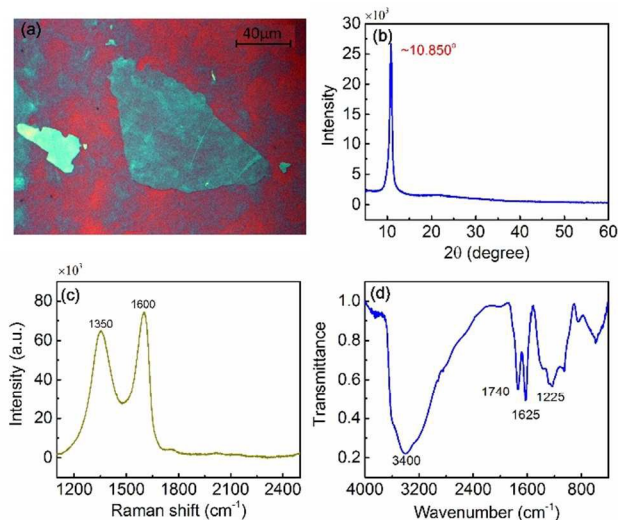
Fig. 3 A microscope image of the graphene oxide microflakes on \text{SiO}_2/\text{Si} substrate; (a) X-ray diffraction curve (b); Raman spectrum recorded with \lambda_{\text{exc}} = 532 \text{ nm} (c), and FTIR spectrum (d) of the GO film.
