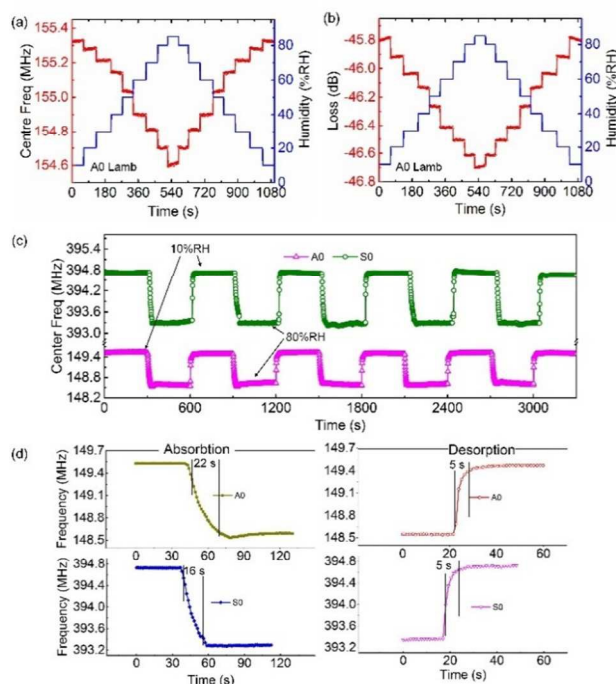
Fig.5 Detailed responses of the resonant frequency shift (a) and insertion loss (b) of the A0 mode, sample D3 to humidity change; the repeatability of the frequency of the A0 and S0 (c) modes of sample D3 when the humidity was repeatedly changed from 10%RH to 80%RH. (d) Detailed frequency response curves, showing the response and recovery times of the sensor (D3).
