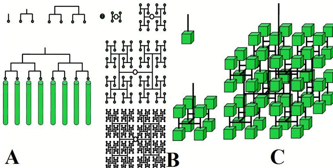
Figure 6. A set of 1D distributors feeding progressively larger 1D arrays (vectors); b-c) extension of the scalable, fractal distributor concept to 2D and 3D, respectively. 47 Copyright 2015 Wiley.
