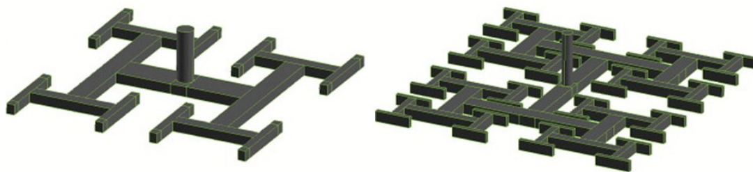
Figure 8. Fractal design with 16 and 64 outlets used for modeling studies. 98 Reprinted from 98 with permission from Elsevier.
