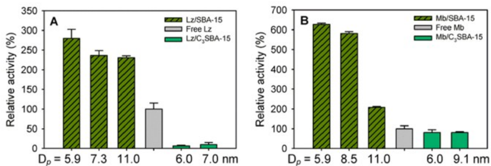
Figure 3. Relative, intrinsic catalytic activities of enzymes immobilized on the surface of SBA-15 pores (green hashed bars), free in solution (grey bar), and inside of hydrophobic, propyl-modified SBA-15 pores (light green bars). Results are shown for a characteristic hydrolysis reaction catalyzed by lysozyme (A) and an oxidation reaction catalyzed by myoglobin (B). 30
