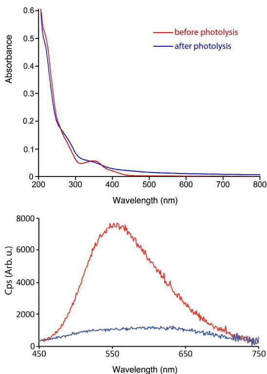
Figure 8. Experimental absorption (top) and emission (bottom) profiles of 2a from dilute acetonitrile solutions ( ca\ 10^{-5} M) at room temperature before and after exhaustive photolysis. The emission profiles were obtained by exciting the complex at 350 nm. The same colour coding is used between the absorption and emission profiles.
