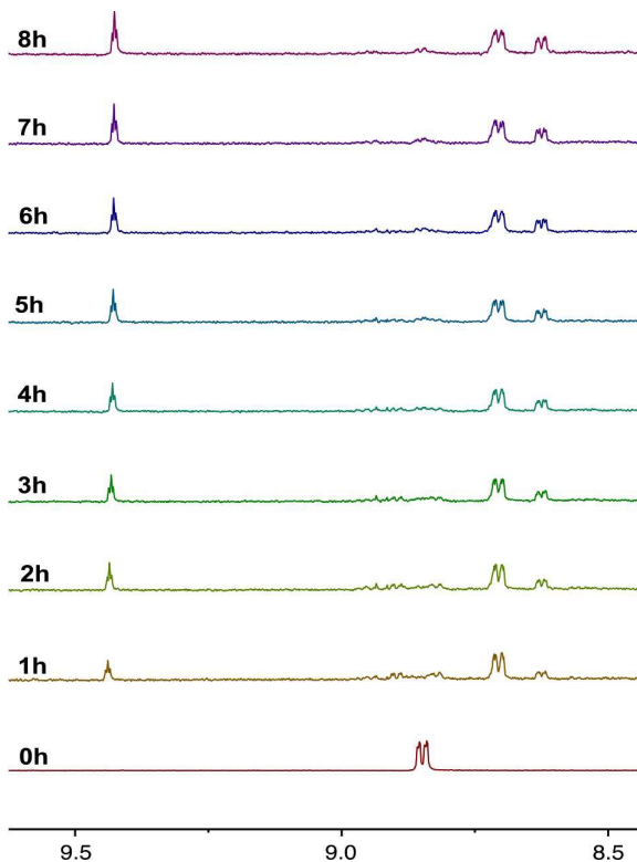
Figure 5. ^1\text{H} NMR progression of the photolysis of 2a in deuterated acetonitrile solutions. The photolysis was performed by irradiating the sample at 365 nm over a period of 8 h.
