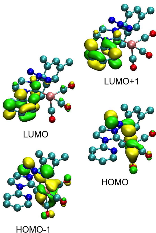
Figure 4. Selected orbital representations for 2a .
