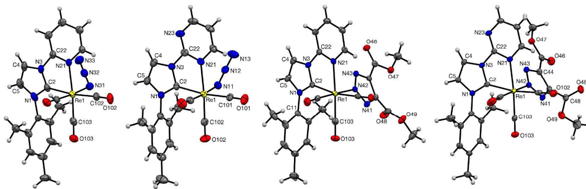
Figure 2. X-Ray structures of the complexes 2a,b and 3a,b . Disordered groups and solvents present in the unit cell have been omitted for clarity. Ellipsoids are displayed at the 50% probability level.
