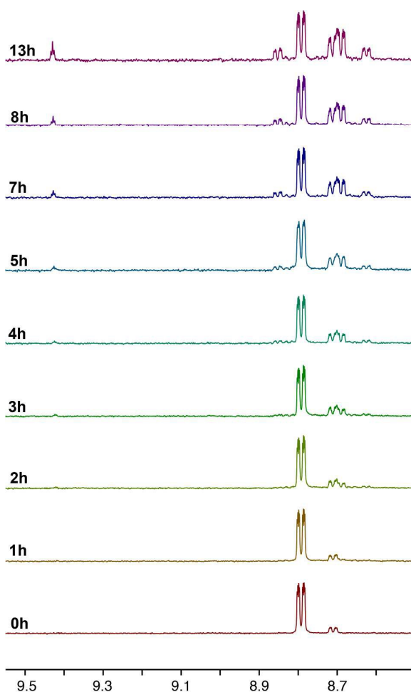
Figure 9. ^1\text{H} NMR progression of the photolysis of 3a in deuterated acetonitrile solutions. The photolysis was performed by irradiating the sample at 365 nm over a period of 13 h.
