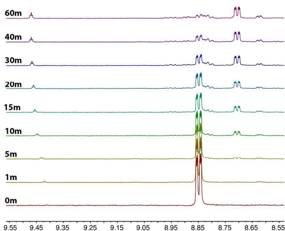
Figure 6. ^1\text{H} NMR progression of the photolysis of 2a in a deuterated acetonitrile solution. The photolysis was performed by irradiating the sample at 365 nm over a period of 1 h.
