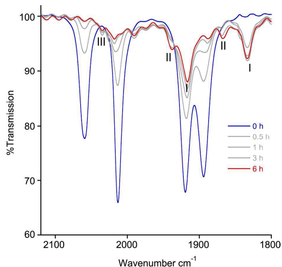
Figure 7. IR progression of the photolysis of 2a in an acetonitrile solution. The photolysis was performed by irradiating the sample at 365 nm over a period of 6 h. For clarity, all traces except the first and last have been drawn in grey.
