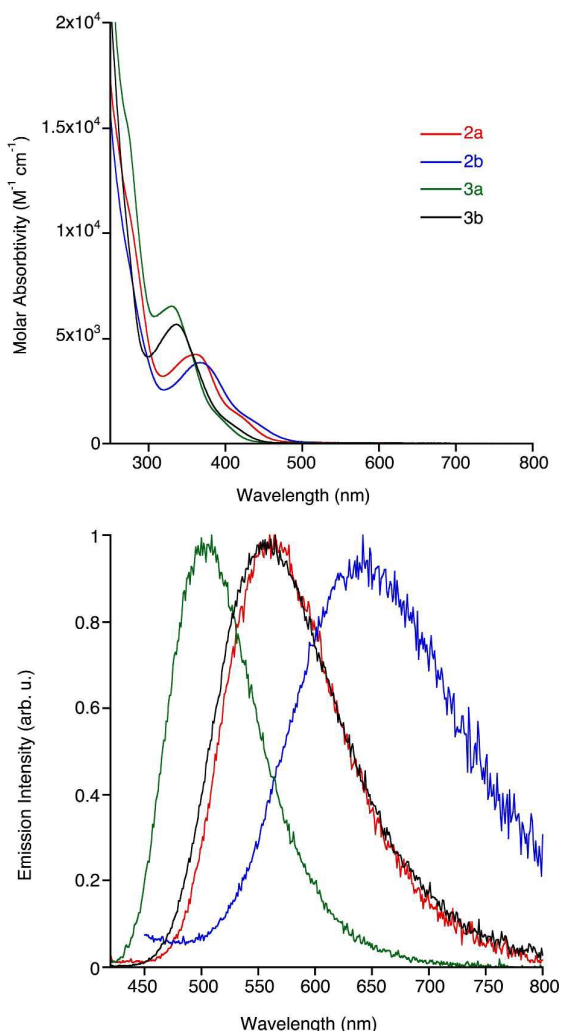
Figure 3. Experimental absorption (top) and emission profiles (bottom) of the complexes from dilute dichloromethane solutions ( \approx 10^{-5} M) at room temperature. The emission profiles were obtained by exciting the complexes to their lowest energy \lambda_{\text{abs}} . The same colour coding (inset) is used between the absorption and emission profiles.
