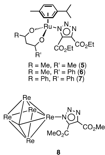
Figure 1. Previously reported cases of triazolate ligands bound to a metal centre through the N(1) nitrogen atoms. The phosphorous, selenium, carbon, and hydrogen atoms of the cluster core have been removed for clarity.
