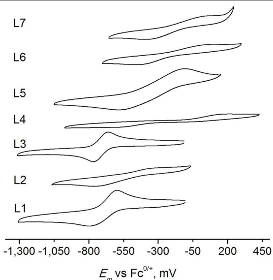
Fig. 7. Cyclic voltammograms of copper complexes with different ligands.
