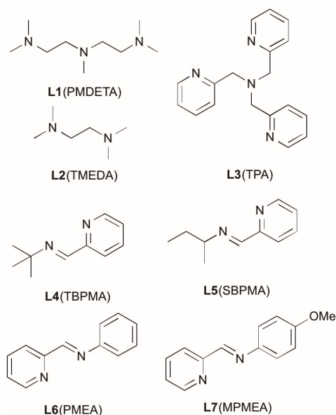
Scheme 1 N -based ligands: L1 : N,N,N',N'',N'' -pentamethyldiethylenetriamine (PMDETA); L2 : N,N,N',N' -Tetramethylenediamine (TMEDA); L3 : Tris (2-Pyridylmethyl)amine (TPA); L4 : ( E )- N -tert-butyl-1-(pyridin-2-yl)methanimine (TBPMA); L5 : ( E )- N -sec-butyl-1-(pyridin-2-yl)methanimine (SBPMA); L6 : ( E )- N -(pyridin-2-ylmethylene)aniline (PMEA); L7 : ( E )-4-methoxy- N -(pyridin-2-ylmethylene)aniline (MPMEA).
