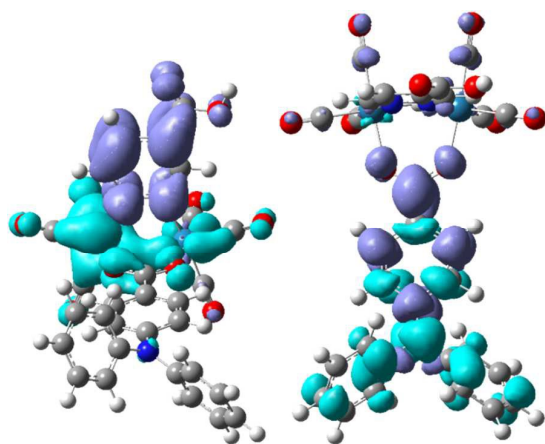
Fig. 2 Electronic density difference maps for the two most intense electronic transitions computed for the rhenium complex [Re 2 H(OOC-TPA)(CO) 6 (pydz-4-COOH)] ( 3 ): the MLCT at 530 nm (left) and the \pi - \pi^* at 344 nm (right). Light blue indicates a decrease in electron density, blue indicates an increase.
