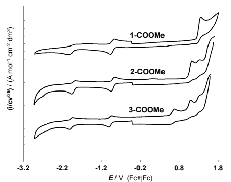
Fig. 3 Normalized CV features of the methyl-ester derivatives of the three dyes on GC electrodes, in MeCN + 0.1 M (\text{NBu}_4)\text{PF}_6 solution, at 0.2 \text{ V s}^{-1} with ohmic drop compensation.
