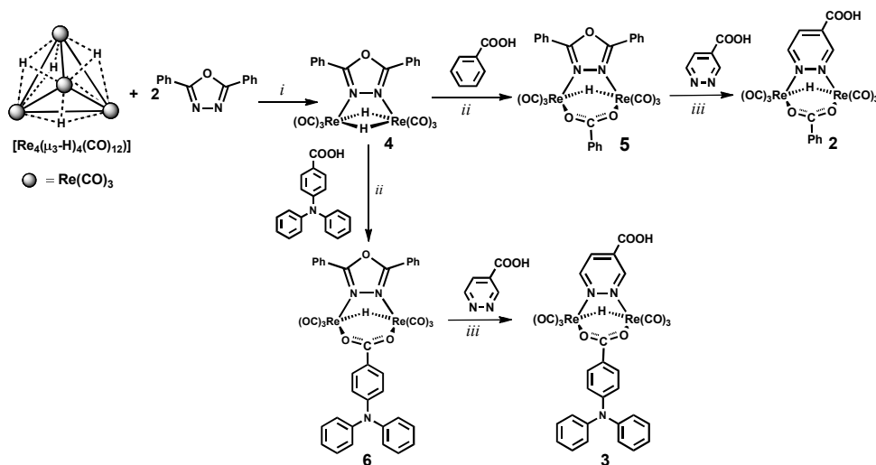
Scheme 1 Synthetic pathways for the preparation of the rhenium complexes 2 and 3 . Reaction conditions: i) \text{CH}_2\text{Cl}_2 , room temperature, 24 h; ii) toluene reflux, 2 h; iii) THF reflux, 12 h.
