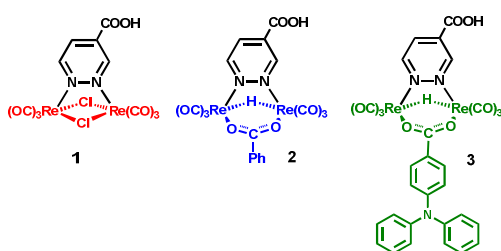
Chart 1 Molecular structure of the three dyes
