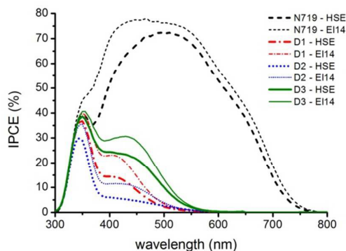
Fig. 6 IPCE spectra for DSSC devices sensitized by different dyes: 1 with HSE electrolyte (thick red dash-dotted line) and with EI14 electrolyte (thin red dash-dotted line); 2 (dotted blue lines); 3 (solid green lines); N719 as reference dye (dashed black lines). Two different iodide/triiodide electrolytes were used, a commercially available one (HSE, Dyesol) and another developed in-house (labeled EI14).
