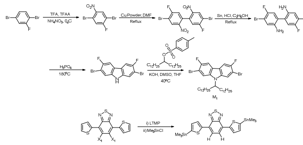
Scheme 1. Synthetic routes to the final monomer products: M1 , M3 and M4 . M2 was synthesised using previously established literature procedures.
