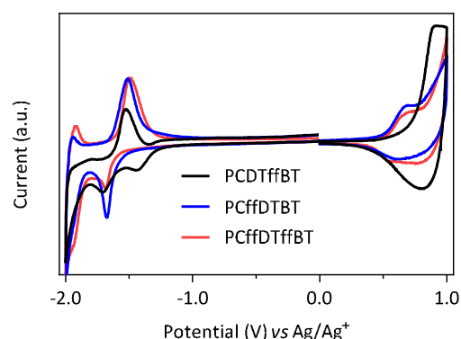
Figure 4. Cyclic voltammograms of PCDTffBT , PCffDTBT and PCffDTffBT on platinum disc electrodes (area 0.031 cm 2 ) at a scan rate of 100 mV s -1 in acetonitrile/tetrabutyl ammonium perchlorate (0.1 mol dm -3 ).
