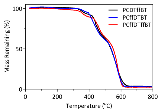
Figure 5. Thermogravimetric analysis of PCDTffBT , PCffDTBT and PCffDTffBT with a heating rate of 10°C min -1 under an inert nitrogen atmosphere.
