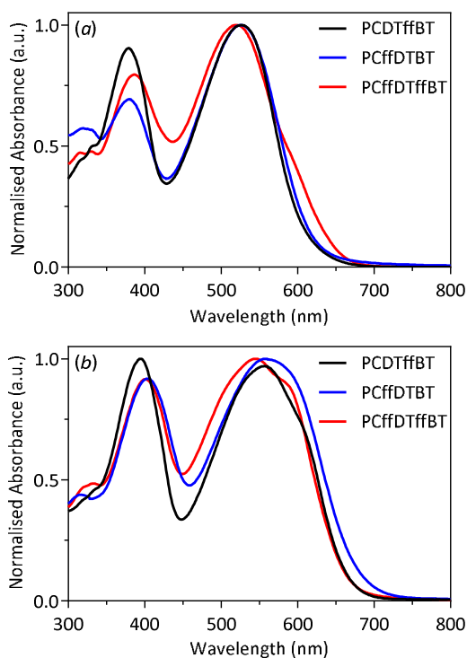
Figure 2. Normalised UV-vis absorption spectra of PCDTffBT , PCffDTBT and PCffDTffBT in: (a) chloroform solution; and (b) thin films.
