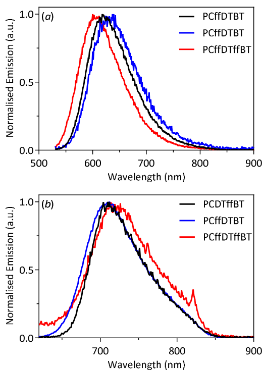
Figure 3. Normalised fluorescence spectra of PCDTffBT , PCffDTBT and PCffDTffBT in: (a) chloroform solution; and (b) thin films.
