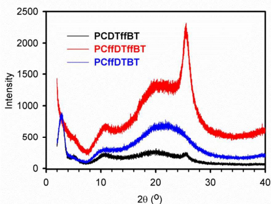
Figure 6. Powder X-ray diffraction (XRD) patterns of PCDTffBT , PCffDTBT and PCffDTffBT .
