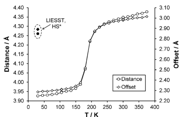
Figure 6 - Change in centroid (N2, C2-C6) to centroid (N2#3, C2#3-C6#3, where #3 = 2-x, 1-y, 1-z) (o) distance and (◊) offset with temperature. ● and ◆ denote distance and offset observed respectively for the HS* structure at 30 K. Error bars are included but obscured by the data markers.
