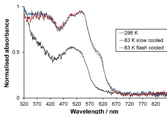
Figure 10 - Normalised single crystal UV-Vis absorption spectra collected at 298 K (HS) and 83 K (LS) for [\text{Fe}(\text{abpt})_2(\text{NCS})_2] polymorph A . The consistency in the spectrum at 83 K independent of cooling strategy is also shown.
