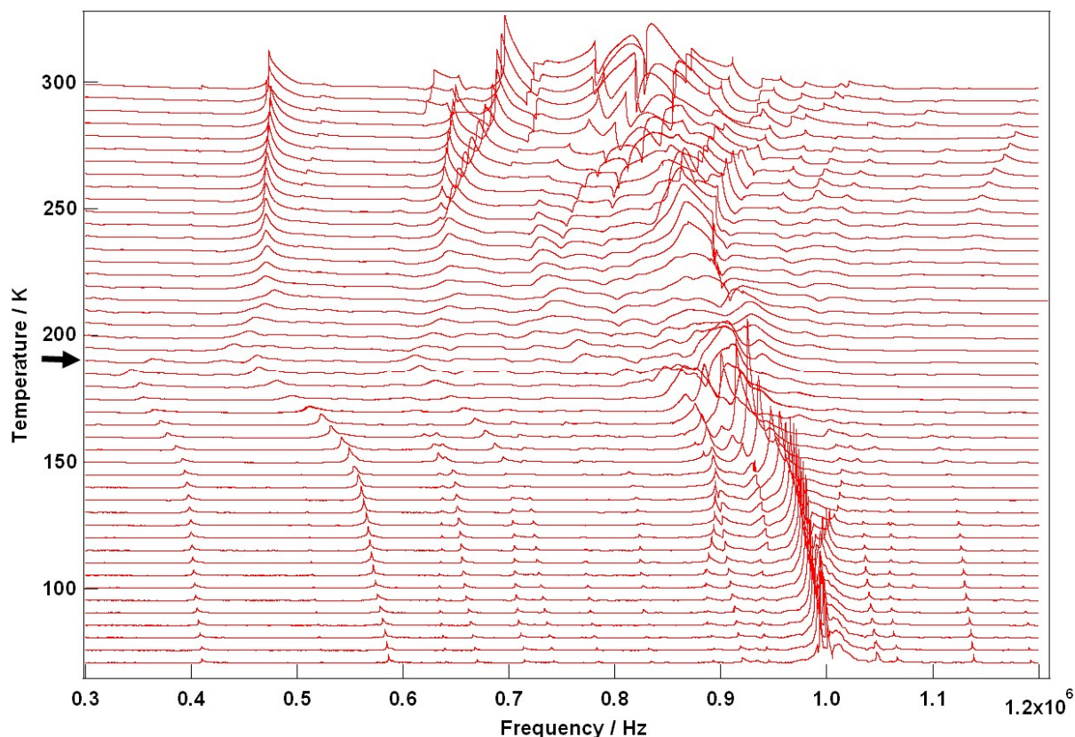
Figure 11 - Stack of RUS spectra as a function of frequency for [\text{Fe}(\text{abpt})_2(\text{NCS})_2] polymorph A from 70 - 300 K, the arrow at around \sim 190 K indicates the spin crossover transition, T_{1/2} = 188 K. 12
