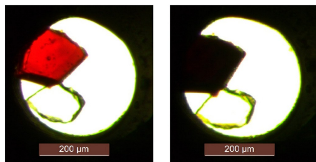
Figure 9 - Photograph of a single crystal of A loaded in the DAC showing the colour change associated with the pressure induced spin transition: (left) ambient pressure, (right) 5.1(2) kbar.
