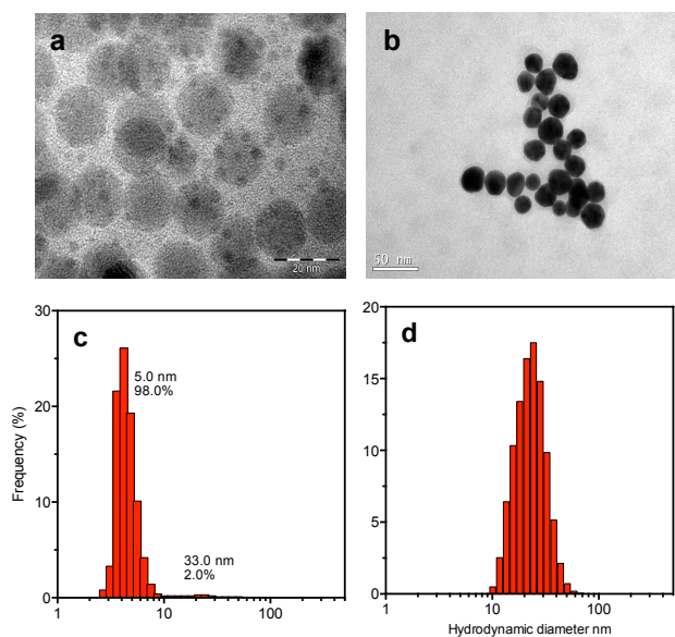
Figure 2. a) TEM image of type 1 HtAuNP produced by adding \text{HAuCl}_4 over Ht, displaying two sizes, 3.5 and 15 nm and b) TEM image of type 2 HtAuNP produced by adding Ht over \text{HAuCl}_4 , showing a homogeneous population of 15 nm. Size distribution of each HtAuNP suspension was also measured by DLS, accordingly, in c) type 1 HtAuNP were polydisperse suspensions of 5 nm and 33 nm, while in d) only one population of 32 nm was found for type 2 HtAuNP.
