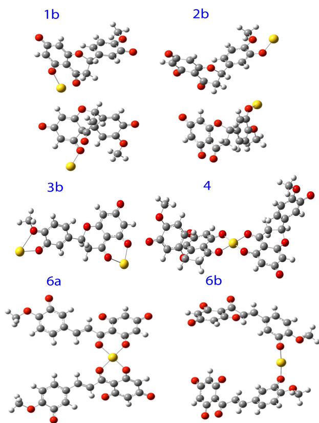
Figure 8. Final structures of complexes formed in the systems Au +3 :Ht -3 1:1 1b and 2b, before (upper panel) and after (lower panel) the full geometrical optimization. Followed by structural geometries for Au +3 :Ht -3 at ratios 2:1 (system 3b) and 1:2 (system 4). And finally the geometries for the four-fold coordination system 6a and the two-fold coordination system 6b of the Au +3 :2Hc -4 interactions.
