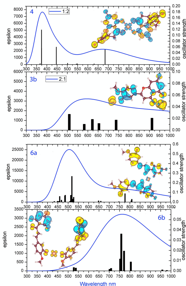
Figure 9. Optical spectra and electronic density differences maps (EDDM) between the ground state and the most "f" intense excited state for Au 3+ :Ht 3- 1:2 (system 4) and b) 2:1 (system 3b) and Au 3+ :Hc 4- 1:2, (systems 6a and 6b). (*) Excited charge density is represented in cyan and the ground state density is represented in yellow. The iso-density surface is obtained at 0.0002 au. The quantity epsilon stands for the molar absorption coefficient proportional to the imaginary part of the dielectric constant.
