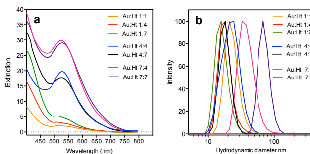
Figure 3. Ht reduces efficiently \text{HAuCl}_4 and yields self-stabilized gold nanoparticles with hydrodynamic diameters up to 68 nm and SPR values in the range of 520–530 nm. a) UV-visible spectra of two-fold diluted gold nanoparticles formed by the addition of different concentrations of \text{HAuCl}_4 (1, 4, and 7 \text{mmolL}^{-1} ) into alkaline solutions of Ht (1, 4, and 7 \text{mmolL}^{-1} ) recorded after 60 minutes of reaction. b) Size distribution measured by DLS.
