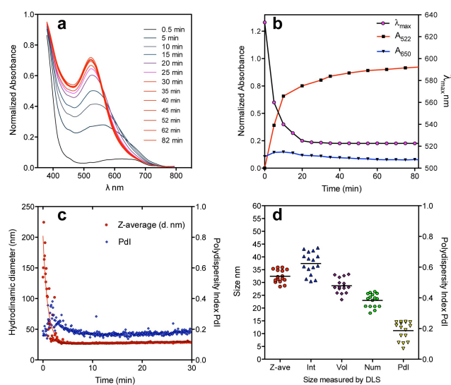
Figure 4. HtAuNP are synthesized within 30 minutes, starting with black colored suspensions formed by large aggregates that gradually decrease in size. The time course of the reaction at room temperature of a mixture of chloroauric acid and hesperetin at molar ratio of 1 and concentration of 4 \text{ mmol L}^{-1} and pH 11 was monitored by a) UV-Vis spectra after 0.5 min (black), 5 min (dark gray), 10 min (dark violet), 15 min (violet), 20 min (magenta), 25 min and (ruby red). b) Position ( \lambda_{\text{max}} ) of the main plasmon peak and absorbance at 522 and 650 nm. c) Hydrodynamic diameter (Zeta-average) and polydispersity index measured, and d) Size of different batches of HtAuNP measured by DLS.
