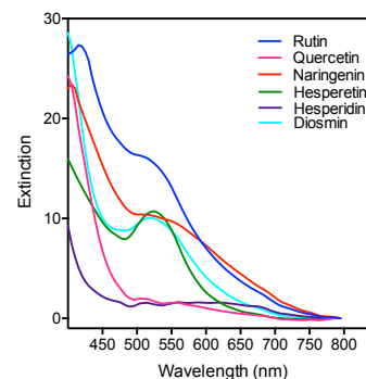
Figure 1. Flavonoids diosmin and hesperetin reduce HAuCl 4 and yield self-stabilized gold nanoparticles. UV-Vis spectra of alkaline solutions of flavonoids (2 mmolL -1 ) with the addition of chloroauric acid (2 mmolL -1 ) recorded after 60 minutes of reaction.
