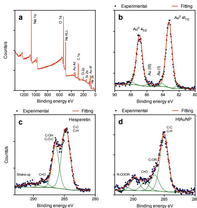
Figure 7 XPS measurements a) XPS survey spectrum of the film formed by dropping and drying on silicon substrate hesperetin reduced and self-stabilized
