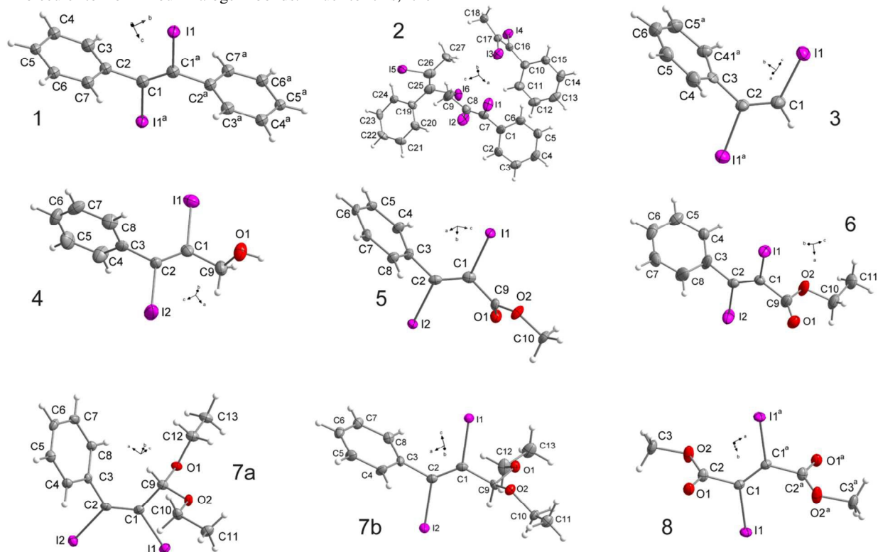
Figure 6 Overview over the asymmetric units or molecular structures of our compounds 1-8 with the specific atom numbering. Symmetry codes: 1 [a (1-x, 1-y, 2-z)]; 3 [a (1-x, y, 1.5-z)]; 8 [a (2-x, -y, 1-z)]. DIAMOND representation, thermal ellipsoids are drawn at 50% probability level.
