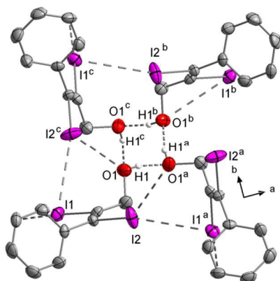
Figure 12 Helix along the c -axis in the crystal structure of 4 . All C-H hydrogen atoms are omitted for clarity. Symmetry codes: a (-0.25+ x , 1.25- y , 0.75+ z ), b (1.5- x , 1- y , -0.5+ z ), c (1.25- x , 0.25+ y , 0.25+ z ). DIAMOND representation, thermal ellipsoids are drawn at 50% probability level.
