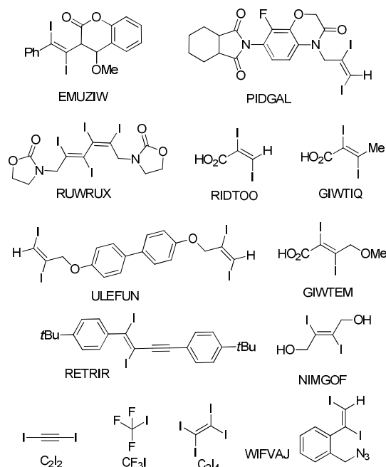
Figure 4 (E)-Diiodo olefines from the literature with their names from CSD.
