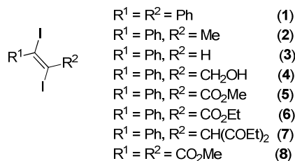
Figure 1 Additional ( E )-iodoolefines that have been synthesized from the corresponding alkyne.
