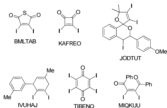
Figure 3 (Z)- and cyclic diiodo compounds from the literature with their names from CSD.
