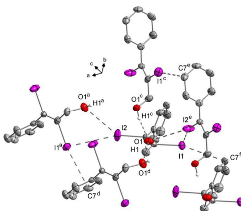
Figure 13 All intermolecular interactions emanating from the asymmetric unit. All C-H hydrogen atoms are omitted for clarity. Symmetry codes: a (-0.25+ x , 1.25- y , 0.75+ z ), c (1.25- x , 0.25+ y , 0.25+ z ), d (-0.25+ x , 1.25- y , -0.25+ z ), e (1.25- x , 0.25+ y , -0.75+ z ), f ( x , y , -1+ z ). DIAMOND representation, thermal ellipsoids are drawn at 50% probability level.
