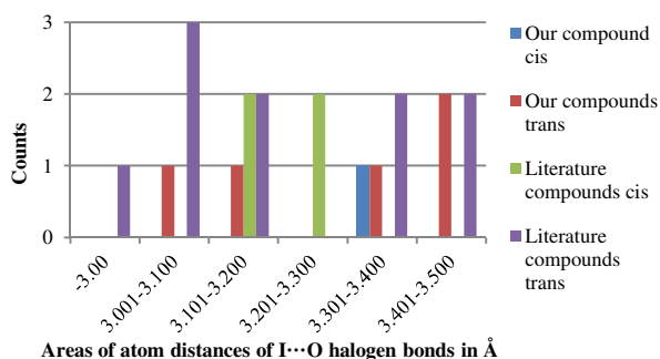
Figure 9 Statistical distribution of the intermolecular I...O halogen bond lengths of all diiodides discussed here, separated in cis/trans and literature compounds and ours. The maximum distance is the sum of the van der Waals radii of the involved atoms (3.50 Å).
