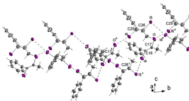
Figure 21 Helical double strand chains along the b -axis in the crystal structure of 2 , formed by I...I halogen bonds. Symmetry codes: a (x, 1+y, z), b (x, -1+y, z), c (-x, -0.5+y, 0.5-z), d (-x, 0.5+y, 0.5-z), e (1+x, y, -1+z). DIAMOND representation, thermal ellipsoids are drawn at 50 % probability level.
