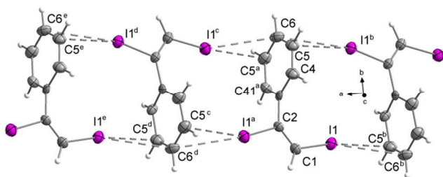
Figure 19 Crystal structure of compound 3 . View of the chains along the a -axis resulting from intermolecular I...C( \pi ) interactions. Symmetry codes: a (1-x, y, 1.5-z), b (0.5-x, 0.5-y, 2-z), c (0.5+x, 0.5-y, -0.5+z), d (1.5-x, 0.5-y, 1-z), e (1+x, y, -1+z). DIAMOND representation, thermal ellipsoids are drawn at 50 % probability level.
