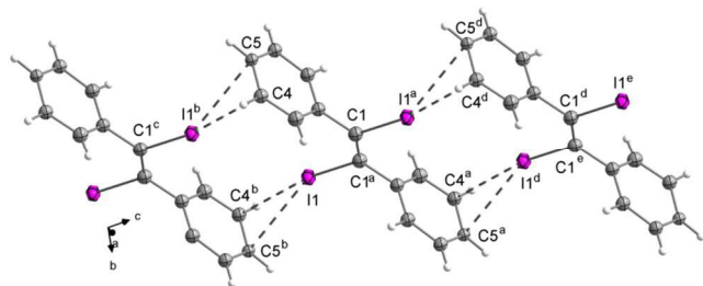
Figure 23 I...C( \pi ) Halogen bonds in the crystal structure of 1 forming chains. Symmetry codes: a (1-x, 1-y, 2-z), b (-x, 1-y, 1-z), c (-1+x, y, -1+z), d (1+x, y, 1+z), e (2-x, 1-y, 3-z). DIAMOND representation, thermal ellipsoids are drawn at 50 % probability level.
