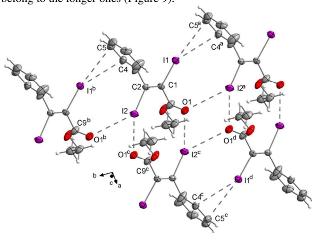
Figure 16 Chains along the b -axis in the crystal structure of the ethylester 6 . Symmetry codes: a ( x, -1+y, z ), b ( x, 1+y, z ), c ( 1-x, 2-y, 1-z ), d ( 1-x, 1-y, 1-z ). DIAMOND representation, thermal ellipsoids are drawn at 50% probability level.
