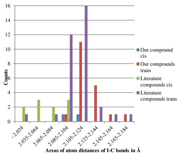
Figure 8 Statistical distribution of the C-I atom distances of all diiodides discussed here, separated in cis/trans and literature compounds and ours. C 2 I 2 18 was excluded because of the very short C-I distance (1.987(3) Å), F 3 Cl 19 and C 2 I 2 20 are included in the literature trans category. Cis diiodo compounds, which are mostly cyclic, have shorter C-I atom distances than linear ones and those with trans configuration. They are even shorter than the literature value given for the C N -I distance (2.095 Å) 21 .
