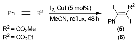
Figure 2 Synthetic pathway of the new 1,2-diiodoolefinic esters 5 and 6 .
