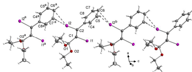
Figure 18 Crystal structure of compound 7b . View of the chains along the c -axis resulting from intermolecular I\cdots C(\pi) interactions. Symmetry codes: a ( x, 0.5-y, -0.5+z ), b ( x, 0.5-y, 0.5+z ). DIAMOND representation, thermal ellipsoids are drawn at 50% probability level.
