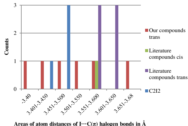
Figure 14 Statistical distribution of the intermolecular I...C( \pi ) halogen bond lengths in Å
