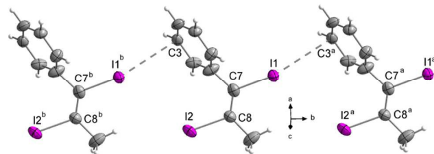
Figure 20 I...C( \pi ) Halogen bonds in the crystal structure of 4 forming chains in b -direction. Symmetry codes: a (x, 1+y, z), b (x, -1+y, z). DIAMOND representation, thermal ellipsoids are drawn at 50 % probability level.
