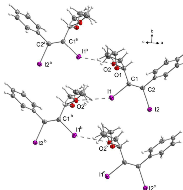
Figure 17 Zigzag chains governed by short intermolecular I\cdots O contacts in the b -axis direction, in the crystal structure of compound 7a . Symmetry codes: a (0.5– x , 0.5+ y , 1.5– z ), b (0.5– x , –0.5+ y , 1.5– z ), c ( x , –1+ y , z ). DIAMOND representation, thermal ellipsoids are drawn at 50% probability level.
