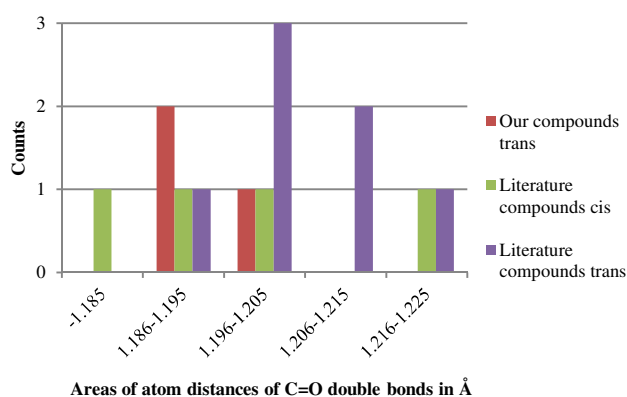
Figure 5 Statistical distribution of the C=O atom distances of all diiodides discussed here, separated in cis/trans and literature compounds and ours. The trend goes to longer bonds compared to the literature value of 1.19 Å 22 . The reference of Allen et al. 21 (1.199 Å) is more appropriate.
