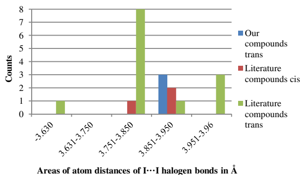
Figure 10 Statistical distribution of the intermolecular I...I halogen bond lengths of all diiodides discussed here, separated in cis/trans and literature compounds and ours. The maximum distance is the sum of the van der Waals radii of the involved atoms (3.96 Å).
