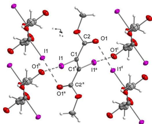
Figure 7 Network in the crystal structure of the diester 8 . Symmetry codes: a (2-x, -y, 1-z), b (x, 0.5-y, 0.5+z), c (2-x, -0.5+y, 0.5-z), d (x, 0.5-y, -0.5+z). DIAMOND representation, thermal ellipsoids are drawn at 50% probability level.
