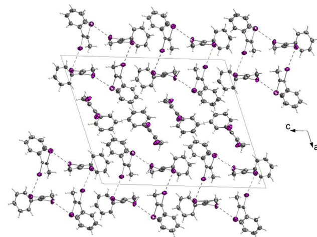
Figure 22 The helices form quad shaped subunits which form strands along the c -axis in the crystal structure of 2 . The molecules that form I...C( \pi ) halogen bonds are between the strands of quad shaped units. DIAMOND representation, thermal ellipsoids are drawn at 50 % probability level.
