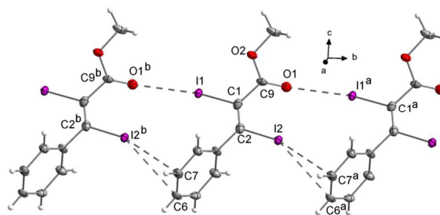
Figure 15 Chains along the b -axis in the crystal structure of the methylester 5 . Symmetry codes: a ( x , 1+ y , z ), b ( x , -1+ y , z ). DIAMOND representation, thermal ellipsoids are drawn at 50% probability level.
