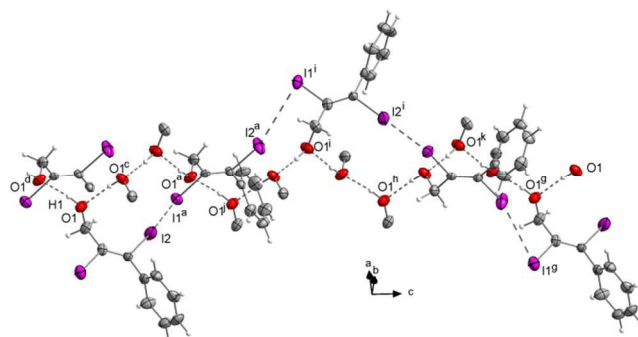
Figure 11 Crystal structure of 4. One turn of the helix formed by the I...I halogen bonds (I2 to I1 g ) includes three turns of the helix formed via hydrogen bonds (O1 to O1 l ; O1 l to O1 h ; O1 h to O1 g ) d(O-H) = 0.84(2) Å, d(O1 \cdots O1^h) = 2.693(3) Å, \angle O1-H1 \cdots O1^h = 169.6(2)^\circ . Some (I)C=C(I)Ph residues are omitted for clarity. Symmetry codes: a (-0.25+x, 1.25-y, 0.75+z), c (1.25-x, 0.25+y, 0.25+z), g (x, y, 3+z), h (x, y, 2+z), i (1.5-x, 1-y, 1.5+z), j (x, y, 1+z), k (1.5-x, 1-y, 2.5+z). DIAMOND representation, thermal ellipsoids are drawn at 50% probability level.
