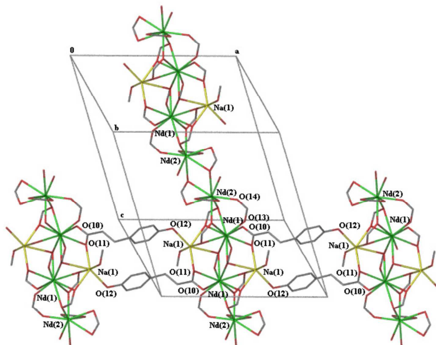
Figure 3: The propagation of the 2D polymeric network of [\text{NaND}_2(4\text{hpp})_7(\text{H}_2\text{O})(\text{MeOH})] \cdot (\text{H}_2\text{O}) \cdot 3(\text{MeOH}) ( 4 ) showing the bridging of the phenolic oxygen atom to the sodium metal centre from a neighbouring chain. Non-metal atoms except those immediately surrounding the metal centres are omitted for clarity.
