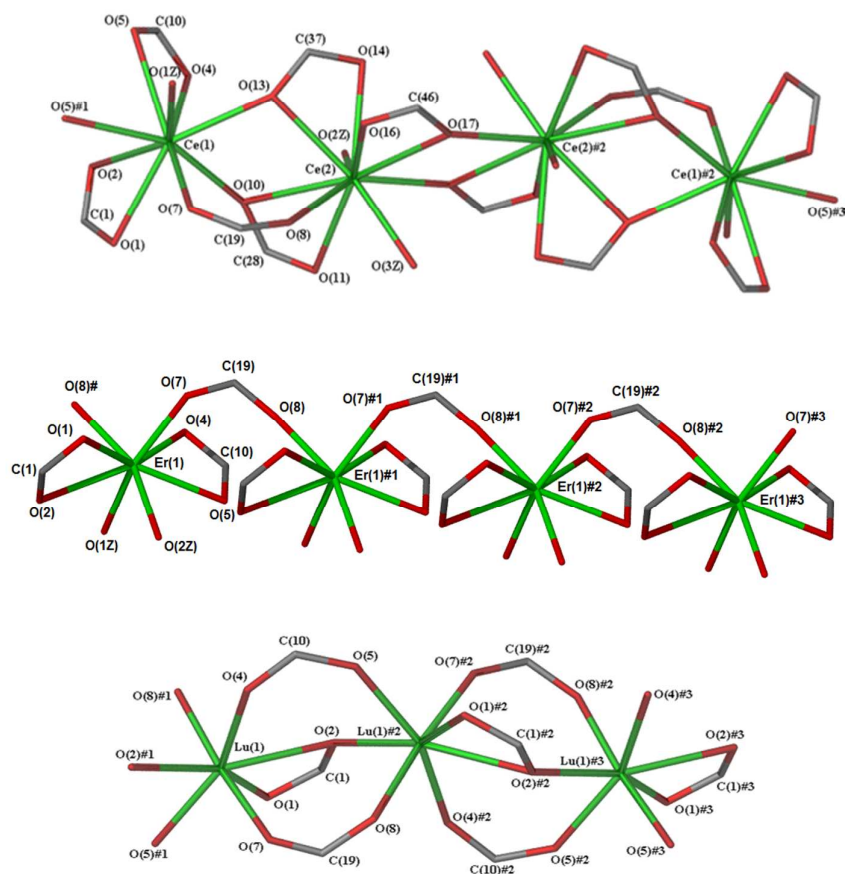
Figure 2: The propagation of the 1D polymeric chains of [\text{La}_4(4\text{hpp})_{12}(\text{H}_2\text{O})_6] \cdot 4(\text{H}_2\text{O}) ( 1 ) and [\text{Ce}_2(4\text{hpp})_6(\text{H}_2\text{O})_3] \cdot 2.5(\text{EtOH}) \cdot (\text{H}_2\text{O}) ( 2a ), [\text{Er}(4\text{hpp})_3(\text{H}_2\text{O})_2] \cdot 1.5(\text{H}_2\text{O}) ( 6 ) and [\text{Lu}(4\text{hpp})_3] \cdot (\text{H}_2\text{O}) ( 7 ). Symmetry equivalents used: complex 1 (#1 x, y-1, z ; #2 x, 1+y, z ), complex 2a (#1 1-x, -y, 1-z ; #2 1-x, 1-y, 1-z ; #3 x, 1+y, z ), complex 6 (# x, 1+x, z ; #1 x-1/2, 1/2-y, z ; #2 1/2-x, 1/2+y, z-1/2 ), and complex 7 (#1 1-x, 1/2+y, 3/2-z ; #2 1-x, y-1/2, 3/2-z ; #3 x, y-1, z ).
