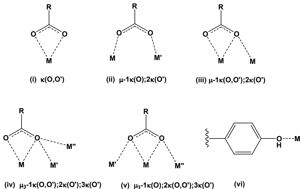
Figure 1: Different coordination modes observed by the 3-(4'-hydroxyphenyl)propionate ion.
