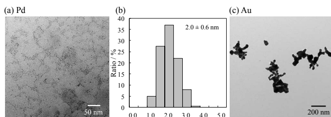
Fig. 4 (a) TEM image of Pd NPs, (b) size distribution histogram of Pd NPs, and (c) TEM image of Au NPs. Pd and Au NPs were prepared at a 1:3 mol ratio of metal:acetylthiocholine (ATC).
