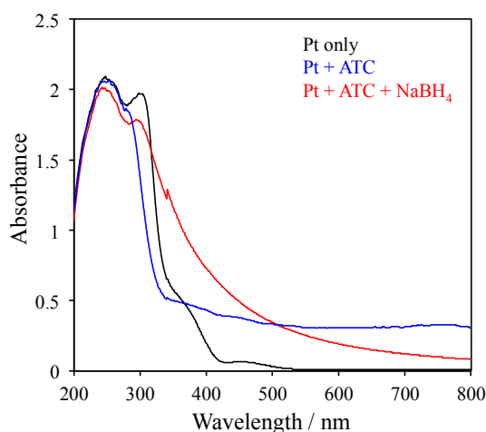
Fig. 1 Absorption spectra of (a) \text{H}_2\text{PtCl}_4 solution in methanol, (b) after the addition of an acetylthiocholine (ATC) aqueous solution to a, (c) after addition of the \text{NaBH}_4 aqueous solution to b. All measurements were performed using a 1 mm quartz cell without dilution.
