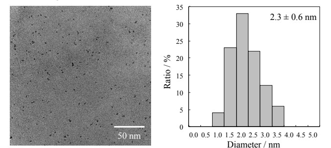
Fig. 2 TEM images and size distribution histogram of Pt nanoparticles prepared at a 1:3 mol ratio of Pt:acetylthiocholine (ATC).
