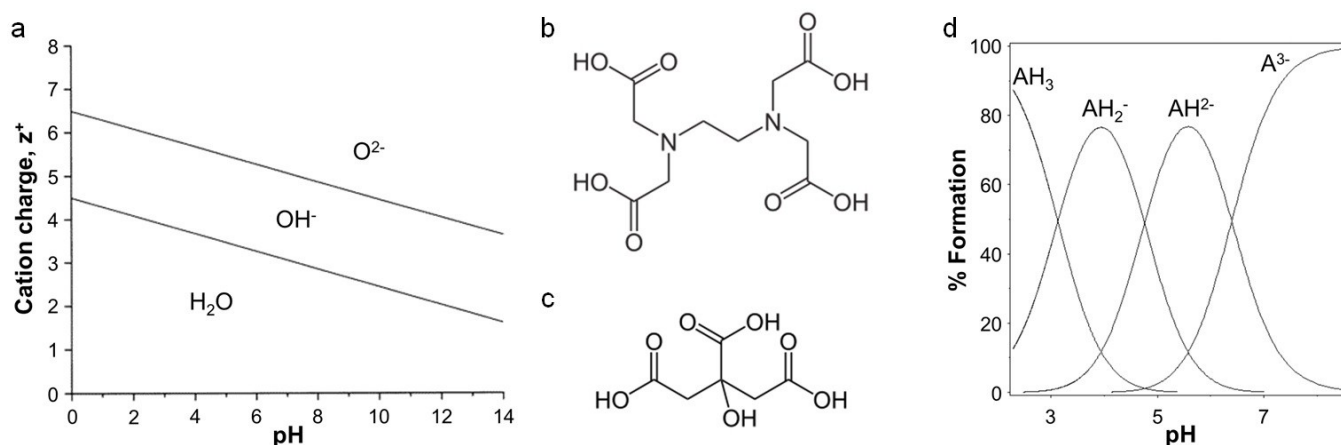
Figure 3 a) Relationship between charge, pH, and hydrolysis equilibrium of cations, modified with permission from reference 2. Structures of b) EDTA and c) citric acid. d) Ion speciation graph for citric acid plotted using the program HSS.
