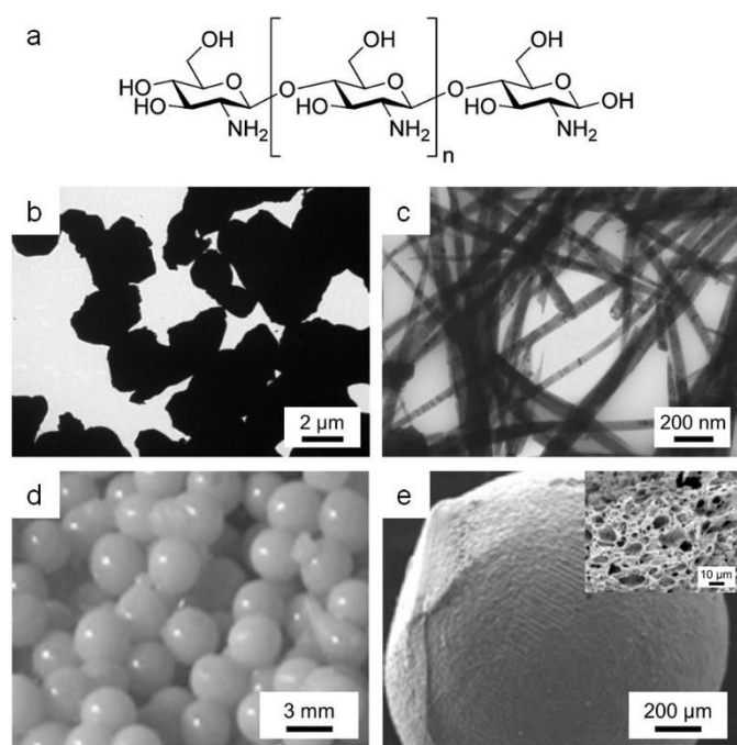
Figure 12 a) Structure of chitosan. TEM images of samples of \text{YBa}_2\text{Cu}_4\text{O}_8 synthesized using b) acetate/tartrate and c) chitosan. d) Photograph and e) SEM image of chitosan beads prepared by crosslinking with \text{Ce}^{3+} with (inset) SEM image of sponge-like structure formed after calcination of the beads. Images reproduced with permission from references 11 (b,c) and 109 (d,e).
