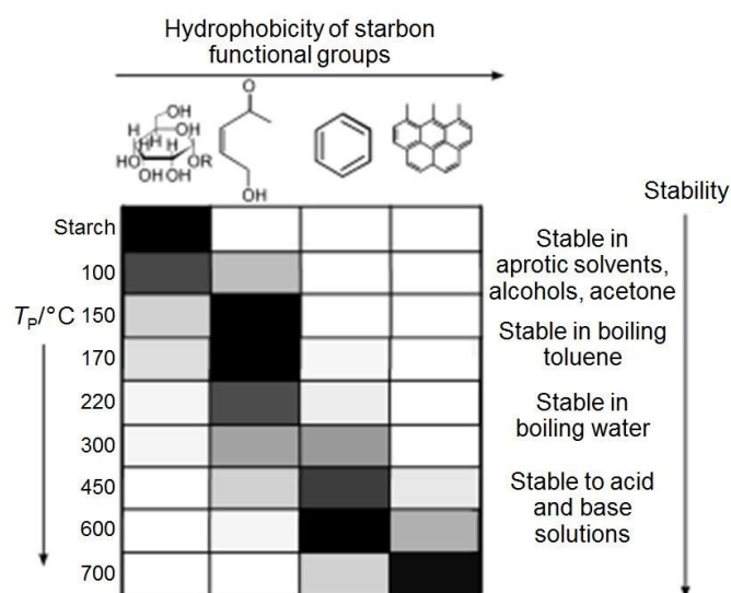
Figure 10 Distribution of functional groups on starch-derived carbons prepared at different temperatures (grey scale to indicate relative amounts where black is highest). Modified with permission from reference 95.
