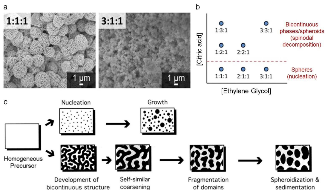
Figure 7 a) SEM images of samples prepared at two EG:CA:TMI (ethylene glycol to citric acid to total metal ion) ratios, b) schematic showing how EG:CA:TMI ratio affects structure and c) schematic of nucleation and spinodal decomposition mechanisms. Modified with permission from reference 78. Copyright (2012) ACS.
