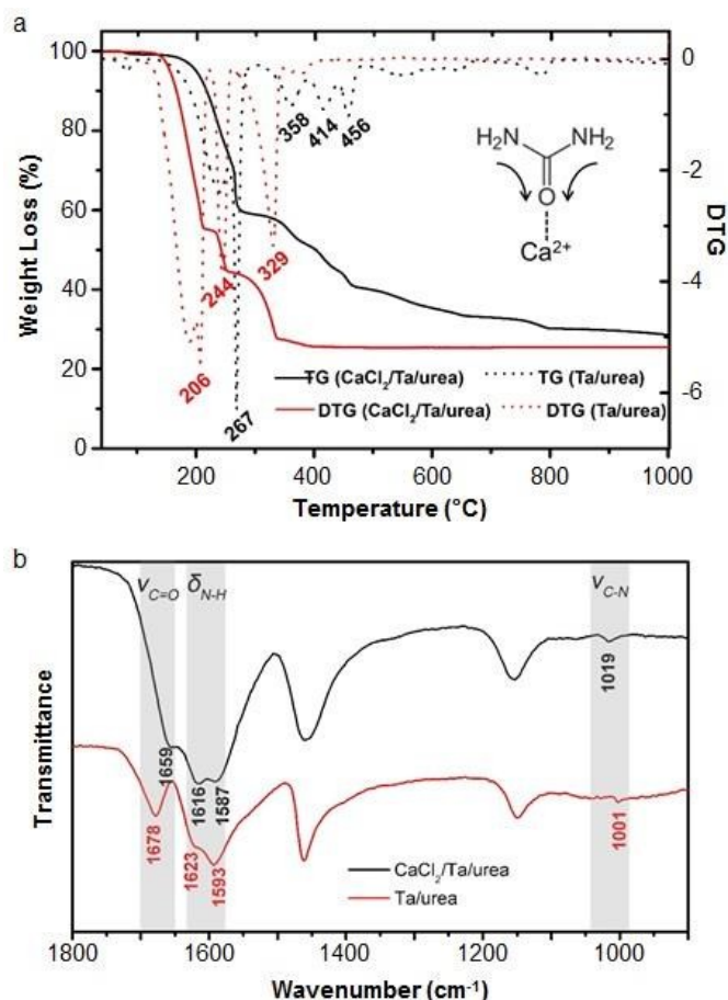
Figure 5 a) TGA/DTG of tantalum/urea mixtures both with (black) and without (red) calcium showing the later onset of decomposition with calcium. b) IR spectra of the same samples showing a shift and reduction in intensity of the C=O stretch of urea when calcium is added. Modified with permission from reference 70.
