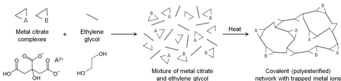
Figure 6 Schematic of the Pechini method of making metal/organic gels
