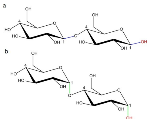
Figure 9 a) Alpha and b) beta glycosidic linkages.
