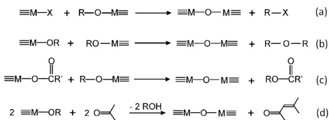
Scheme 6 Condensation steps in non-hydrolytic sol-gel chemistry including a) alkyl halide elimination, b) ether elimination, c) ester elimination and d) aldol-like condensation. Modified with permission from reference 133.
