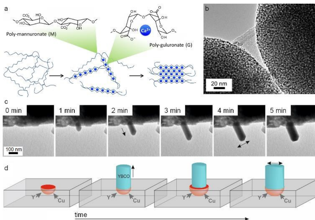
Figure 13 a) Egg-box model of cation binding in alginate. TEM images of b) YBCO nanowires synthesized from alginate with acetate/tartrate precursors with (inset) \text{BaCO}_3 nanoparticles that act as sites for catalytic float outgrowth. TEM images of c) straight nanowires growing from a precursor of alginate with metal nitrates with d) schematic showing nanowire spontaneously broadening as a result of microcrucible creep and expansion during heating. Images modified with permission from references 91 and 114 (c/d). Image (b) reproduced with permission from reference 111. Copyright (2013) American Chemical Society.
