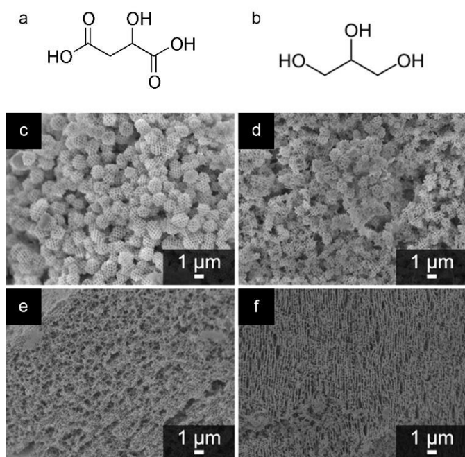
Figure 8 Structures of a) malic acid and b) glycerine. SEM images of samples of \text{Ce}_{0.5}\text{Mg}_{0.5}\text{O}_{1.5} prepared at a 2:1:1 molar ratio of EG:CA:TMI (ethylene glycol to citric acid to total metal ions) in a PMMA opal template showing c) no reagent substitutions, (d) substitution of glycerine for EG, (e) substitution of malic acid for CA, and (f) substitution of both glycerine and malic acid for EG and CA, respectively (c-f modified with permission from reference 81). Copyright (2015) American Chemical Society.
