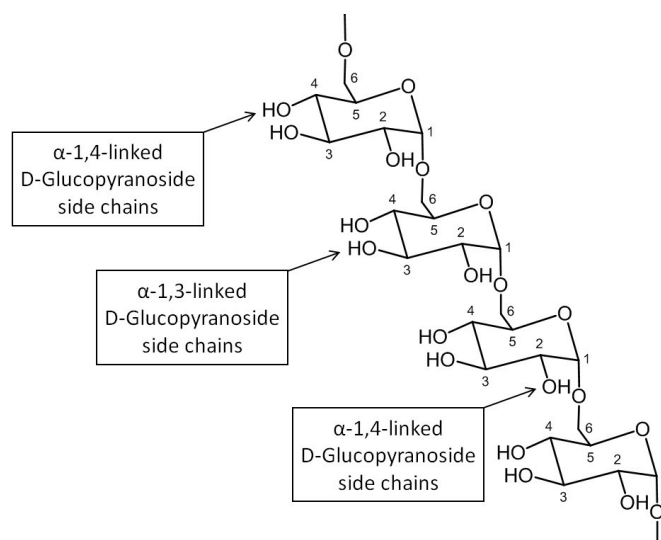
Figure 11 Structure of Dextran showing the different glycosidic bonds.
