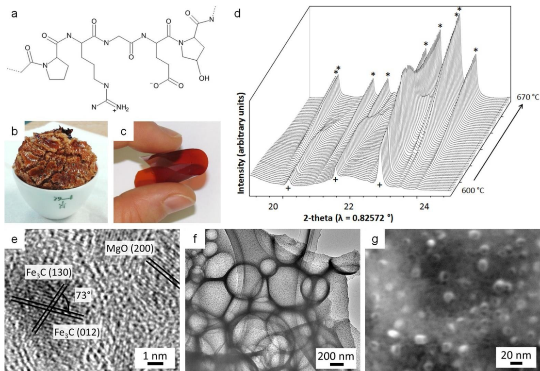
Figure 14 a) Typical structure of a gelatin fragment. Images of b) foam from gelatin and iron nitrate and c) film from gelatin and iron acetate. d) Synchrotron powder X-ray diffraction data showing the iron nitride (+) to carbide (*) transition during a sol-gel synthesis from gelatin. e) TEM image of a \text{Fe}_3\text{C}/\text{MgO}/\text{C} composite showing two types of nanoparticles. TEM (f) and SEM (g) images of a \text{Fe}_3\text{C}/\text{MgO}/\text{C} composite after acid washing showing macropores and mesopores. Images reproduced with permission from references 121 (c) and 123 (d). Copyright (2010) and (2015) American Chemical society. Images (e-g) modified with permission from reference 125.
