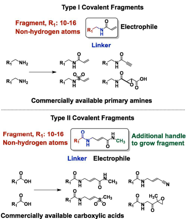
Figure 6. Proposed design of covalent fragments. Type I covalent fragments are made from non-aromatic amines (~4000 commercially available) and contain the fragment part R 1 (10-16 non-hydrogen atoms), a linker, and the electrophile. R 1 is separated from the amino group with methylene as a linker to avoid the conjugation of the nitrogen lone pair to the fragment. This ensures that these types of acrylamides will have similar reactivity toward thiols. Type II covalent fragments are based on carboxylic acids (~92,000 commercially available) that are converted into covalent fragments. Type II fragments satisfy all 5 criteria and are therefore ideally suited for covalent tethering. In both cases FDA approved covalent drugs and reactive natural products can serve as inspiration and a guide to select electrophiles for covalent fragment library design.
