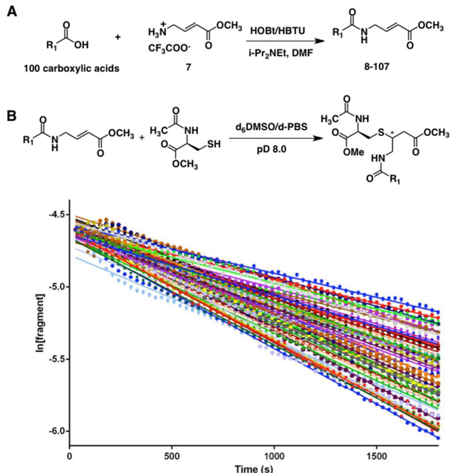
Figure 5. (A) Design and synthesis of the fragment library. Electrophile 7 can be prepared on a 10g scale. (B). Pseudo-first order NMR rate plots of the reaction of 50 compounds with N -acetyl cysteine methyl ester. Different colors represent different fragments. Reproduced from ref. 12.
