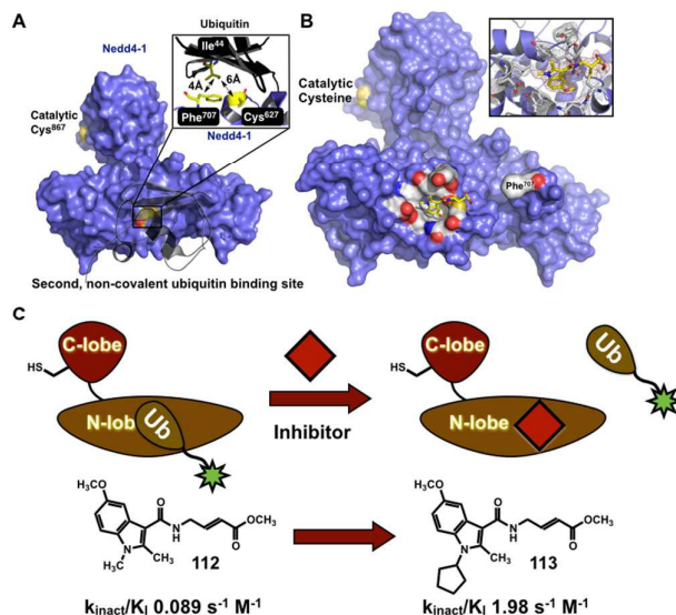
Figure 9. Covalent fragments as PPI inhibitors. A) Co-crystal structure of Nedd4-1 catalytic HECT domain with ubiquitin. Phe 707 of Nedd4-1 forms critical hydrophobic interactions with Ile 44 of ubiquitin. Mutation of Phe 707 of Nedd4-1 into alanine increases the K_d from ~11 \mu\text{M} to 340 \mu\text{M} . Therefore Phe 707 and Ile 44 represent a classic protein-protein interaction hot spot. In addition, Tyr 605 of Nedd4-1 also forms critical binding interactions with Leu 73 of Ub. B) Crystal structure of the indole 112 bound to the catalytic HECT domain of Nedd4-1 showing that compound 112 actually blocks Tyr 605 of Nedd4-1 from interacting with Ub. C) The potency of compound 112 and its analogue 113 were investigated in fluorescence polarization assays to obtain k_{\text{inact}}/K_i values.
