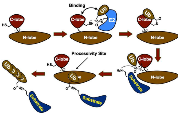
Figure 8. Simplified model of HECT E3 mediated protein ubiquitination. E2~Ub thioester binds the catalytic HECT domain, followed by a transthiolation reaction, producing HECT E3~Ub thioester. Subsequently, HECT E3~Ub ligates Ub onto the lysine of the substrate, followed by polyubiquitin chain growth. The C- and N-lobes of the HECT domain rotate relative to each other during the catalytic cycle.
