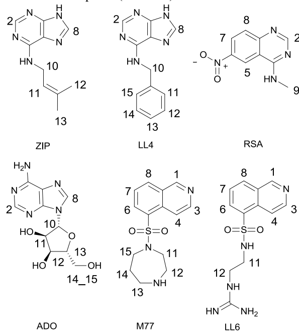
Fig. 1 Cdk-2 inhibitors used for the INPHARMA analysis. K_d values were measured by isothermal titration calorimetry and are: LL4, 62 \mu\text{M} ; ZIP, 35 \mu\text{M} ; RSA, 208 \mu\text{M} ; ADO, 184 \mu\text{M} ; M77, 460 \mu\text{M} ; LL6, 286 \mu\text{M} .
