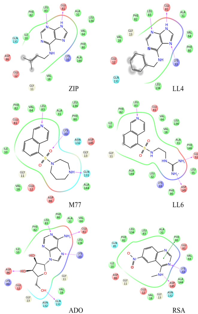
Fig. 3 Schematic representation of the protein-ligand interactions for all analyzed compounds. We show all binding interactions observed in the binding poses selected by INPHARMA-STRING in the 5% top-ranked binding modes. The binding site residues within 4 Å from the ligand are indicated as spheres, while hydrogen bonds are represented by red arrows. Blue, hydrogen bond donor; red, hydrogen bond acceptor; green, hydrophobic interaction.
