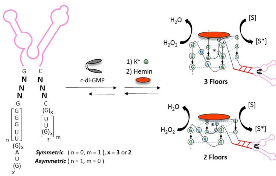
Figure 1: A cyclic dinucleotide riboswitch, Vc2 RNA, 32-34 fused to a G-quadruplex.
