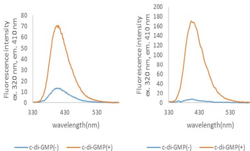
Figure 5: Peroxidase reaction of tyramine using ST2Sym riboswitch-G4 fused RNA [3 floors G-tetrads (Left) and 2 floors G-tetrads (Right)] in the presence or absence of c-di-GMP. Conditions: same as Figure 4. Fluorescence intensities at 410 nm in the absence and presence of c-di-GMP are 13.1 and 70.9 respectively for 3 floors G-tetrads, 6.8 and 177.4 respectively for 2 floors G-tetrads.
