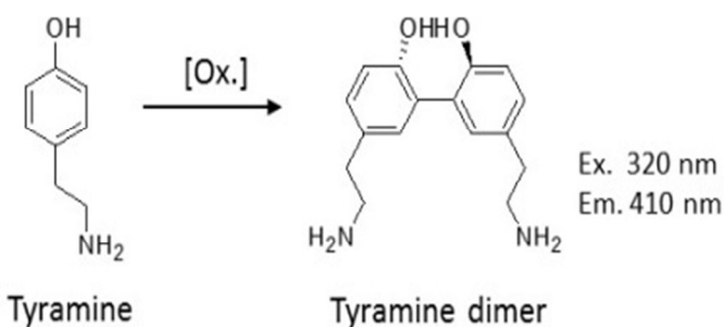
Figure 3: Oxidation of tyramine to tyramine dimer
