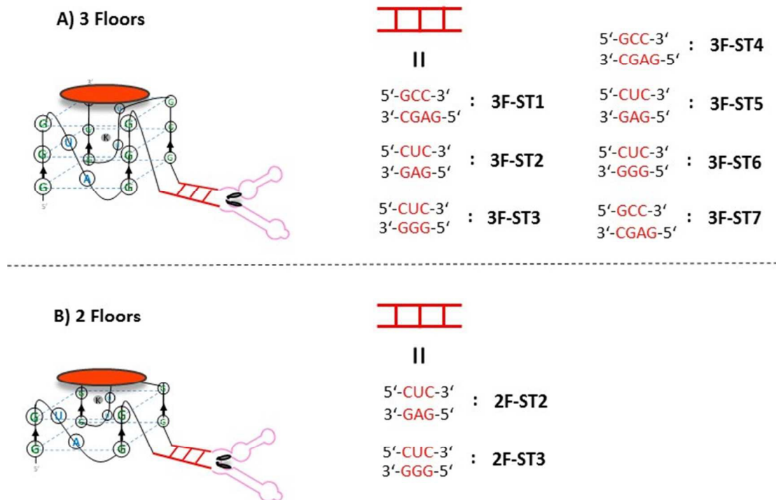
Figure 2: Asymmetric and symmetric riboswitch-G4 fusions used for this study (see supplementary information for the detailed sequences.). A) riboswitch-G4 fused RNA with three G-tetrad floors complexed to hemin; B) riboswitch-G4 fused RNA with two G-tetrad floors complexed to hemin.
