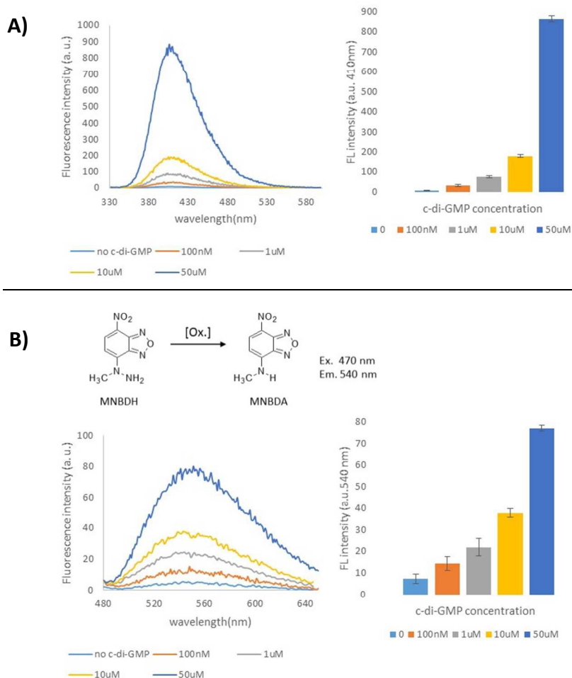
Figure 6: C-di-GMP concentration-response fluorescence intensity in peroxidase reaction.
