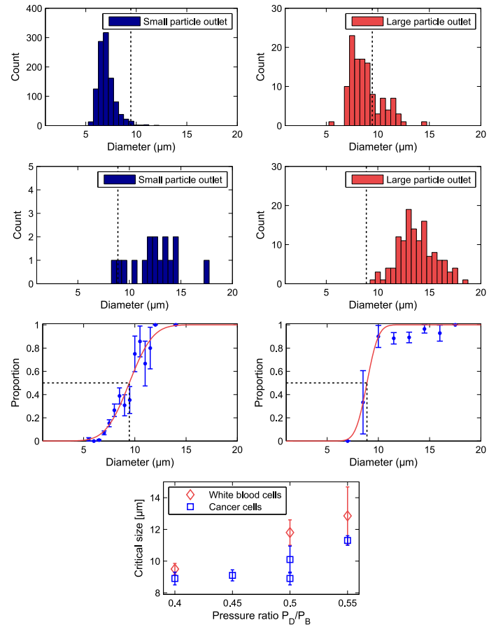
Fig. 4 Separation of WBCs and LS174T cells in a PFF device with a fixed critical diameter at 10 \mu\text{L/h} . (A-B) Size distribution of WBCs in each outlet after separation. (C-D) Size distribution of cancer cells in each outlet after separation. (E) Proportion of WBCs in the large particle outlet. The critical diameter is marked by black dashed lines and reads 9.5 \pm 0.35 \mu\text{m} . (F) Proportion of cancer cells in the large particle outlet. The critical diameter is marked by black dashed lines and reads 8.9 \pm 0.4 \mu\text{m} . The recovery was 91.4% for cancer cells with a removal of 89.7% WBCs. (G) Measured critical diameter of cancer cells and WBCs vs. the pressure ratio between the buffer inlet and the drain.
