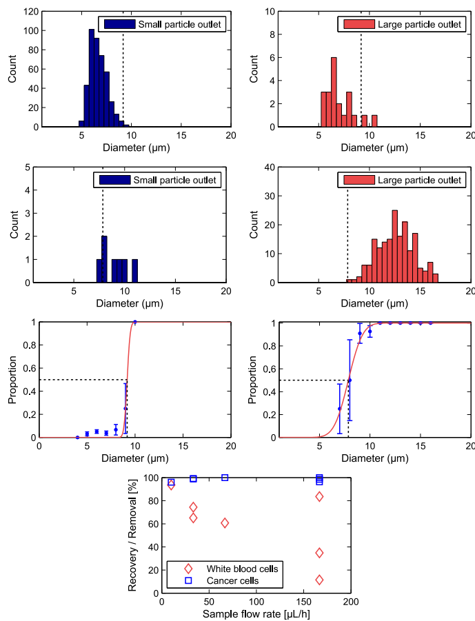
Fig. 3 Separation of WBCs and LS174T cells in a PFF device with a fixed critical diameter at 10 \mu\text{L/h} . (A-B) Size distribution of WBCs in each outlet after separation. (C-D) Size distribution of cancer cells in each outlet after separation. (E) Proportion of WBCs in the large particle outlet. The critical diameter is marked by black dashed lines and reads 9.2 \pm 2.1 \mu\text{m} . (F) Proportion of cancer cells in the large particle outlet. The critical diameter is marked by black dashed lines and reads 7.9 \pm 0.15 \mu\text{m} . The recovery was 96.0% for cancer cells with a 93.6% removal of WBCs. (G) Recovery of cancer cells and removal of WBCs at different sample flow rates.
