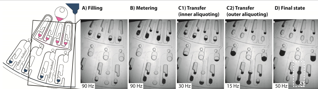
Fig. 4 Experiment showing principle of centrifugo-pneumatic multi-liquid aliquoting with stained sample material. Every second collection chamber is combined with a quantification structure (a) for measurement of aliquoted volumes. The quantification structure is described in detail in Fig. 5.
