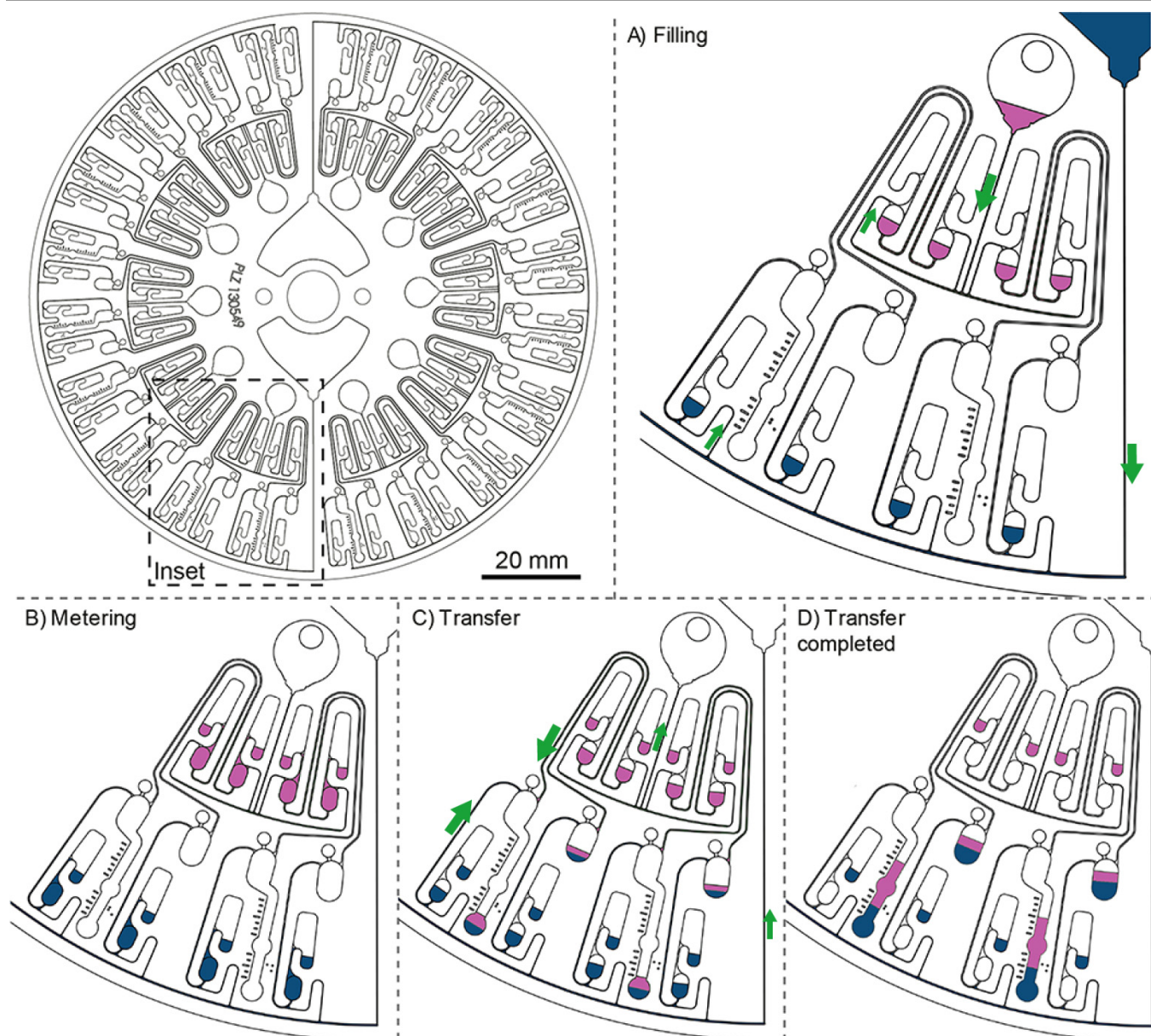
Fig. 3 Microfluidic disk with 10 inner aliquoting structures and two outer aliquoting structures with twenty aliquots each and ten inner aliquoting structures with four aliquots each. The fluidic operation of the inner and outer aliquoting is described step by step for the marked inset. The fluidic principle of the inner and outer aliquoting is described in detail in Fig. 2. Green arrows indicate liquid flow at selected locations. A detailed description of the implemented channels and chambers is given in ESI Fig. 3. An experimental run of the implemented design using colored dye can be seen in Fig. 4.
