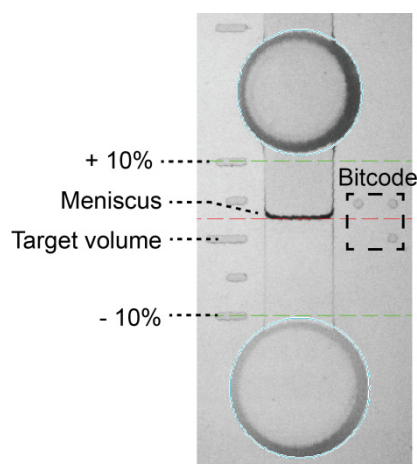
Fig. 5 Quantification structure for metering of individual aliquots. The structure consists of an upper and lower circular chamber, connected by a channel. The lower chamber has a volume of 4.5 \mu l and the channel has a total volume of 1 \mu l. For a filling volume of 5 \mu l the meniscus is positioned at the center between the circular chambers. The circular chambers and the position of the meniscus (red line) are detected by an automated Matlab algorithm. The aliquoted volume can then be calculated from the meniscus position within the channel with a precision of 20 nl. Each aliquot is identified via an individual barcode number.
