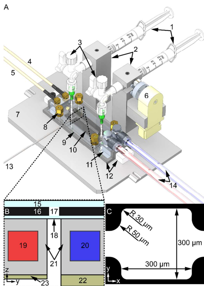
Figure 1: Overview of the device for temperature-controlled acoustophoresis with pressure calibration. (A) The different parts of the device: (1) 3 ml plastic syringes with luer lock for injecting and subtracting samples. (2) Aluminum syringe holders with set screws to secure the syringes. (3) 4-way luer lock stopcock with stainless steel dispensing tip and silicon and Tygon tubing connected to the microfluidic chip. (4-5) BNC to MCX cables and connectors for the trapping and levitating ultrasonic-piezo-actuators, respectively. (6) Motorized magnet stirrer with PTFE magnetic stirrer bar inside injection syringe to prevent sedimentation. (7) Aluminum base plate compatible with Zeiss Axiovert 40 microscope xy-stage. (8) Nuts, compression springs, and spacers, four in each corner of the PMMA manifold (9), to secure a good coupling between microfluidic chip and the ultrasonic-transducers. The manifold has passages for flow connectors and bright-light (optimized for trans-illumination microscopy). (10) Microfluidic chip with micro-cages. (11) Aluminum matching layer with water channels. (12) ABS plastic cover to protect the piezo-transducers mounted on the bottom of (11). (13) Two thermocouple probes to monitor (PID controller) and register (data logger) the temperature of the microfluidic chip (10). (14) Inlet and outlet water tubing connected to the temperature controller's liquid loop for active temperature regulation. (B) Cross section view of the device: (15-18) Different parts of the microfluidic chip were: (15) is the top glass layer, (16) the silicon layer with etched channels and micro-cages (17) and (18) the bottom glass layer, (19-20) water channels machined in (21) the aluminum housing (red and blue indicates the flow of water: blue in and red out), (22) trapping piezo-actuator (resonance frequency 2.52 \pm 0.02 MHz, Q-factor 9 \pm 0.004 ), (23) levitation piezo-actuator (resonance frequency 7.62 \pm 0.054 MHz, Q-factor 32 \pm 0.1 ). (C) Top-view of the micro-box-cage with inlet and outlet channel. The internal height of the microfluidic chip is 110 \mu\text{m} .
