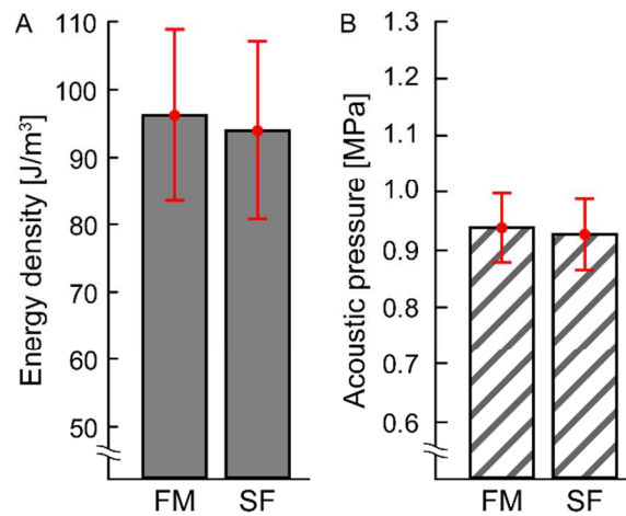
Figure 2: (A) Energy density and (B) acoustic pressure amplitude inside the trapping chamber measured with the light-intensity method 16 for frequency-modulation (FM) and single frequency (SF) actuation. The respective mean values with corresponding standard deviations ( \pm\sigma ) are shown in red. For FM actuation the average energy density and acoustic pressure are 96.3\pm 12.8 J/m 3 and 0.94\pm 0.06 MPa, respectively. For SF actuation the average energy density and acoustic pressure are 94.2\pm 13.2 J/m 3 and 0.93\pm 0.06 MPa, respectively. The temperature was actively regulated during both measurements ( 36.4\pm 0.2^\circ\text{C} ).
