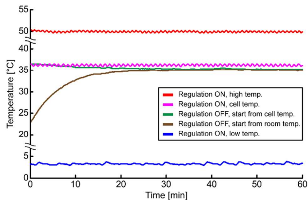
Figure 3: Demonstration of temperature control at different regulation schemes measured over a period of one hour with continuous ultrasound (frequency modulation, center frequency 2.53 MHz, span 100 kHz, rate 1 kHz, actuation voltage comparable to an acoustic pressure of 0.94 MPa). The device is tested at both low ( 3.2 \pm 0.2^\circ\text{C} , blue curve) and high ( 50 \pm 0.2^\circ\text{C} , red curve) temperatures with active temperature regulation. To ensure high cell viability the device was set to regulate a temperature < 37^\circ\text{C} , in this demonstration the “cell” temperature was 36.2 \pm 0.2^\circ\text{C} (magenta colored curve). In addition, as a control, the device was operated without active temperature regulation from room temperature (brown curve) and from “cell” temperature (green curve). As a consequence of the design of the device, the final temperature after one hour was 35.1 \pm 0.1^\circ\text{C} for the brown and green colored curves.
