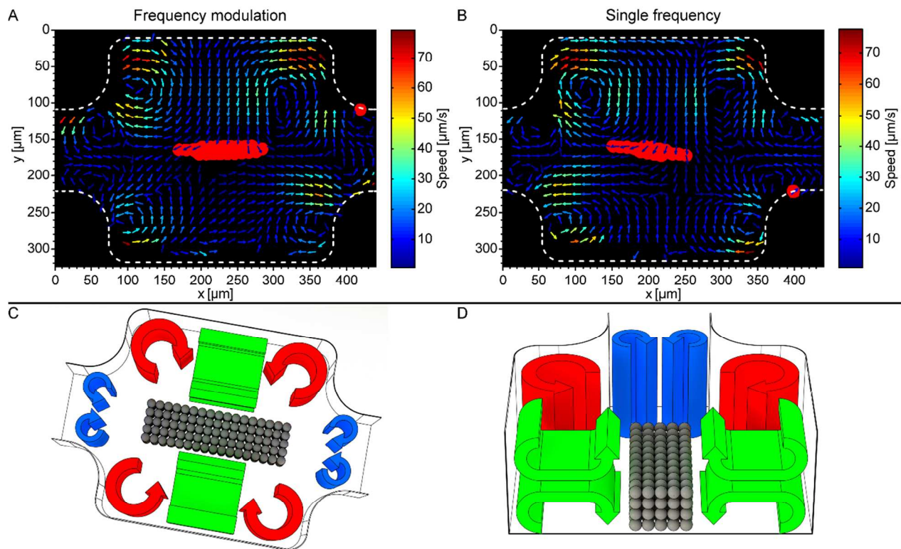
Figure 5: Quantitative (A-B) and qualitative (C-D) description of the acoustic streaming in the micro-box-cage. (A): Micro-particle-image-velocimetry ( \mu PIV) of the acoustic streaming when implementing frequency-modulated (FM) ultrasound (2.53 MHz, span 0.1 MHz, and a rate of 1 kHz, acoustic pressure amplitude 0.87 \pm 0.02 MPa). (B): \mu PIV of the acoustic streaming at single frequency (SF) ultrasound (2.53 MHz and acoustic pressure amplitude 0.87 \pm 0.02 MPa). The red colored regions in (A) and (B) indicates where the larger 10 \mu\text{m} beads are trapped. (C): Sketch of the three different types of acoustic streaming in the trapping chamber: Standard Rayleigh boundary streaming (red), smaller Rayleigh streaming located at the transitions to the inlet and outlet channel of the chamber (blue), and finally vertical Rayleigh streaming (green). The qualitative description of the acoustic streaming is verified in supplementary video S1. (D): Cross section view of (C) giving a more detailed view of the vertical streaming vortices (green). The gray colored spheres in (C) and (D) represent a trapped particle aggregate.
