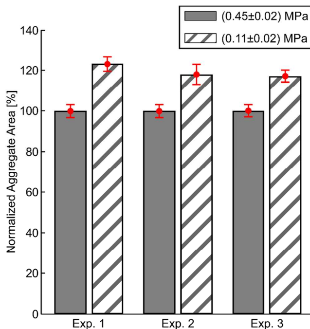
Figure 4: Area of the imaged trapped particle aggregates in the trapping chamber measured for two different acoustic pressure amplitudes. The solid grey colored bars show the aggregate size at the pressure amplitude (0.45 \pm 0.02) MPa and the striped white-and-grey colored bars show the aggregate size at the pressure amplitude (0.11 \pm 0.02) MPa for the three different experiments. The respective normalized aggregate area mean values with corresponding standard deviations ( \pm\sigma ) is shown in red for the three experiments: Exp. 1 ( 100\% \pm 3.6\% and 123\% \pm 3.9\% ), Exp. 2 ( 100\% \pm 3.5\% and 118\% \pm 5.4\% ), and Exp. 3 ( 100\% \pm 3.2\% and 117\% \pm 3.2\% ), for the two pressure amplitudes (0.45 MPa and 0.11 MPa), respectively. The temperature was actively regulated during the three experiments: Exp. 1 ( 36.0 \pm 0.2^\circ\text{C} and 35.8 \pm 0.2^\circ\text{C} ), Exp. 2 ( 36.1 \pm 0.2^\circ\text{C} and 35.8 \pm 0.2^\circ\text{C} ), and Exp. 3 ( 36.1 \pm 0.2^\circ\text{C} and 35.7 \pm 0.2^\circ\text{C} ), for the two pressure amplitudes (0.45 MPa and 0.11 MPa), respectively.
