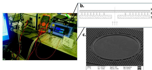
Fig. 2. a) Blister burst pressure test setup. b) Schematic view of the (R)igid backing-(B)lister-(S)ubstrate arrangement c) SEM of the blister that was tested. (© CBMS 33 )
