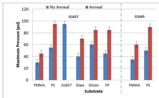
Fig. 4. The maximum pressure endurance for Kraton G1657 and Kraton G1645 blisters bonded to different substrates.
