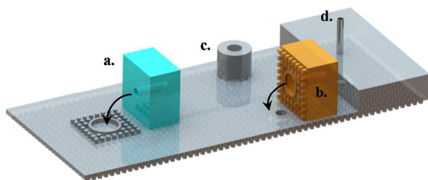
Fig. 5. Possible world to chip configurations for this technology: A simple capillary electrophoresis design with a) patterned blister to facilitate interfacing with external ports b) patterned port to interface with the device c) Modified rigid backing with integrated connectors d) New England pin embedded in a thick elastomer layer. (also see Fig S3. in ESI.†)
