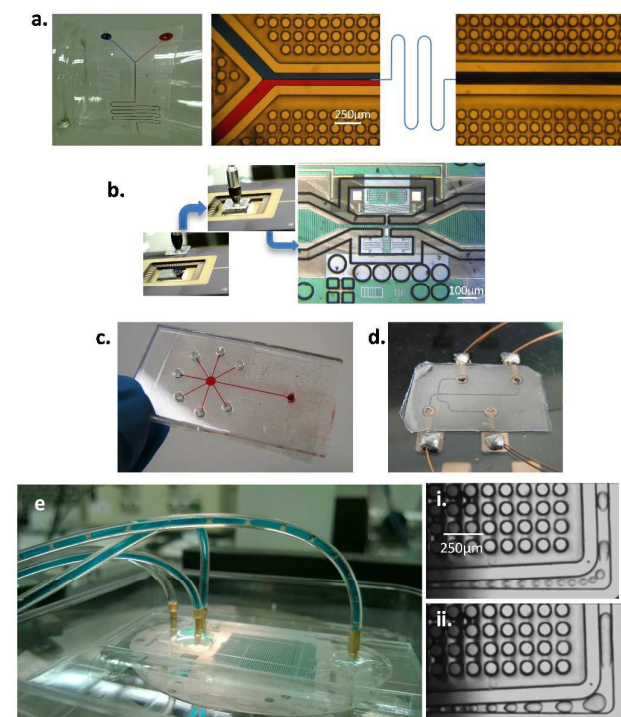
Fig. 3. Gecko-inspired-adhesives integrated microfluidic device on various substrates , a) Micromixer on glass erlenmeyer flask with red and blue food dye, b) Microfluidic channel network for MEMS cell gripper showing integrated thermal actuators, springs and dielectrophoretic pumps (Images courtesy of Dr. Stephan Warnat, Dalhousie University) c) Microfluidic distributor on laser cut PMMA substrate d) Capillary Electrophoresis device on polystyrene with gold plated electrodes e) (i) A droplet generator device with induced coalescence for turbulent mixing with flow rate ratio of i) Q_{oil} : Q_{water}=2:1 ; ii) Q_{oil} : Q_{water}=1:1 [ Q_{water}=2.5\mu\text{l}/\text{min} ]
