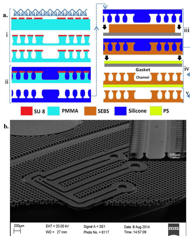
Fig. 1. (a) Process layout for fabrication of gecko-inspired adhesive integrated microfluidic devices i) PMMA master mold development ii) Silicone daughter mold casting iii) Thermo-compressive molding of SEBS iv) SEBS device with PS backing v) SEBS device without any backing layer (b) SEM image of a capillary electrophoresis microfluidic device. A cross section of a wider channel sample is as in inset
