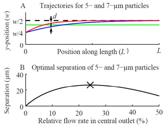
Figure 2. (A) Simulated trajectories of 5- \mu\text{m} (blue) and 7- \mu\text{m} (red) polystyrene microparticles starting from an initial position of ideal acoustic pre-alignment in width and height. Arrows indicate the point of maximal separation ( d ), the dashed black line indicates the channel center, and the green line indicates the interface between the side and central outlet flow streams. (B) Plot showing the maximum achievable particle-particle distance versus the relative center outlet flow rate when separating pre-aligned 5- and 7- \mu\text{m} particles.
