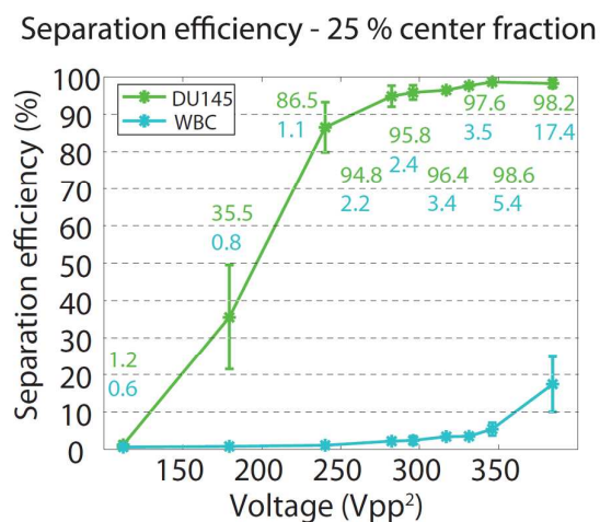
Figure 4. Separation efficiency of prostate cancer cell line, DU145, and white blood cells (WBC) when extracting 25% of the total flow in the center outlet. The total sample flow rate was 100 \mu\text{L}/\text{min} and the cells were collected through the center outlet with a flow rate of 25 \mu\text{L}/\text{min} . The error bars represents the standard deviation for n=3 .
