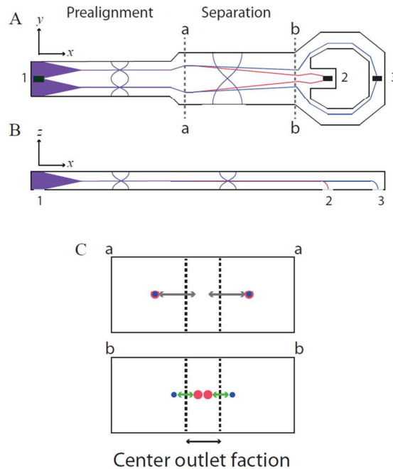
Figure 1. Illustration of the chip and particle trajectories from (A) the top and (B) the side. Cells or particles are infused at (1) and are acoustically pre-aligned in two dimensions to two positions along the width ( y -axis) of the chip and are at the same time levitated to mid-height ( z -axis) of the channel (purple lines). The pre-aligned cells then enter the wider separation channel at (a-a), where the larger, denser, or less compressible cells are focused faster towards the center of the channel (red line). Thus, these cells or particles are separated from smaller, less dense, or more compressible cells (blue line) and the two different fractions can be collected in the two outlets (2) and (3). (C) The cross sections at (a-a) and (b-b) in A, where the grey arrows indicate the necessary sideways shift of a cell to exit through the central outlet and the green arrows indicate the cell-cell distance at (b-b). The dashed black lines indicate the center outlet flow stream, which can be tuned by adjusting the relative flow rates in the center outlet (2) with respect to the flow rate in (3).
