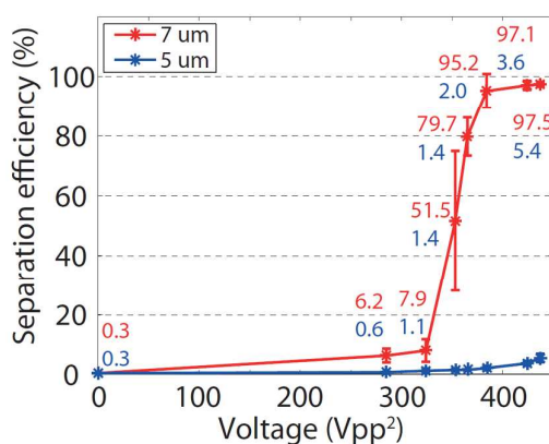
Figure 3. (A) Separation efficiency of 5- \mu\text{m} versus 7- \mu\text{m} polystyrene particles when extracting 25% of the total flow in the center outlet. The total sample flow rate was 100 \mu\text{L}/\text{min} and the particles were collected through the center outlet with a flow rate of 25 \mu\text{L}/\text{min} . (B) Separation efficiency of 5- \mu\text{m} and 7- \mu\text{m} polystyrene particles when taking out 10 % of the total fluid flow in the center outlet. The total sample flow rate was 100 \mu\text{L}/\text{min} and the particles were collected through the center outlet with a flow rate of 10 \mu\text{L}/\text{min} . The error bars represents the standard deviation for n=3 .
