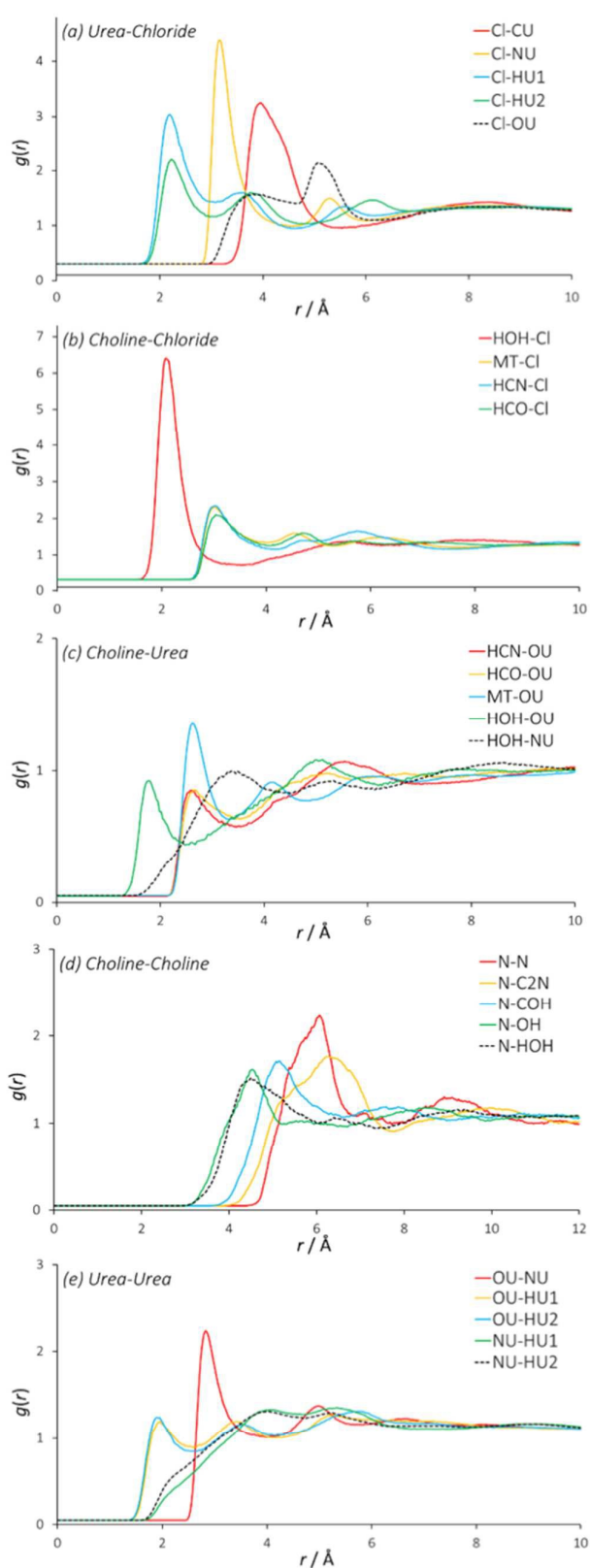
Figure 3. Partial (site-site) radial distribution functions between all different species present in the DES mixture. These RDFs are centred on specific atom types most strongly demonstrating the structuring within liquid reline for simplicity.
