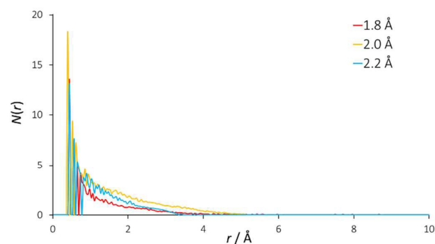
Figure 5. Radial distribution functions of void space in the EPSR model. Separate curves show the result of using different radii from each void origin to define empty spaces.
