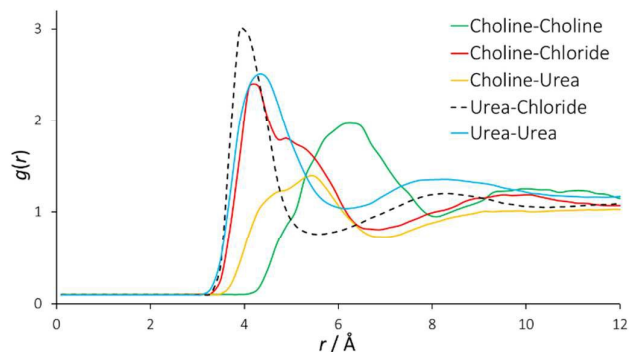
Figure 2. Radial distribution functions between all different species present in the DES mixture. For these RDFs, the molecular centres are defined as the centre of mass.
