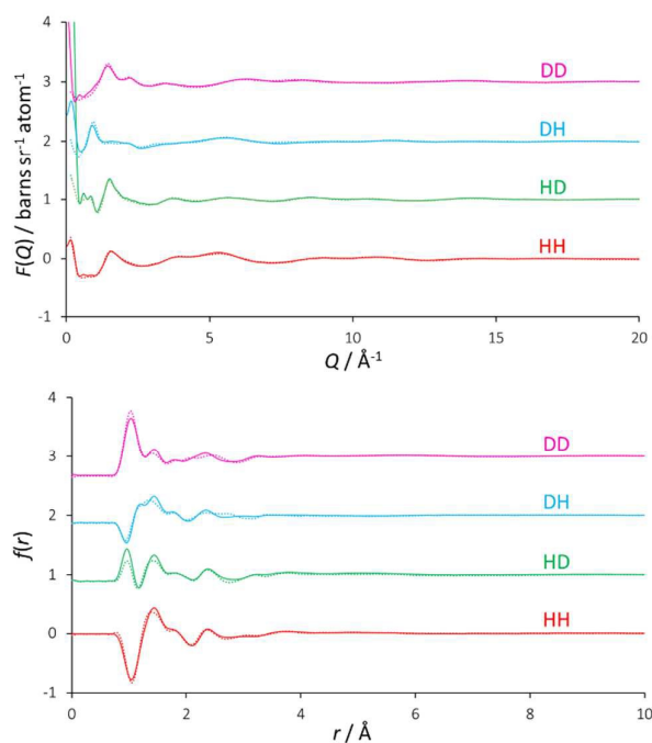
Figure 1. EPSR fits (solid coloured lines) to the total diffraction profiles (coloured circles), shown as a function of Q (upper figure) and r (lower figure) space.
