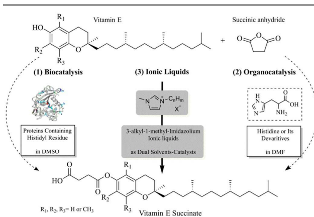
Scheme 1. Three strategies (1) biocatalysis, (2) organocatalysis and (3) using ionic liquids as dual solvent-catalysts for the esterification of vitamin E with succinic anhydride.
