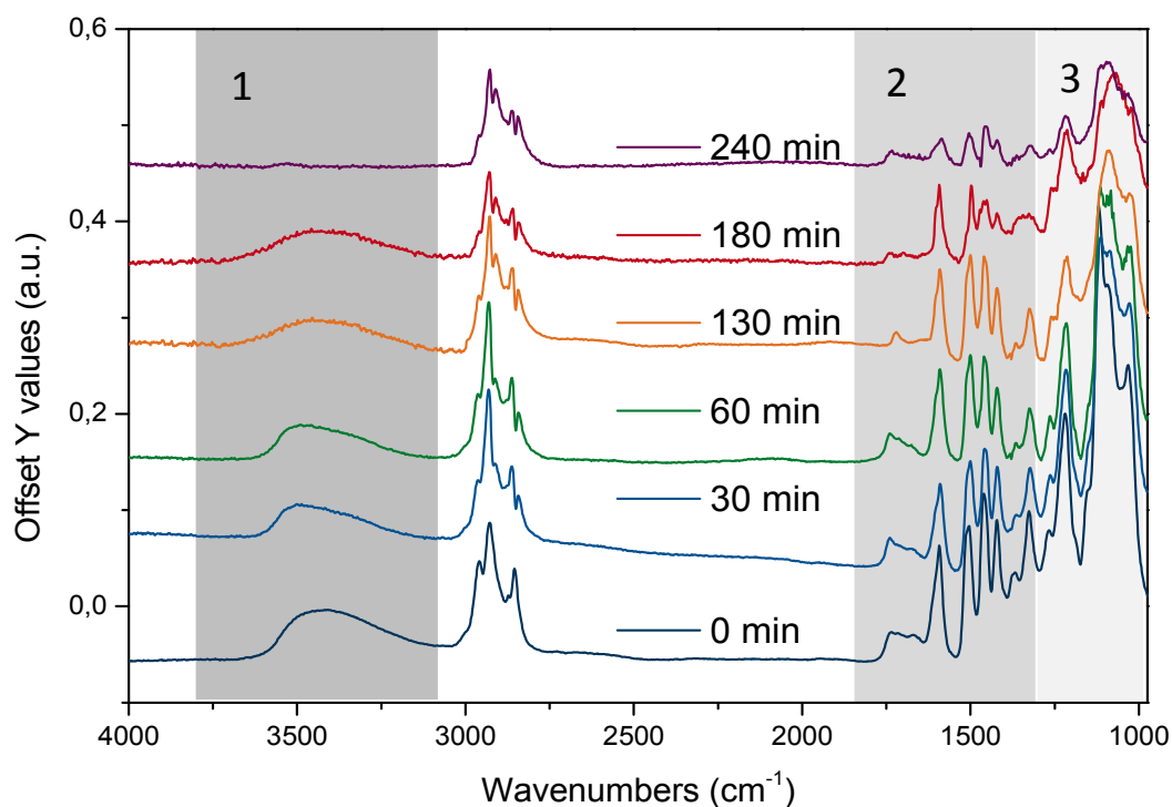
Figure 4. Time-resolved in situ ATR-IR difference spectra of organosolv lignin reacting over Ni/HBEA catalysts in n -hexadecane at 523 K and 20 bar H 2 .
