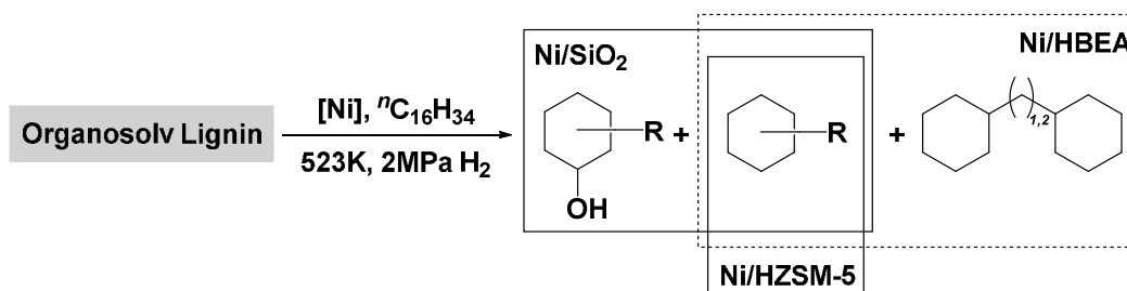
Figure 2. Schematic product distributions in the organosolv lignin deconstruction over Ni/SiO 2 , Ni/HZSM-5 and Ni/HBEA catalysts.
