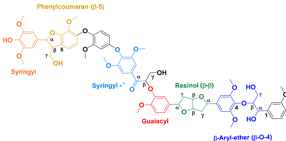
Figure 1. Elucidating the structure of beech extracted organosolv lignin. a) ATR-IR spectrum; b) 2D HSQC NMR ( \text{DMSO-}d_6 ); c) Representation of monolignolic units (S, S' and G) and its lignol linkages ( \beta -5, \beta -O-4, \beta - \beta ); d) Schematic lignin fragment showing the seven monolignols identified.
