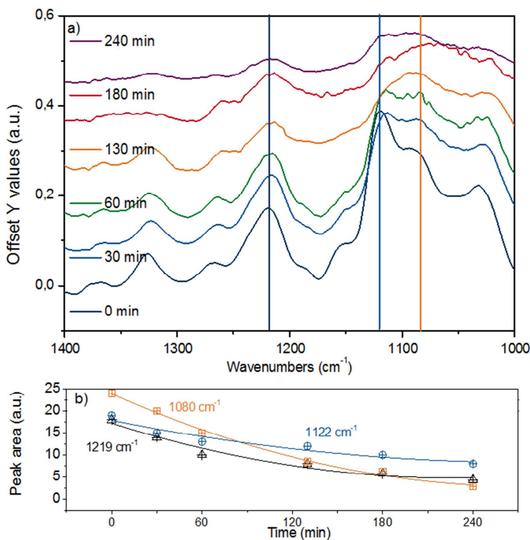
Figure 7. a) ATR-IR spectra in the spectral region of 1400 - 1000\text{ cm}^{-1} for organosolv lignin reacting over Ni/HBEA in n -hexadecane at 523 K and 20 bar \text{H}_2 . b) Deconvoluted and integrated peak areas at 1219\text{ cm}^{-1} , 1122\text{ cm}^{-1} and 1080\text{ cm}^{-1} representing the aromatic C-C-O stretching vibration, the aliphatic secondary and primary C-C-O stretching vibrations, respectively.
