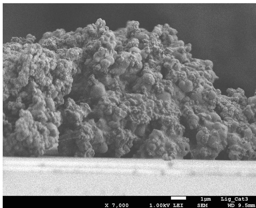
Figure 3. HR-SEM cross section of the lignin-catalyst physical mixture being deposited as a layer on the silicon crystal through drop coating.
