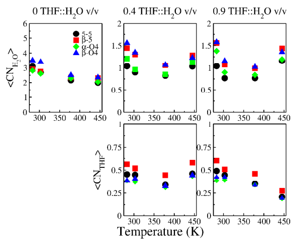
Figure 10) Solvent-lignin (bond) coordination numbers. Top row sub-figures correspond to H 2 O coordination while the bottom row correspond to THF coordination. Error-bars are standard-error of the mean and are at most the size of the data-points.
