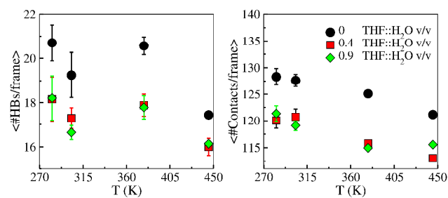
Figure 6) (Left) Average number of lignin-lignin hydrogen-bonds per frame (one frame corresponds to 20ps). (Right) Average number of lignin-lignin contacts per frame. Error bars are standard error of the mean.
