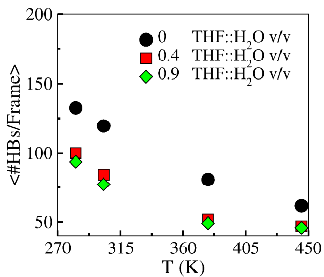
Figure 7) Average number of lignin-water HBs per frame (one frame corresponds to 20ps). Error bars are equal to or smaller than the size of each shape and are of the standard error of the mean.
