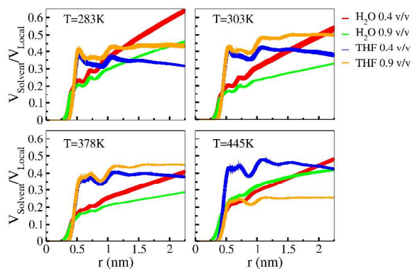
Figure 9) Solvent occupied local volume ratios. The radius of the local volume near the lignin is taken to be a sphere with a radius centered at 0.35nm and ranging up to ~1.1nm. Error-bars are standard error of the mean and are the width of the line.
