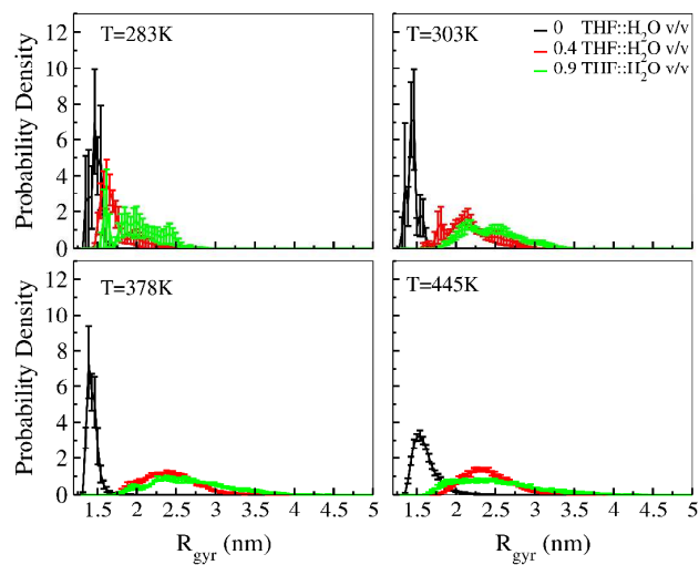
Figure 2) Average radius of gyration ( R_g ) distributions of lignin. Error-bars are standard error of the mean of each histogram bin.
