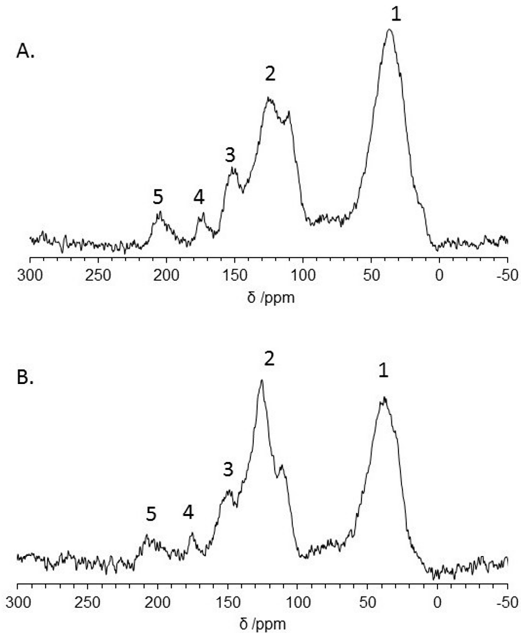
Figure 5. ^{13}\text{C} CP MAS NMR spectras of A. FruLi and B. FruLi+TCA in which 1. Aliphatic \text{sp}^3 carbon, 2. \text{sp}^2 carbon related structures 3. Furan type structure, 4. Carboxylate and 5. Ketone/aldehyde.
