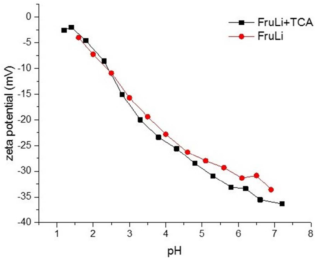
Figure 6. Development of the surface charge of FruLi and FruLi+TCA as a function of pH.
