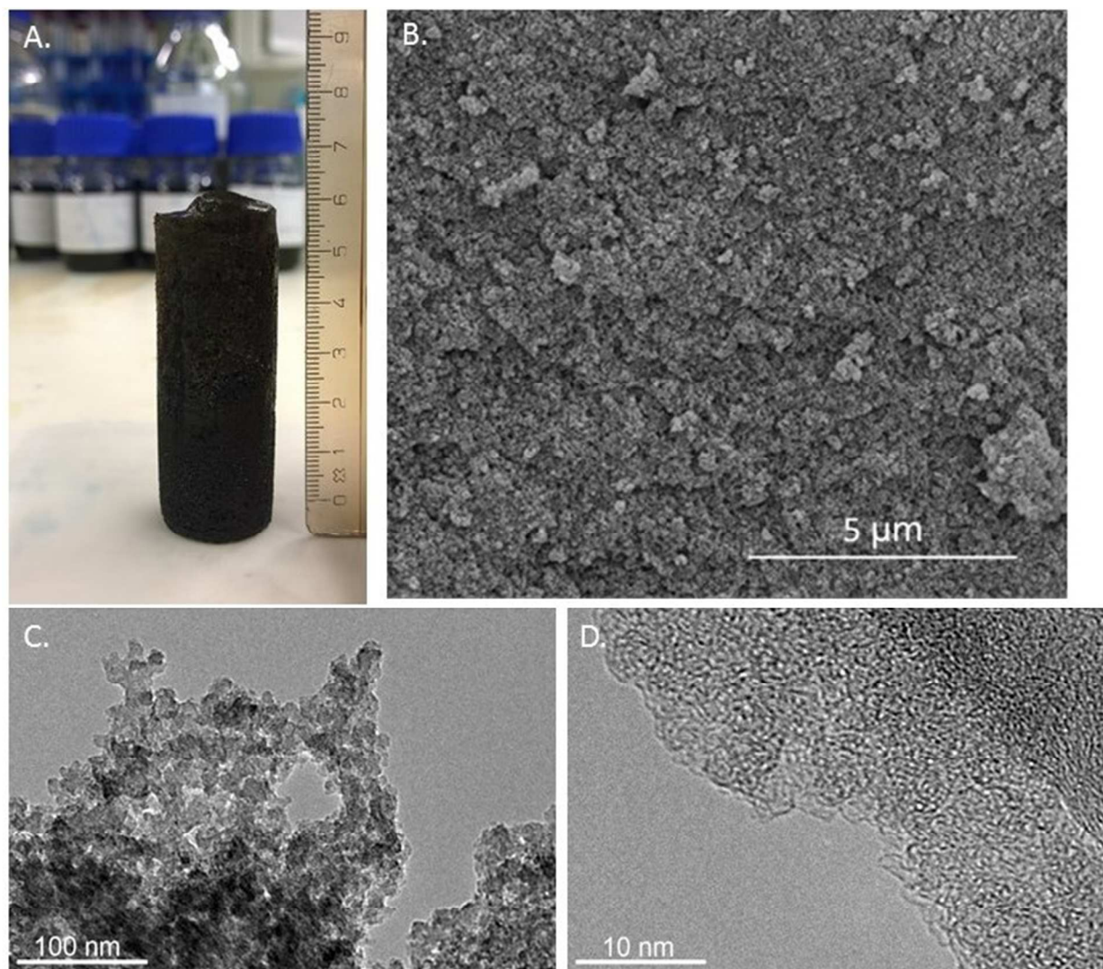
Figure 1. A. Monolithic carbon structure (fructose based, FruLi) after synthesis, B. SEM image 20k magnification, C. and D. TEM images with 60k and 600k magnifications respectively.
