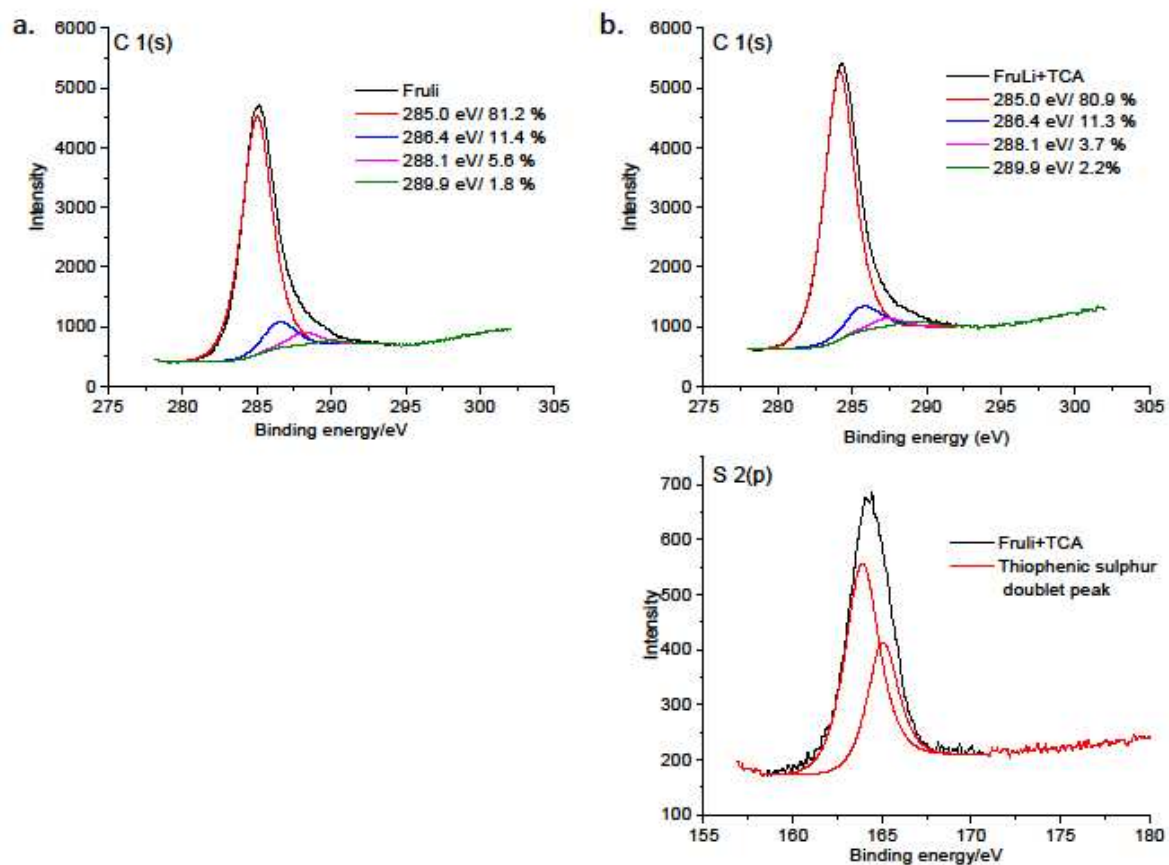
Figure 4. XPS C 1(s) deconvolution spectra of A. FruLi and B. FruLi+TCA C 1(s) and S 2(p) deconvolution spectras.
