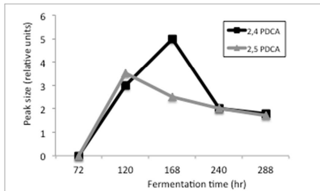
Figure 3. LC-MS peak height for bioproducts 2,4-PDCA (black) from R. jostii pTipQ2-ligAB and 2,5-PDCA (gray) from R. jostii pTipQ2-praA grown on M9 minimal media containing 0.1% vanillic acid vs fermentation time
