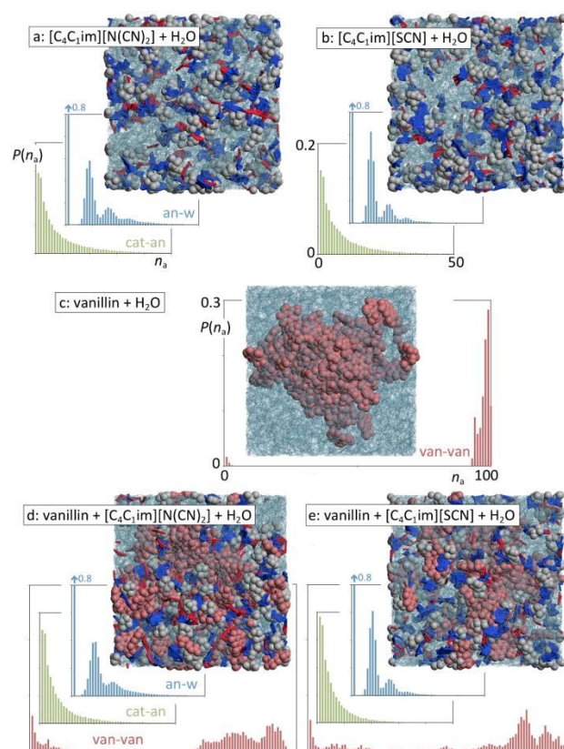
Fig. 12 Simulation snapshots and discrete probability distribution functions of aggregate sizes, P(n_a) for different types of system and aggregate type. (a-b) Ionic liquid aqueous solutions; (c) Water-vanillin mixture; (d-e) Vanillin in ionic liquid aqueous solutions. (green graphs): ionic liquid polar aggregates (strands); (blue graphs): anion-water network; (red graphs) vanillin clusters.
