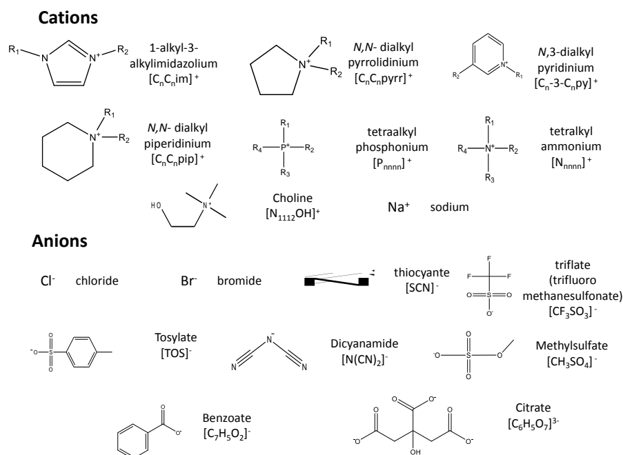
Fig. 2 Chemical structures of the anions and cations of all ILs and salts investigated.
