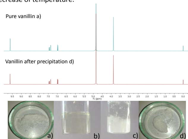
Fig. 14. a) appearance of commercial vanillin and respective ^1\text{H} NMR spectrum; b) vanillin dissolved in 0.80 \text{ mol} \cdot \text{kg}_{\text{water}}^{-1} aqueous solution of [\text{C}_4\text{C}_1\text{im}][\text{TOS}] at 303 K; c) precipitation of vanillin with the addition of water and decrease of temperature; and d) recovered vanillin and respective ^1\text{H} NMR spectrum.
