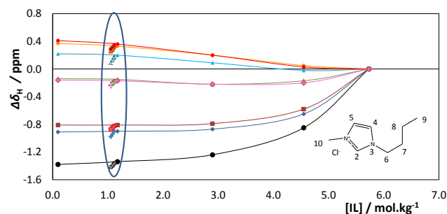
Fig. 11 1 H NMR chemical shift deviations of [C 4 C 1 m]Cl in aqueous solutions relative to pure [C 4 C 1 m]Cl (5.7 mol.kg -1 ): (●) H(2), (◆) H(4), (■) H(5), (▲) H(6), (▲) H(7), (●) H(8), (●) H(9), and (●) H(10). Effect of the vanillin concentration within the blue ellipse.
