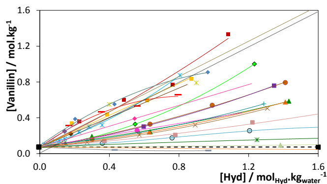
Fig. 5 Influence of the hydrotropes (ionic liquids and conventional salts) concentration in the solubility of vanillin in aqueous solutions at 303 K: (---, ■)
