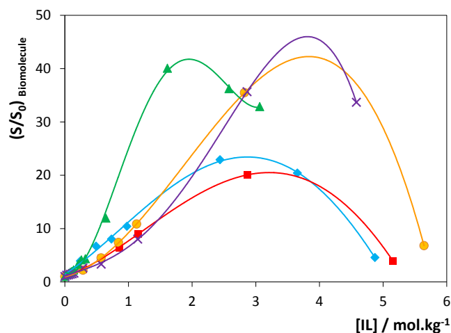
Fig. 3 Influence of the ILs concentration in the solubility of gallic acid in aqueous solutions of [\text{C}_4\text{C}_1\text{im}][\text{N}(\text{CN})_2] , and [\text{C}_4\text{C}_1\text{im}]\text{Cl} , and vanillin in aqueous solutions of [\text{C}_2\text{C}_1\text{im}][\text{N}(\text{CN})_2] , [\text{C}_4\text{C}_1\text{im}][\text{TOS}] and [\text{C}_4\text{C}_1\text{im}]\text{Cl} at 303 K. Lines are guides for the eye.
