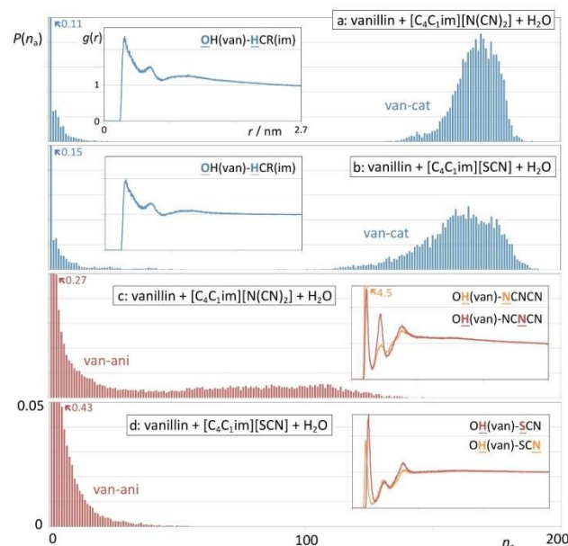
Fig. 13 Discrete probability distribution functions of aggregate sizes, P(n_a) , and (as insets) pair radial distribution functions, g(r) , for different types of aggregate type and pairs of interaction centre. (a-b) size distribution of cation-vanillin aggregates and cation-vanillin interactions in the systems with (a) [N(CN)_2] -induced and (b) [SCN] -induced hydrotropy. (c-d) size distribution of anion-vanillin aggregates and anion-vanillin interactions in the systems with (c) [N(CN)_2] -induced and (d) [SCN] -induced hydrotropy.
