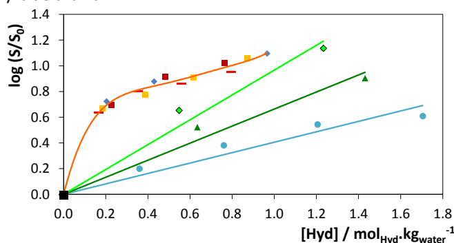
Fig. 7 Influence of the ionic liquids concentration in the vanillin solubility at 303 K: (■), pure water, (●) [C_2C_1im]Cl , (▲) [C_4C_1im]Cl , (◆) [C_6C_1im]Cl , (■) [C_8C_1im]Cl , (◆) [C_{10}C_1im]Cl , (■) [C_{12}C_1im]Cl , and (■) [C_{14}C_1im]Cl .
