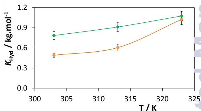
Fig. 9 K_{Hyd} temperature dependency for the solubility of vanillin in aqueous solutions of (◆) [C 2 C 1 im][N(CN) 2 ] and (●) [Na][C 7 H 5 O 2 ].
