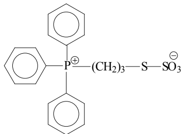
Triphenylphosphoniopropylthiosulfate zwitterion
