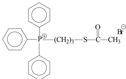
(3-Thioacetylpropyl)triphenylphosphonium bromide
