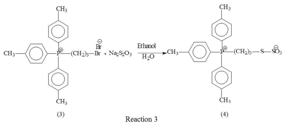
Scheme 1: Synthesis of tri( p -tolyl)phosphoniopropylthiosulfate zwitterion (4)
