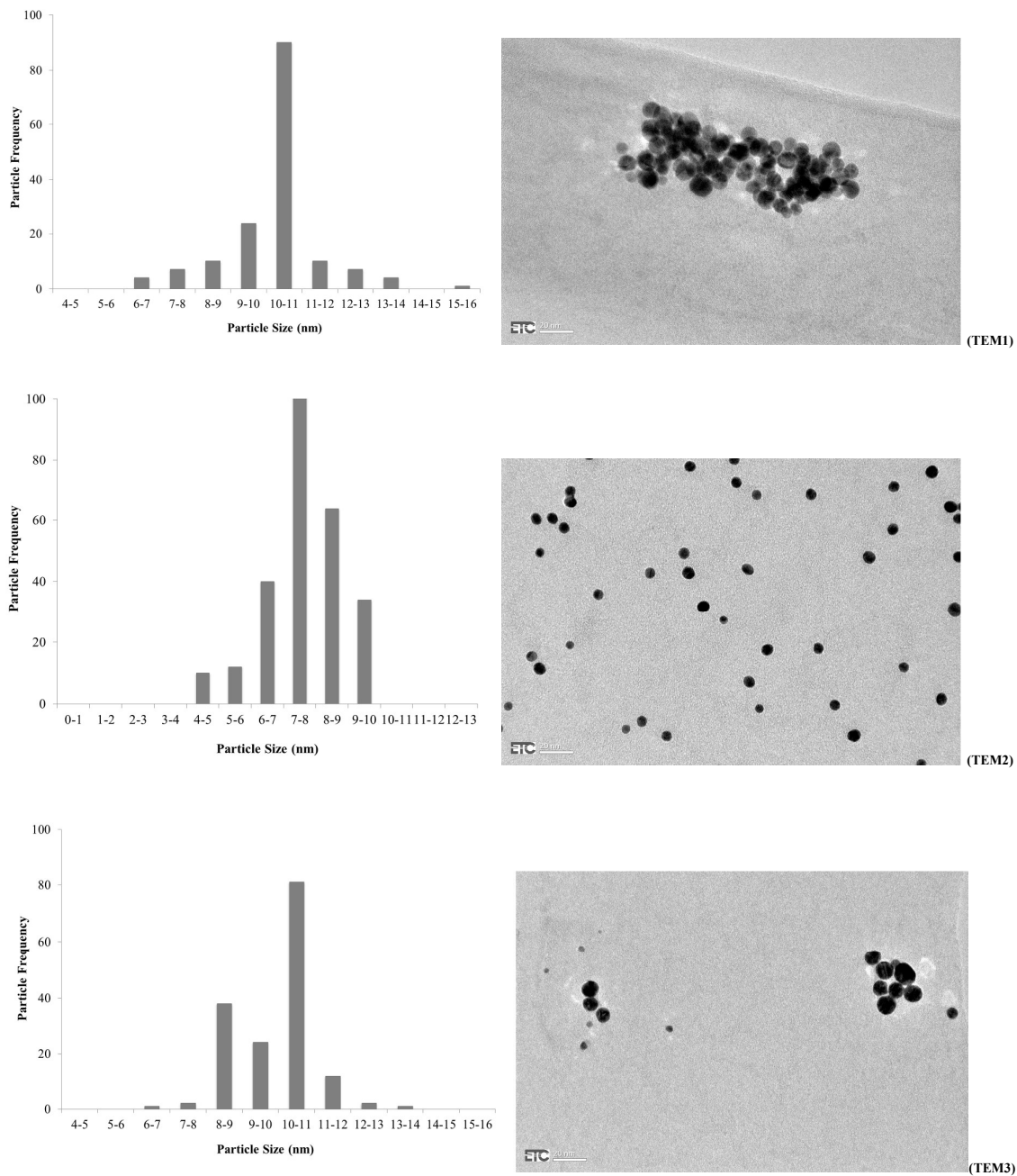
Figure 5. Representative TEM micrographs of cationic phosphonium gold nanoparticles synthesised using triphenylphosphoniopropylthiosulfate ( TEM1 ), (3-thioacetylpropyl)triphenylphosphonium bromide ( TEM2 ), and tri( p -tolyl)phosphoniopropylthiosulfate ( TEM3 ) as protecting ligands in DMSO, and corresponding particle size histograms.
