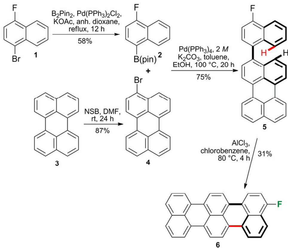
Synthesis of 3-fluoroterrylene 72x61mm (300 x 300 DPI)
