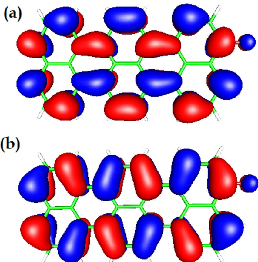
(a) LUMO and (b) HOMO for 3-fluoroterrylene. 98x98mm (120 x 120 DPI)
