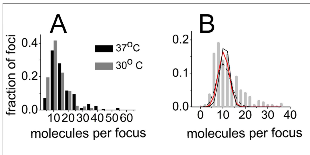
Figure 7. SeqA foci do not have a fixed number of molecules per focus.
