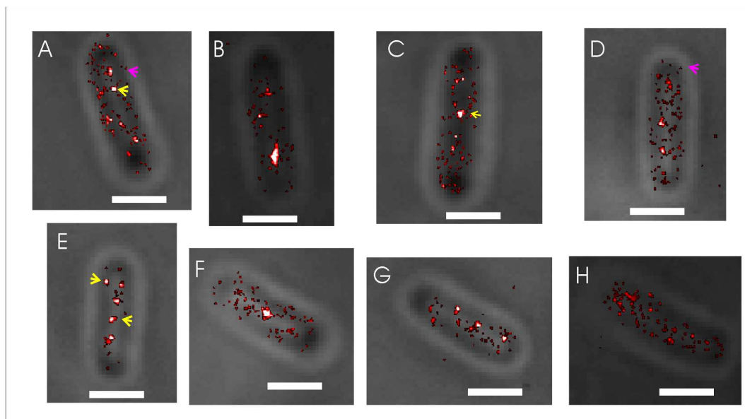
Figure 2. PALM imaging of SeqA in Escherichia coli cells shows the molecules localized to heterogeneous structures.
