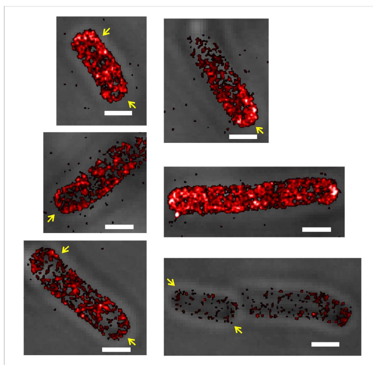
Figure 10. PALM reconstructions of Escherichia coli \Delta dam cells overexpressing SeqA-PAmCherry from a plasmid.
