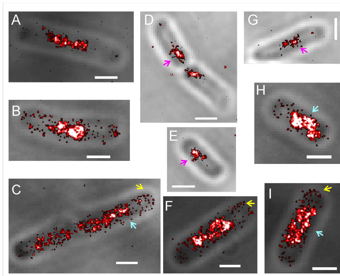
Figure 9. PALM reconstructions of Escherichia coli cells overexpressing SeqA-PAmCherry from a plasmid.
