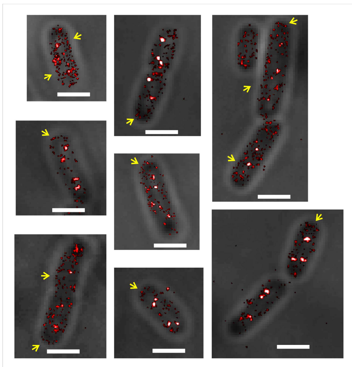
Figure 3. PALM images of Escherichia coli cells where a fraction of the SeqA molecules localize to the membrane.
