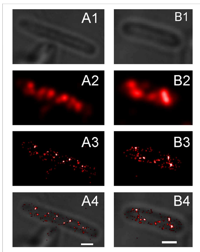
Figure 1. PALM imaging shows more detail of the SeqA foci in Escherichia coli than conventional fluorescence microscopy.
