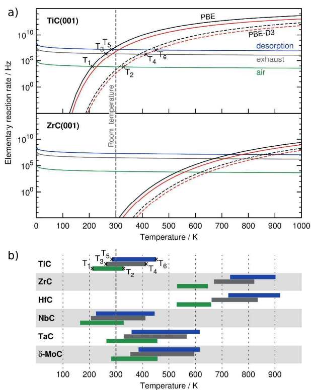
Fig. 2: a) Calculated rates for desorption and adsorption of CO 2 on TiC and ZrC (001) surfaces. On TiC, marked points with T_1 – T_6 labels in a) and b) show how desorption temperature ranges in b) have been obtained. Legend for a): Green, grey, and blue; adsorption rates on a single site per time unit for a CO 2 partial pressure of 40, 15·10 3 , and 10 5 Pa, respectively. Black and red; desorption rates per site and time unit from MMC and TopC sites. PBE (solid) and PBE-D3 (dashed) values are provided. Legend for b): Green, grey, and blue bars belong to desorption temperature ranges for CO 2 partial pressures of 40, 15·10 3 , and 10 5 Pa, respectively.
