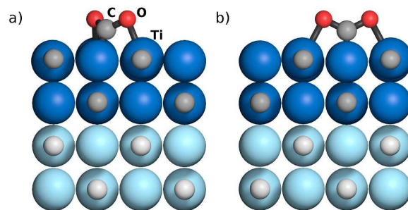
Fig. 1 Side sketches of CO 2 adsorbed on a) MMC and b) TopC sites of TiC(001) surface. Atom labels indicate the sphere colouring. Lighter colour layers were fixed during optimization. For respective top views see Figure S1 of the ESI†.
