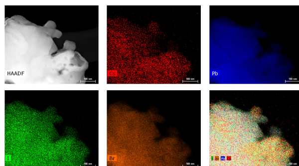
Figure 4. HAADF and TEM-EDS image of Cs 0.2 FA 0.8 PbI 2.84 Br 0.16 .
