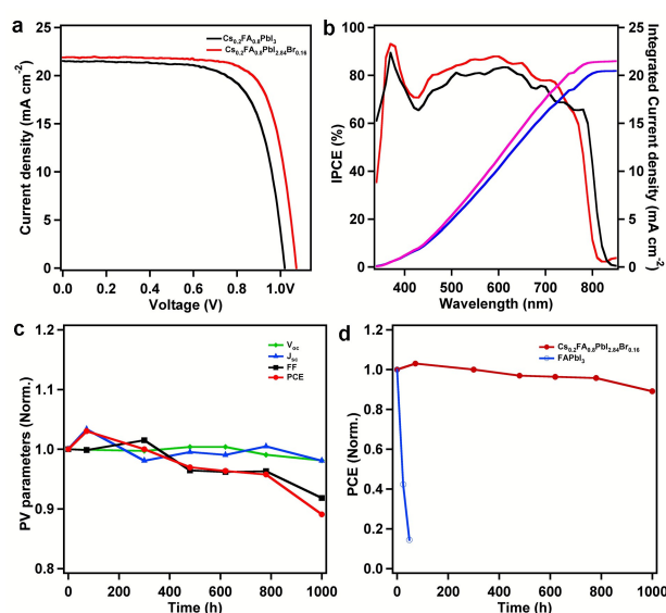
Figure 6. Photovoltaic properties of \text{Cs}_{0.2}\text{FA}_{0.8}\text{PbI}_3 and \text{Cs}_{0.2}\text{FA}_{0.8}\text{PbI}_{2.84}\text{Br}_{0.16} perovskite solar cells. a , J-V curves of the \text{Cs}_{0.2}\text{FA}_{0.8}\text{PbI}_3 and \text{Cs}_{0.2}\text{FA}_{0.8}\text{PbI}_{2.84}\text{Br}_{0.16} perovskite solar cells. b , IPCE spectra of the \text{Cs}_{0.2}\text{FA}_{0.8}\text{PbI}_3 (black) and \text{Cs}_{0.2}\text{FA}_{0.8}\text{PbI}_{2.84}\text{Br}_{0.16} (red) perovskite solar cells and their integrated currents \text{Cs}_{0.2}\text{FA}_{0.8}\text{PbI}_3 (blue) and \text{Cs}_{0.2}\text{FA}_{0.8}\text{PbI}_{2.84}\text{Br}_{0.16} (purple). c , Evolution of the Photovoltaic parameters with time for the \text{Cs}_{0.2}\text{FA}_{0.8}\text{PbI}_{2.84}\text{Br}_{0.16} perovskite solar cells. The unsealed solar cells were kept under ambient conditions in the dark and the performances were re-evaluated at periodic intervals. d , Comparison of the stability of \text{Cs}_{0.2}\text{FA}_{0.8}\text{PbI}_{2.84}\text{Br}_{0.16} and FAPbI 3 perovskite solar cells, conditions as in Figure 6c.
