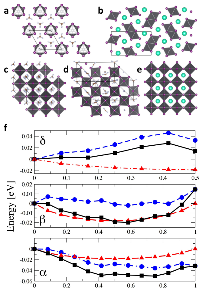
Fig. 5 Various phases of FAPbI 3 and CsPbI 3 and variation of internal energy of mixed Cs x FA 1-x PbI 3 in different phases. a and b represent the \delta phase in the FA and Cs perovskites, respectively; c and d show the \alpha and \beta FAPbI 3 , respectively. e shows the cubic phase of the CsPbI 3 structure. Comparison between the structures reported in panels a and b, and panels b, c and e highlights the significant difference in the \delta structure of FA and Cs lead iodide, as opposed to the strong similarities in the corresponding perovskite phases. f, Variation of internal energy, \Delta E (dashed blue line), mixing entropy contribution, -T\Delta S (dot-red dashed line), and free energy, \Delta F = \Delta E - T\Delta S (black continuous line) as a function of Cs content, x .
