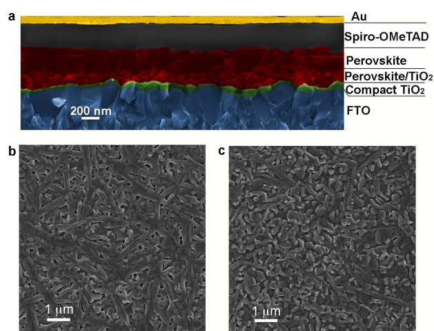
Fig. 3 a, cross-sectional SEM image of a complete photovoltaic device. b, top-view SEM image of the Cs 0.2 FA 0.8 PbI 3 perovskite. c, top-view SEM image of the Cs 0.2 FA 0.8 PbI 2.84 Br 0.16 perovskite.
