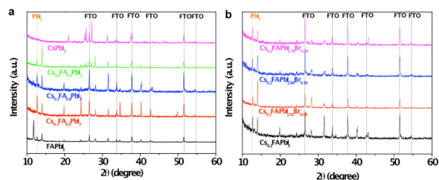
Fig. 2. a, XRD spectra of FAPbI 3 , CsPbI 3 and the Cs x FA (1-x) PbI 3 . b, Effect of iodide substitution by bromide on the XRD spectra of Cs 0.2 FA 0.8 PbI (3-y) Br y .
