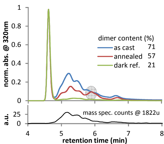
Figure 3: Top: High performance liquid chromatography (HPLC) traces from UV-vis detection at 320 nm of illuminated and re-dissolved PC60BM films normalized to the monomer peak at 4.6 min. A significant amount of dimer is observed in the as cast film (blue) between 5 and 7 min retention time (herein referred to as 'dimer region'). Annealing at 180°C for 10 min before illumination (red) reduces dimerization. Films were illuminated 40 hours under a one sun equivalent white light LED. The dark reference (green) was exposed to a small amount of ambient light. Bottom: For an aged as cast sample, a mass spectrometry trace (HPLC-MS in APCI mode) was recorded using single-ion-monitoring (SIM) at an atomic mass of 1822 u, which represents the PC60BM dimer mass. The excellent correlation between the SIM and the UV trace confirms that the signal between 5 and 7 minutes corresponds to PC60BM dimers. Multiple isomers have different geometries and HPLC retention times, which explains the presence of multiple dimer peaks between 5 and 7 minutes.
