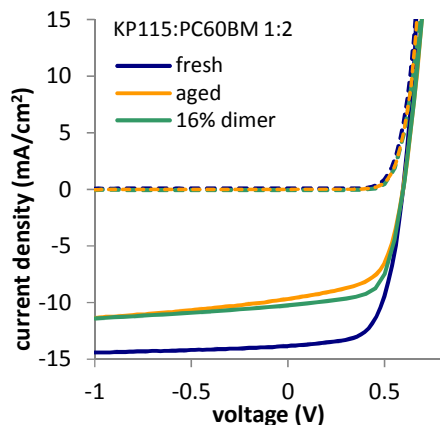
Figure 1: Light (solid lines) and dark (dashed lines) JV curves of fresh and aged (120 h) KP115:PC60BM solar cells along with KP115:PC60BM solar cells containing 16% PC60BM dimers, added during cell production. PC60BM dimers were isolated using HPLC from photo-irradiated PC60BM films. The structure of KP115 (PDTSTzTz) 3,33,34 is given in the supporting information.
