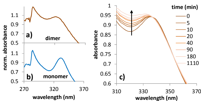
Figure 6: UV-vis absorption of a) PC60BM dimer and b) PC60BM monomer as obtained from HPLC data at 4.6 min and 5.3 min retention time, see also Figure 3. c) Spectral changes during illumination of a PC60BM film indicate the formation of dimers.
