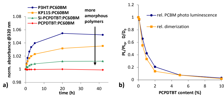
Figure 7: a) Photo-induced dimerization measured with UV-vis absorption in polymer-fullerene (1:2) blends with different degrees of polymer aggregation. b) Relative PC60BM photoluminescence (PL/PL 0 ), which is obtained by integration over the emission band and normalization to the value in neat PCBM, and the relative degree of dimerization compared to a plain PC60BM film (D/D 0 ) as measured by absorption is plotted for a series of fullerene films with increasing content of PCPDTBT.
