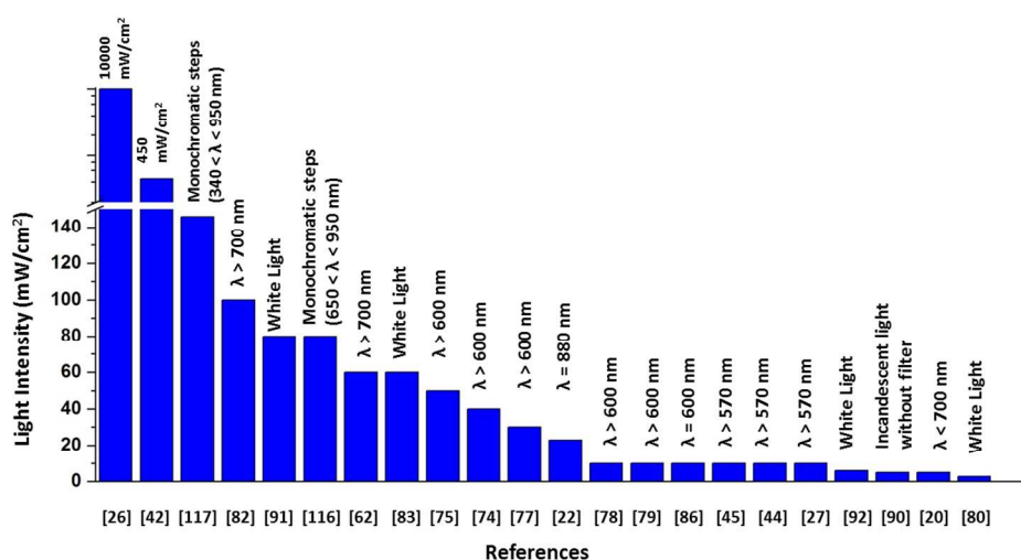
Fig. 17 Intensity and wavelength range adopted in literature for solar cell illumination
