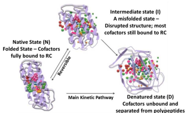
Fig. 18 A schematic of thermal denaturation of RCs as described in ref.121. The spheres of various colours represent the RC cofactors and the ribbons represent the polypeptides. (The scheme is illustrative and does not represent the true structure of RC)
