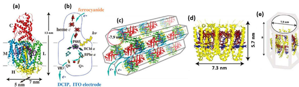
Fig. 12 (a) Structure of the RC complex-(L, M, H, and C are the RC's subunit polypeptides), (b) electron transfer cofactors and pathway inside the RC, (c) schematic view of the RC inside silica nanopores in FSM7.9. (d) Molecular structure of LH2 complex, (e) schematic view of LH2-FSM7.9 conjugate. The value for 'a' in (e) was estimated to be 9.2-11.4 nm upon the binding of 1.11 mg of LH2/mg of FSM7.9 based on the results in the specific study. [Reproduced with permission from ref. 104 (Copyright © 2010, American Chemical Society) and ref. 106 (Copyright © 2006, American Chemical Society)]
