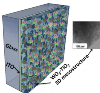
Fig. 8 RCs immobilized to \text{WO}_3\text{-TiO}_2 3D mesostructure; inset – TEM image of the mesoporous structure of \text{WO}_3\text{-TiO}_2 [Adapted with permission from ref.90, Copyright © 2005, American Chemical Society]
