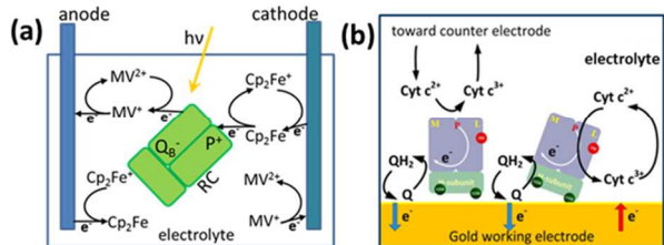
Fig. 13 (a) Reaction centers added to electrolyte with two electron transfer mediators (ferrocene and methyl viologen). The thick arrows represent reactions with high reaction rate constants, while the thin arrows represent reactions that reduce cell efficiency. [Adapted from ref. 80] (b) Reaction centers added to electrolyte with two electron transfer mediators (Ubiquinone-10 and cytochrome c) [Reproduced with permission from ref. 116, Copyright © 2012, American Chemical Society]
