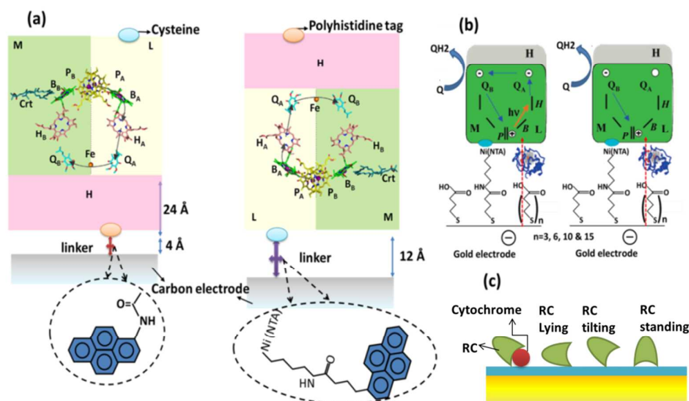
Fig. 7 (a) Two possible ways of RC binding and ET pathways between RC and electrode. P- primary electron donor (special pair), B-monomeric bacteriochlorophyll, H-bacteriopheophytin, Qa and Qb-primary and secondary electron acceptors (quinones). [Adapted from ref. 81 and ref.34, with permission from Elsevier Ltd] (b) Photoinduced- and dark- electron transfers in RC-Cyt-SAM-Gold electrode [Adapted with permission from ref.82, Copyright © 2007, American Chemical Society] (c) Different orientations of RC with cytochrome c on NTA SAM modified electrode [Adapted with permission from ref. 18, Copyright © 2006, American Chemical Society]
