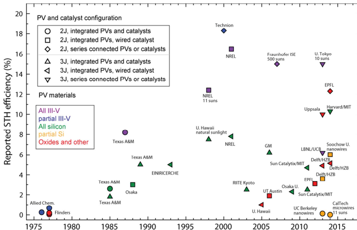
Fig. 3. Reported solar to hydrogen (STH) conversion efficiencies as a function of year and sorted by the number of tandem photovoltaic junctions used (2 or 3). The degree of integration of photovoltaic and catalyst elements is also distinguished, see Fig. 2. The fill colour represents the semiconductor materials used in the photovoltaic portion of the device. All STH conversion efficiencies are as reported in the original publications (see Tables 2 – 5).
