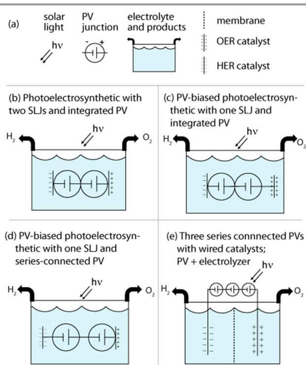
Fig. 2. Depiction of commonly employed solar photoelectrochemical water splitting architectures in circuit diagram form. (a) Key for symbols used; see Table 1 for abbreviations. Wires are indicated by solid lines. If elements are touching without a wire (e.g. the PVs) they are monolithically integrated. (b) The photoelectrosynthetic geometry shown in Fig. 1 with integrated PV elements and with both catalysts integrated. (c) A PV-biased photoelectrosynthetic device with one buried junction (the photoanode wired to the OER catalyst) and one SLJ. (d) A PV-biased photoelectrosynthetic device with series-connected PV elements where the OER catalyst is integrated and the HER catalyst is wired. (e) A PV + electrolyzer approach with 3 PV cells wired in series and a membrane is used to separate chemical reaction products.
