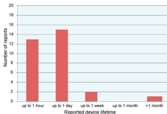
Fig. 4. Histogram of reported lifetimes for the overall water splitting devices tabulated in Tables 2 – 5. Long-term operational stability remains a central challenge for achieving scalable systems
