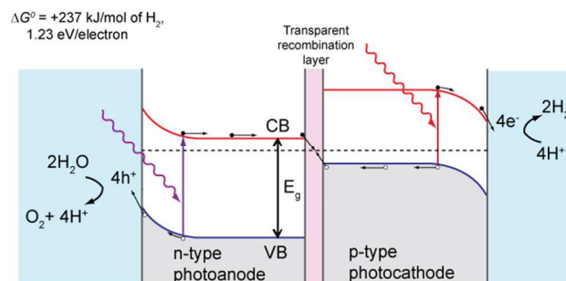
Fig. 1. Schematic of an idealized tandem-junction photoanode and photocathode device during steady-state operation. The process of solar water splitting is overlaid on the equilibrium diagram. Proton conduction in the electrolyte from the anode to the cathode is required for continuous operation. Adapted from Nozik. 42
