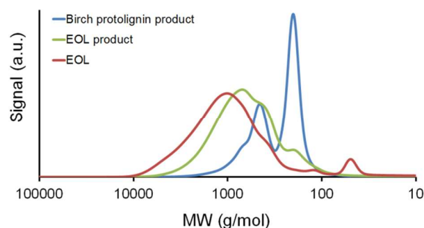
Fig. 3 Gel permeation chromatograms of ethanol organosolv lignin (EOL) and the DCM lignin oils, obtained after hydrogenolysis of EOL and birch sawdust (entry 1 and 2, table 2). Polystyrene standards were used for calibration.
