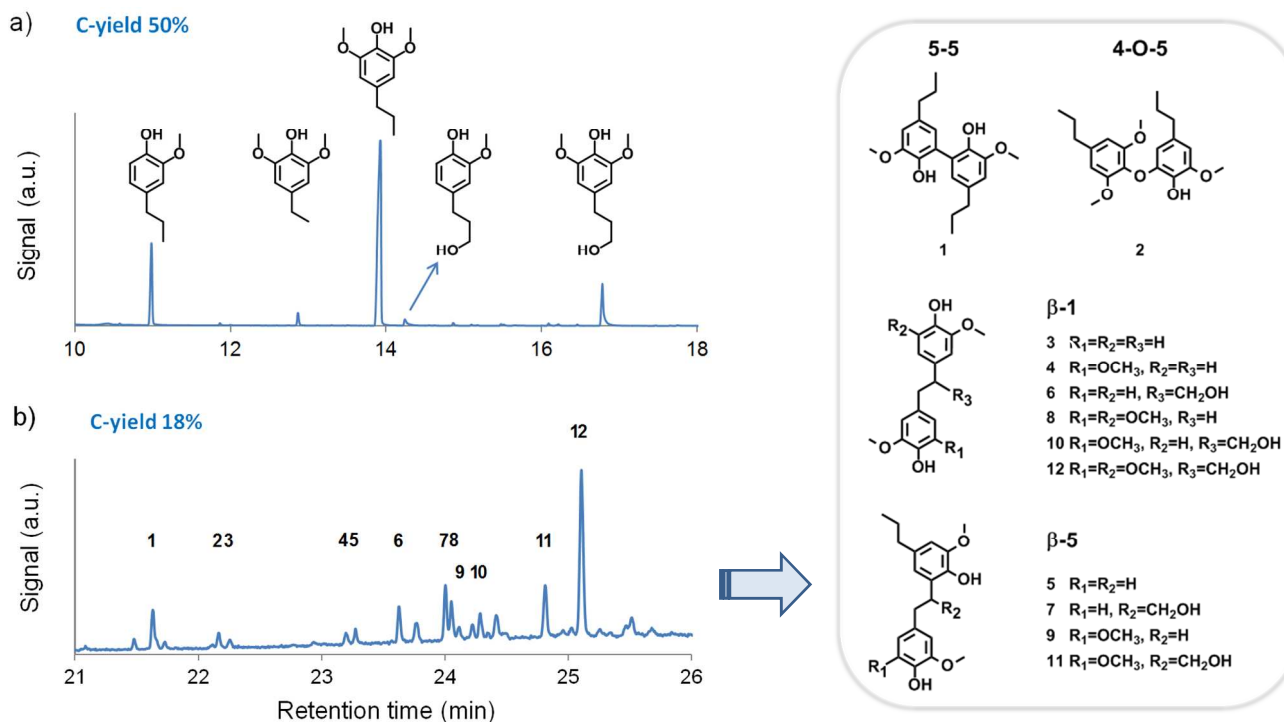
Fig. 1 Gas-chromatograms and peak identification of a) the lignin monomer fraction (left to right: 4- n -propylguaiacol, 4-ethylsyringol, 4- n -propylsyringol, 4- n -propanolguaiacol and 4- n -propanolsyringol) and b) the trimethylsilylated dimer fraction after birch hydrogenolysis (reaction conditions from entry 5, Table 1). C-yield represents the carbon yield, as defined in the experimental section.
