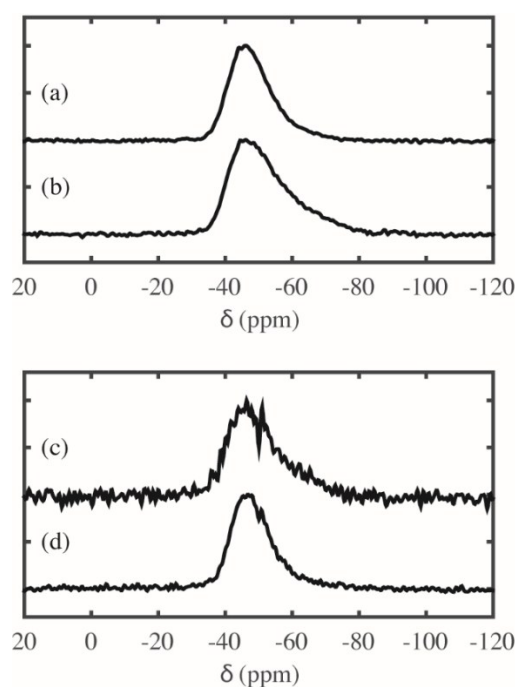
Fig. 1 ^{29}\text{Si} CP-MAS NMR spectra of silicon imidonitride samples prepared from triflic acid or ammonium triflate catalysed gels and fired at 1000 °C. Catalyst: (a) 1-2 drops triflic acid; (b) 10% [\text{NH}_4][\text{OTf}] ; (c) 5% [\text{NH}_4][\text{OTf}] ; (d) 0.4% [\text{NH}_4][\text{OTf}] . Note that (a) and (b) were recorded at 14.1 T, whereas (c) and (d) were recorded at 9.4 T.
