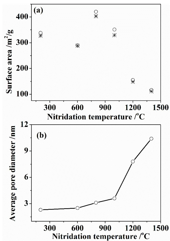
Fig. 11 Heating temperature variation in surface area (a) and average pore size (b) of silicon imidonitride/nitride samples produced by heating gels made with 0.4% [NH_4][OTf] for 6 h. In the surface area plot (a) the open circles are multi point and the stars single point surface area.
