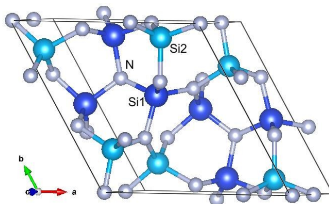
Fig. 5 Plot of the non-centrosymmetric structure of \alpha\text{-Si}_3\text{N}_4 , using the refined atomic coordinates in Table S1 and showing the 6-membered rings. The Si1 silicon atoms are shown in blue and Si2 in a lighter shade of blue. Nitrogen atoms are shown in grey.
