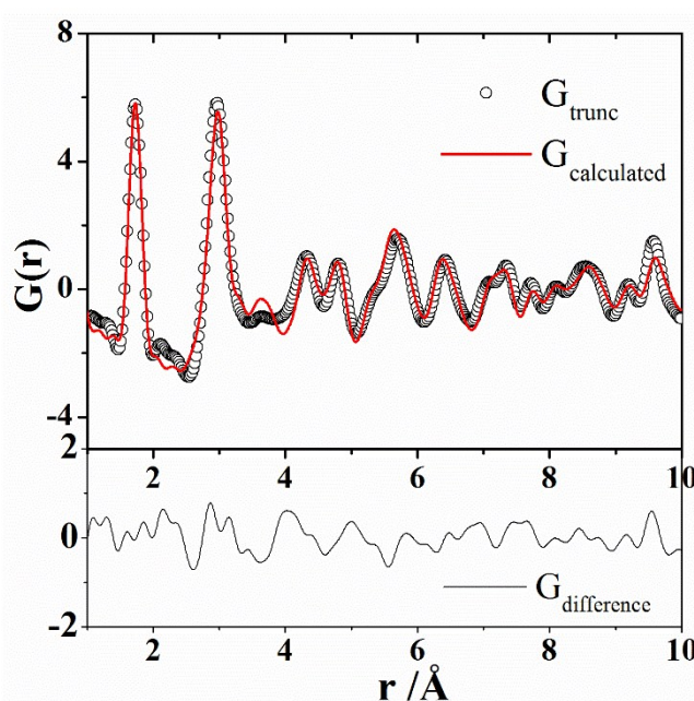
Fig. 6 Real space refinement of the PDF from a silicon imidonitride sample synthesised at 1400 °C for 18 h. Starting model: \alpha\text{-Si}_3\text{N}_4 with refined coordinates from the Rietveld refinement of the Bragg pattern described above.
