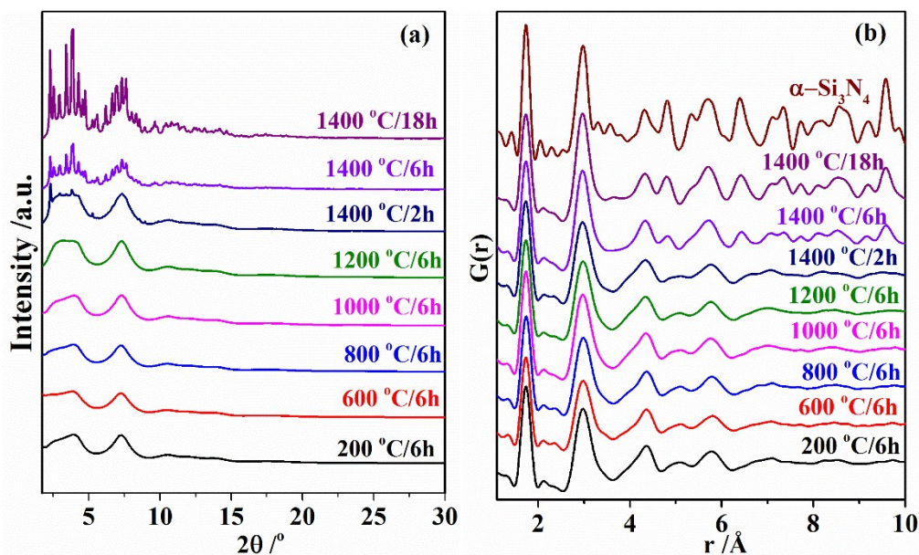
Fig. 4 Total scattering intensity with polyimide capillary subtracted (a, \lambda = 0.1722 Å) and PDFs (b) of silicon imidonitride/nitride samples produced by heating gels made with 0.4% [\text{NH}_4][\text{OTf}] at the temperatures shown, and calculated PDF of \alpha\text{-Si}_3\text{N}_4 (top right). 27
