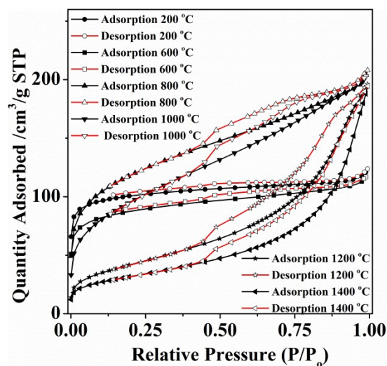
Fig. 10 N_2 adsorption-desorption isotherms of silicon imidonitride/nitride samples produced by heating gels made with 0.4% [NH_4][OTf] at temperatures shown for 6 h.
