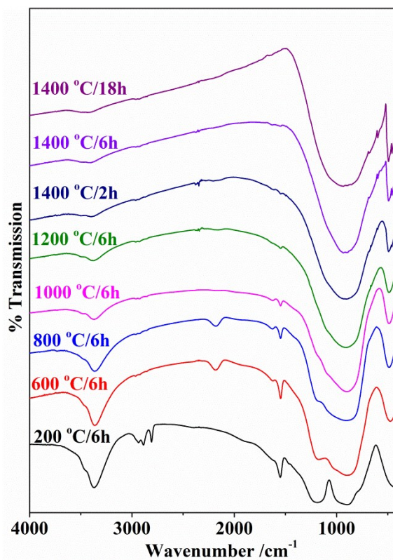
Fig. 3 Infrared spectra of silicon imidonitride/nitride samples produced by heating xerogels made with 0.4% [\text{NH}_4][\text{OTf}] in ammonia at the temperatures shown.
