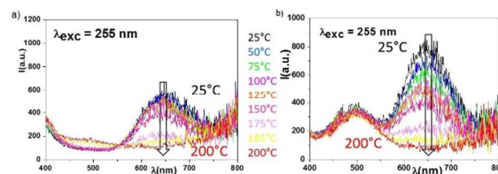
Fig. 6 Room temperature emission graphs under a 255 nm excitation beam obtained after a 2-hour irradiation at 315 nm. The irradiated crushed crystals were successively heated from 25°C to 200°C under a reductive atmosphere of Ar/H 2 10%. a) 0.081% of Ce 3+ content (LC) and b) 0.348% of Ce 3+ content (HC).
