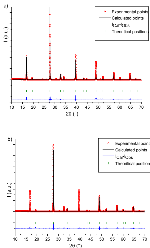
Fig. 1: Rietveld diffraction pattern refinements illustrated on \text{Rb}_2\text{KInF}_6 : Ce a) LC crystal (targeted concentration equal to 2%) and b) HC crystal (targeted concentration equal to 10%).
