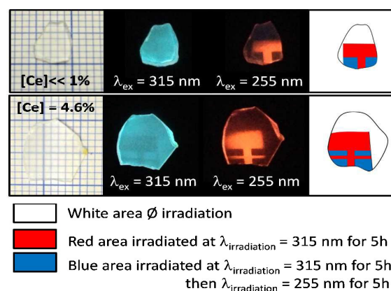
Fig. 7 Printing tests performed on single crystals. Photographs of Ce-doped Rb 2 KlnF 6 single crystals after several irradiation processes.
