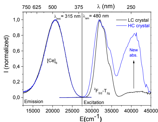
Fig. 2: Room temperature luminescence spectra of LC ( [\text{Ce}] < 1\% ) (black curves) and HC ( [\text{Ce}] = 4.6\% ) (blue curves) Ce-doped \text{Rb}_2\text{KInF}_6 single crystal ( \lambda_{\text{exc}} = 315 nm, \lambda_{\text{em}} = 480 nm).
