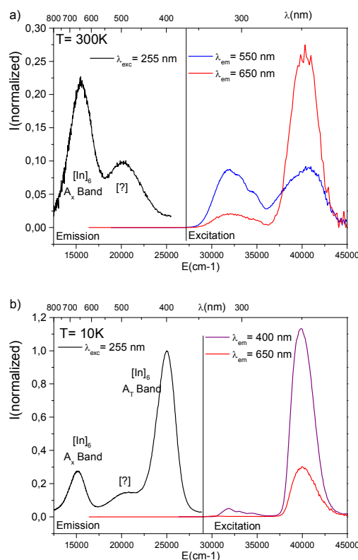
Fig. 4: Room a) and low temperature (10 K) b) luminescence spectra after a 2-hour irradiation at 315 nm showing the contribution of the indium ions reduced under the UV beam on the 4.6% cerium content \text{Rb}_2\text{KInF}_6 crushed crystal (HC).
