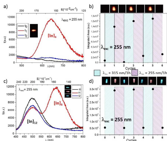
Fig. 5 Ce-doped Rb 2 KlnF 6 emission characterization. a) Ce 3+ 0.081% (LC crystal) emission spectra at different cycle steps under \lambda_{\text{exc}} = 255 nm, b) integrated area of emission curves with powder photographs of the LC crushed crystal under \lambda_{\text{exc}} = 255 nm, c) Ce 3+ 0.348% (HC crystal) emission spectra at different cycle steps under \lambda_{\text{exc}} = 255 nm, d) integrated area of emission curves with powder photographs of the HC crushed crystal under \lambda_{\text{exc}} = 255 nm.
