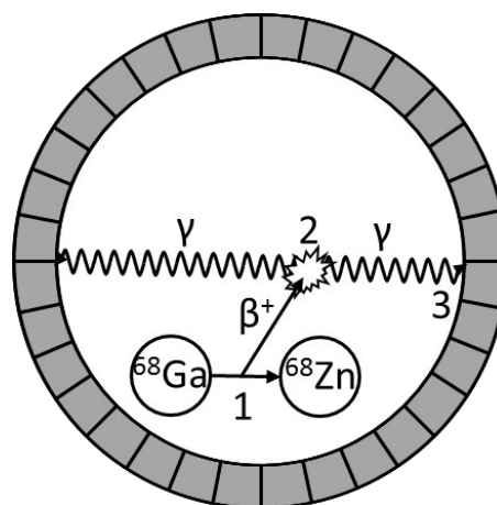
Figure 1. Schematic of a PET imaging process. 1. Positron emitted from radionuclide. 2. Positron and electron undergo annihilation interaction and emit two photons. 3. Emitted photons detected. 8
