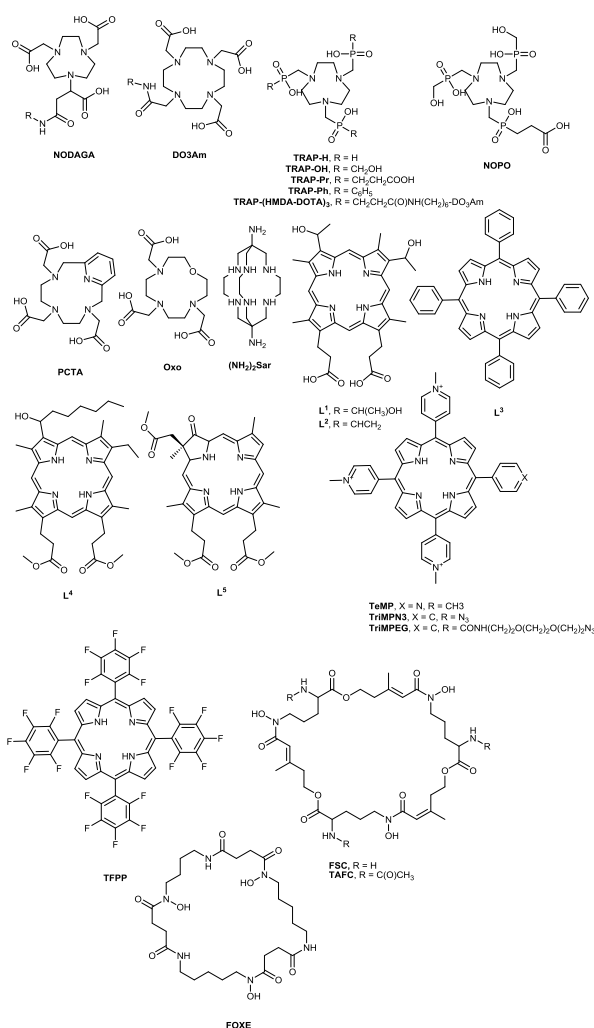
Figure 3 Structures of novel cyclic gallium chelators
