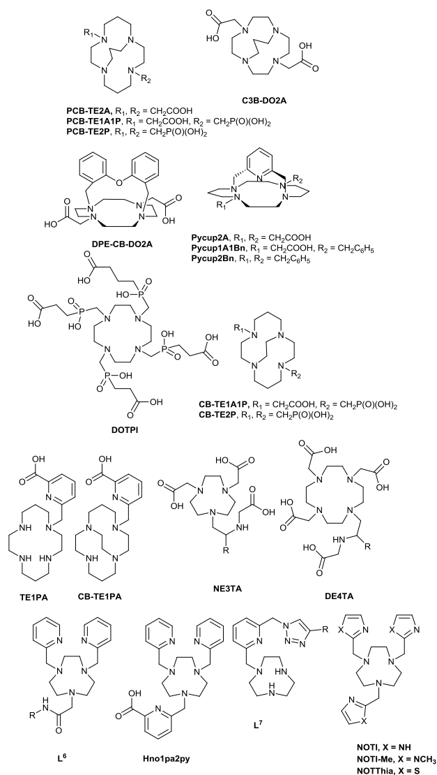
Figure 6 Structures of new copper macrocyclic chelators
