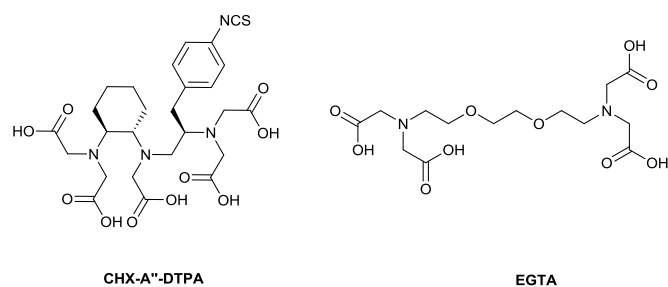
Figure 9 Acyclic scandium chelators
