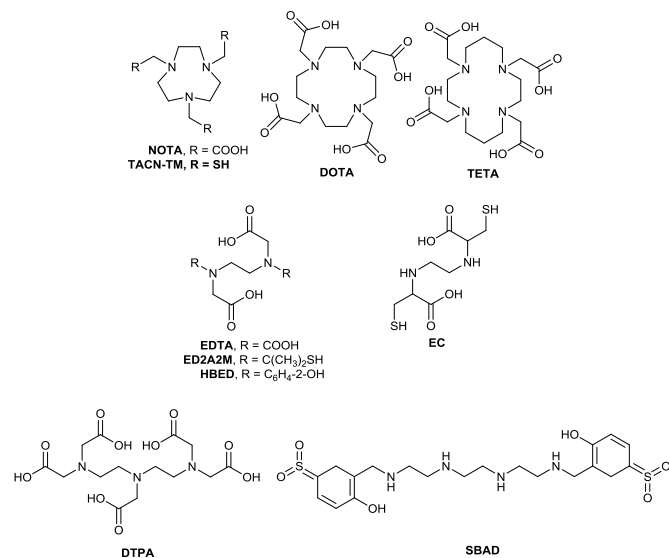
Figure 2 Structures of gallium chelators
