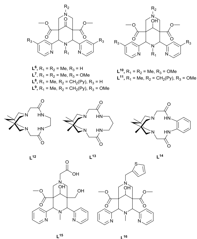
Figure 7 Bispidines applied to copper chelation
