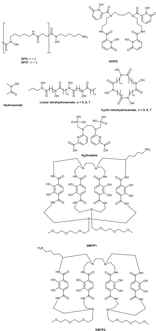
Figure 8 Structures of zirconium chelators
