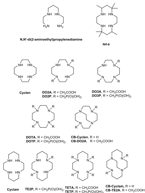
Figure 5 Structure of copper chelators
