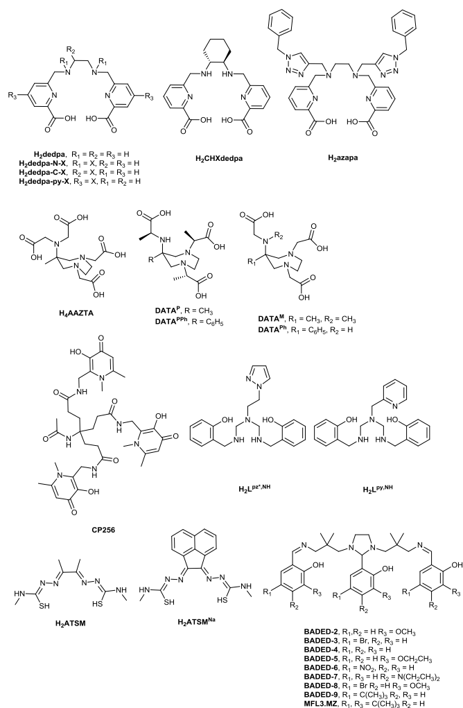
Figure 4 Structures of novel non-macrocylic gallium chelators
