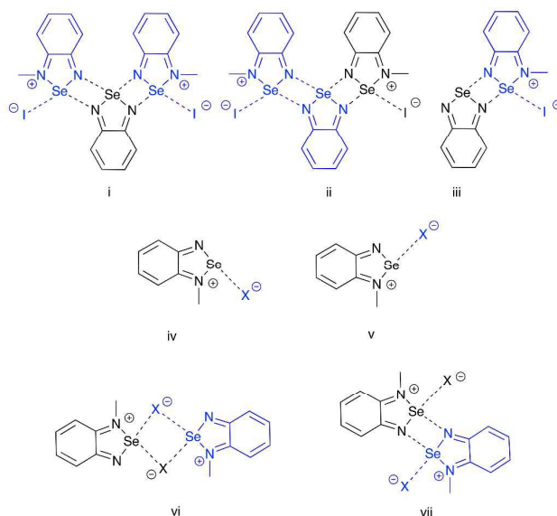
Figure 5. Partition schemes used in the DFT-D3 fragment interaction analyses. Each fragment (region) is identified with a distinct colour.
