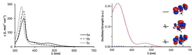
Figure 4. Experimental (left) and calculated (right) UV-vis spectra of [ 5a ][I]. Frontier orbitals shown as an inset in the calculated spectrum.
