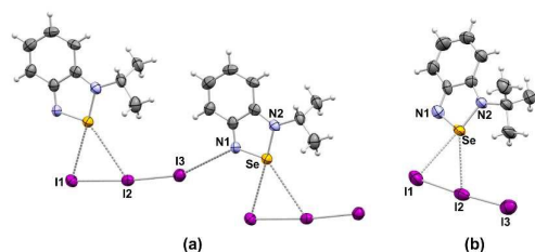
Figure 2. Crystal structures of (a) [ 5b ][I 3 ] and (b) [ 5c ][I 3 ]. Selected bond distances (a) Se ⋯ I 1 : 3.249(1) Å, Se ⋯ I 2 : 3.626(5) Å; (b) Se ⋯ I 1 : 3.309(1) Å, Se ⋯ I 2 : 3.727(1) Å.
