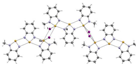
Figure 1. Arrangements of molecules and ions in the crystal 4 [ 5a ] 2 [I] 2 . Selected distances: Se 1 -N 1 : 2.573(4) Å and 2.5937 Å.
