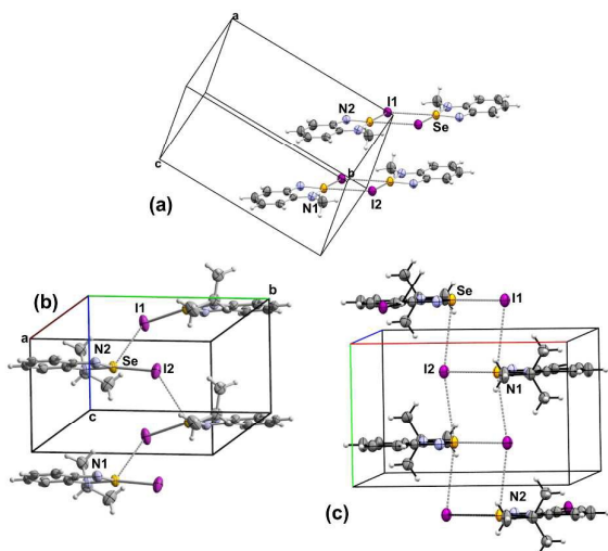
Figure 3. Packing arrangement in the crystal structures of the iodide salts of (a) 5a (b) 5b and (c) 5c .
