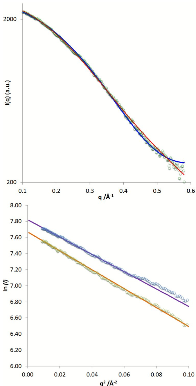
Fig. 2 SAXS data for a 3 mM acetone solution of \text{TBA}_5[\text{Mo}_6\text{O}_{18}\text{NC}(\text{OCH}_2)_3\text{MnMo}_6\text{O}_{18}(\text{OCH}_2)_3\text{CNH}_2] (top). Fits : Cylindrical model (red), spherical model (blue). Guinier plots, whose low q linear fits yield the radius of gyration, for a fresh sample (purple), and a sample aged for 7 days (orange) (bottom).
