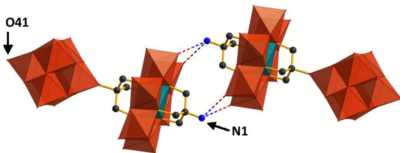
Fig. 1 Graphical representation of two molecules of (1) with solid state hydrogen bonding interactions displayed as broken bonds. Mo, orange; Mn, teal; C, black; O, red; N, blue
